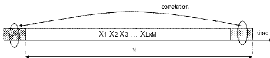
a) STANDARD SC-FDMA: correlation of CP samples
