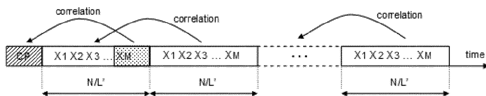
b) PROPOSAL: correlation of CP and the repeated blocks
