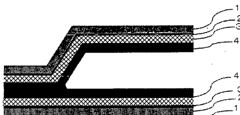
(A-2)
