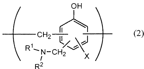
[Chemical Formula 3]
