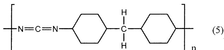
[Chemical Formula 5]
