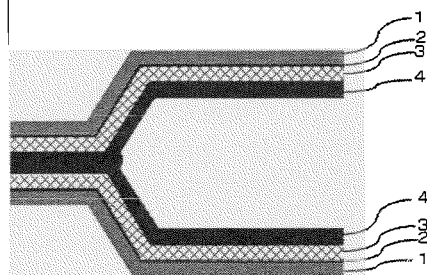
(A-1)
