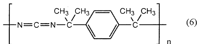
[Chemical Formula 6]
