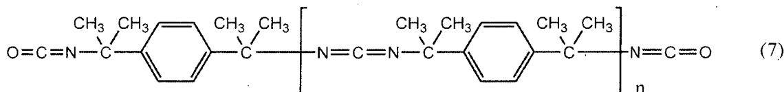
[Chemical Formula 7]
