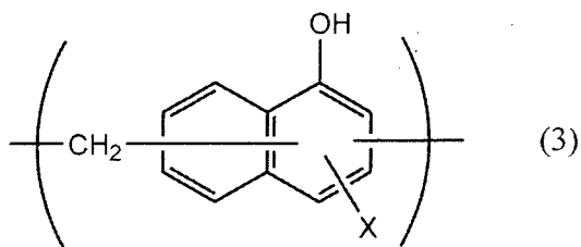
[Chemical Formula 4]
