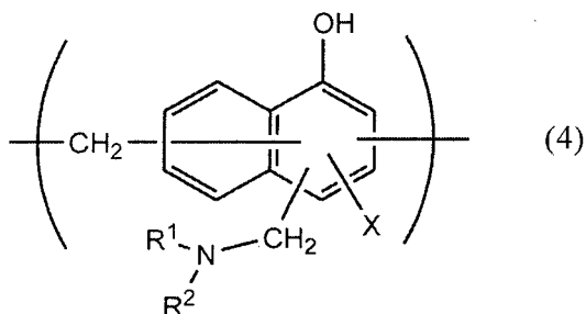
[Chemical Formula 4]
