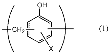
[Chemical Formula 2]
