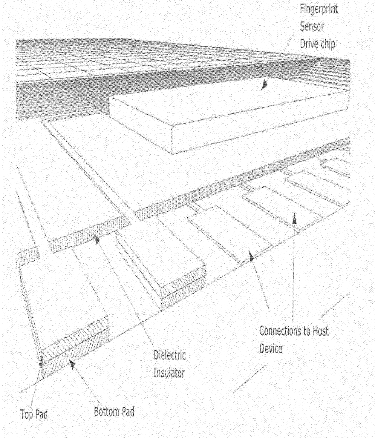
Fig 32: Detail Interconnect of Fingerprint Sensor Sharing Substrate with Touchscreen
