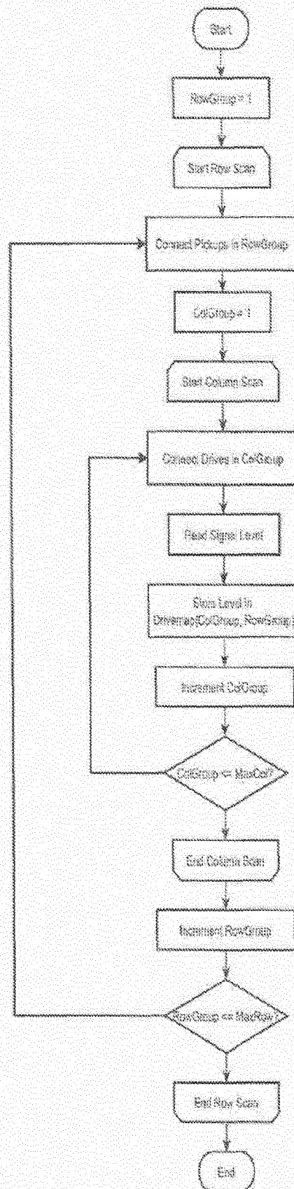
Fig 43: Dual Grid Coarse Position Determination- Scan Process
