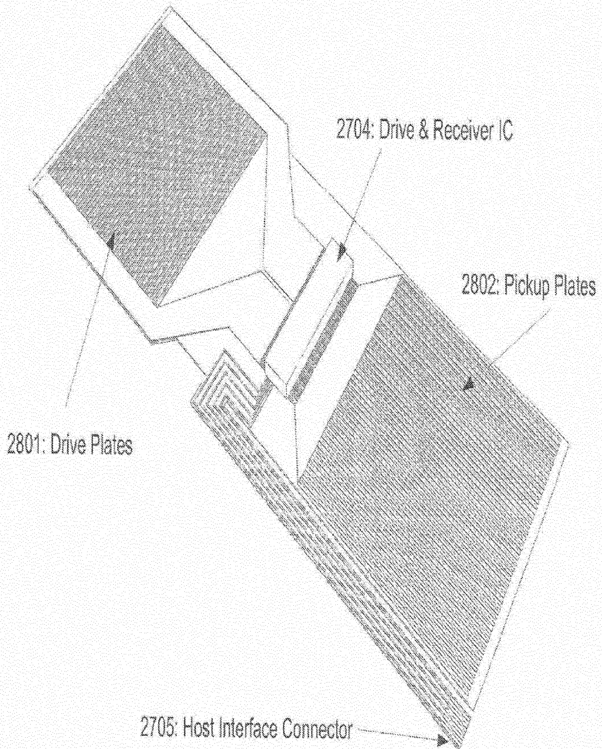
Fig 28: Unfolded Sensor
