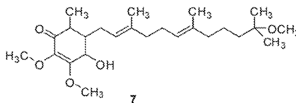
Compound 7: 4-hydroxy-2,3-dimethoxy-5-(11-methoxy-3,7,11-trimethyldodeca-2,6-dienyl)-6-methylcyclohex-2-enone
