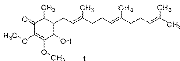
Compound 1 : 4-hydroxy-2,3-dimethoxy-6-methyl-5-(3,7,11-trimethyldodeca-2,6,10-trienyl)cyclohex-2-enone
