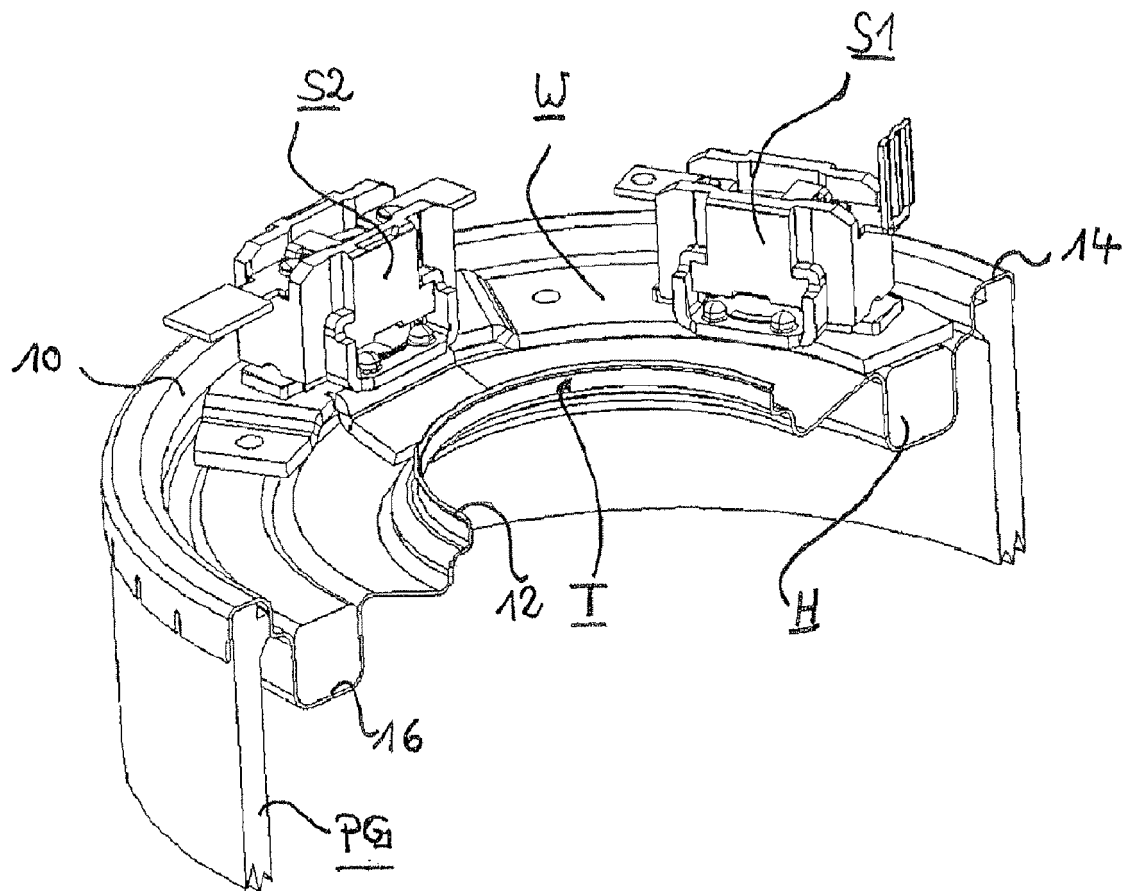
FIG. 2 (PRIOR ART)
