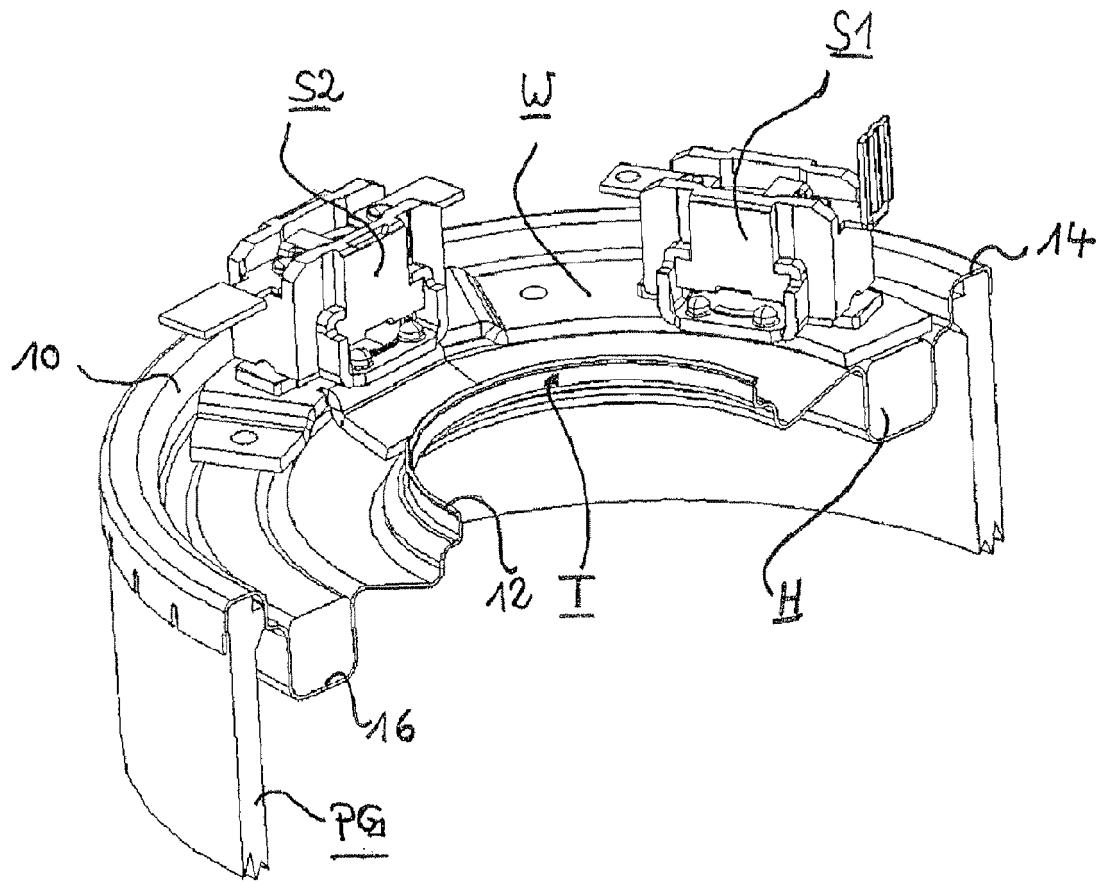
FIG. 2 (PRIOR ART)
