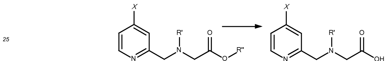
Scheme 18
