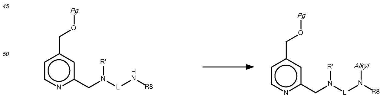
Scheme 25
