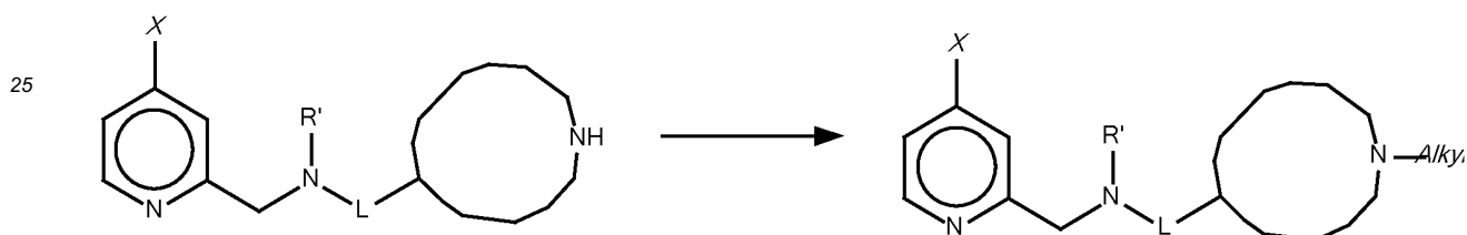
Scheme 21
