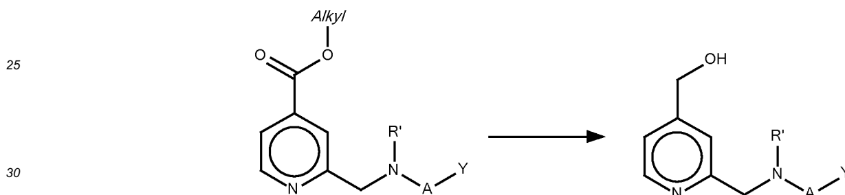
Scheme 30
