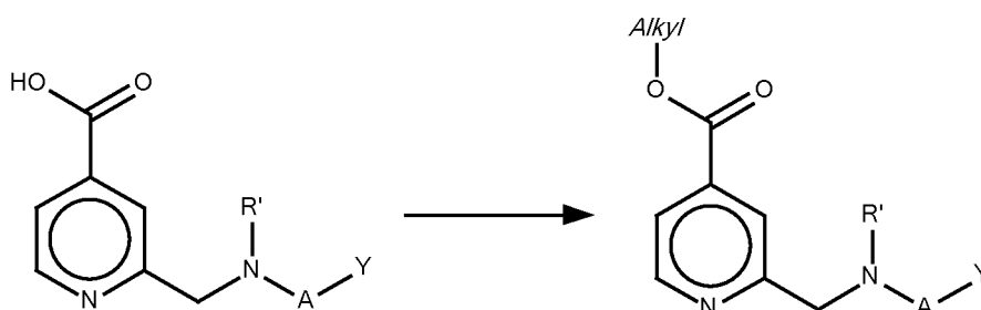
Scheme 33
