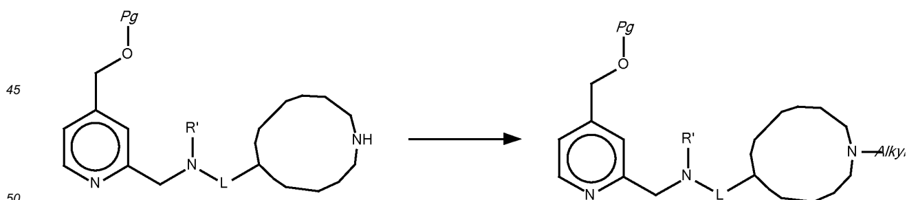
Scheme 22
