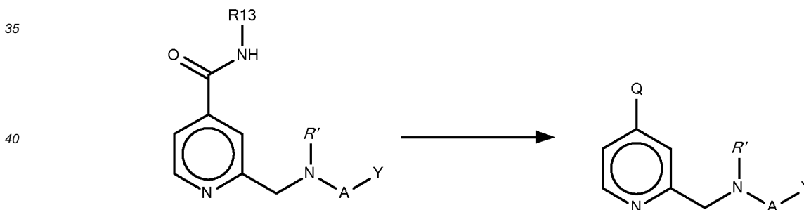
Scheme 5 - Reduction of amide
