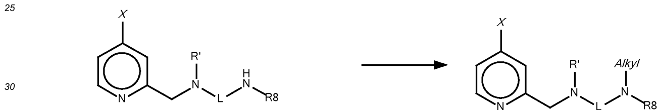
Scheme 24
