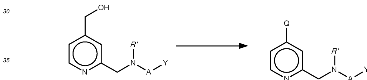
Scheme 7
