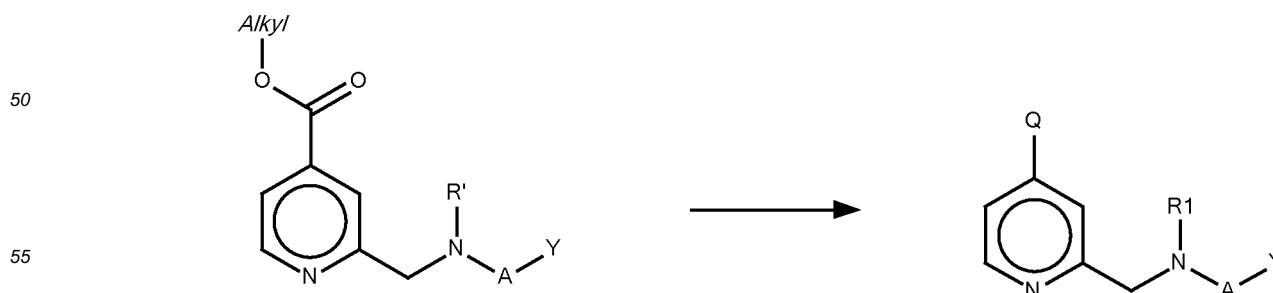
Scheme 8
