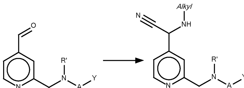
Scheme 35
