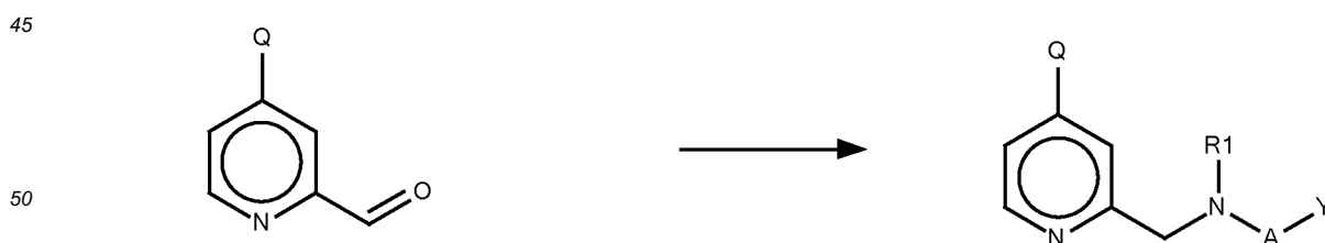
Scheme 3 - Reductive amination
