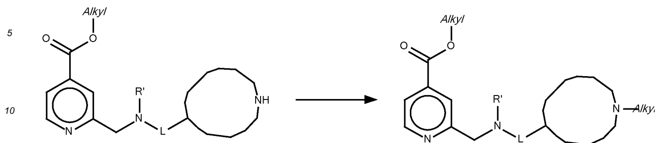
Scheme 20
