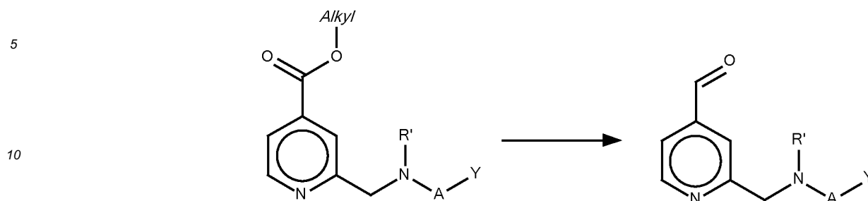
Scheme 29
