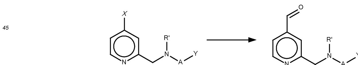
Scheme 31
