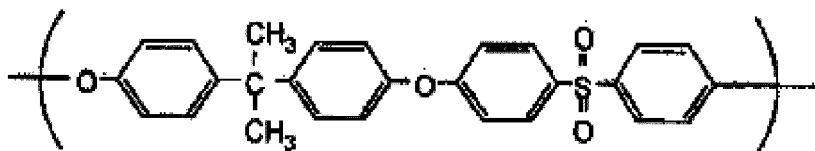
[Chemical formula 1]
