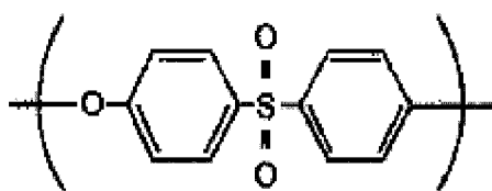
[Chemical formula 2]
