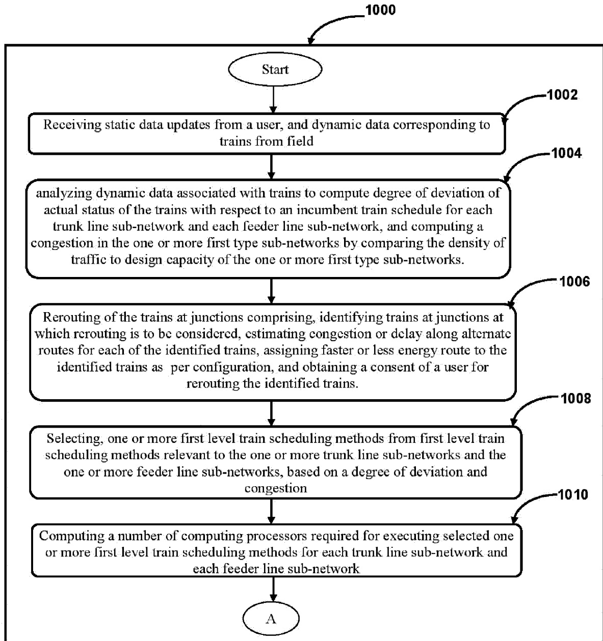
FIGURE 10
