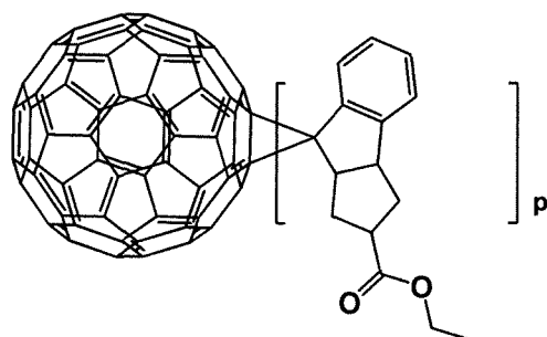
[Formula 1- 1- 41]
