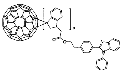
[Chemical Formula 1-1-19]
