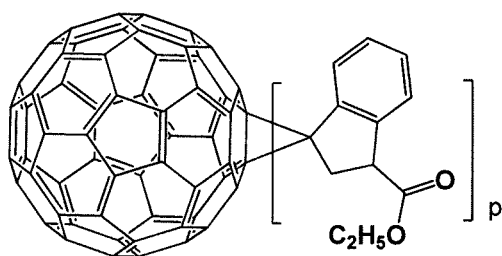
[Formula 1- 1- 1]
