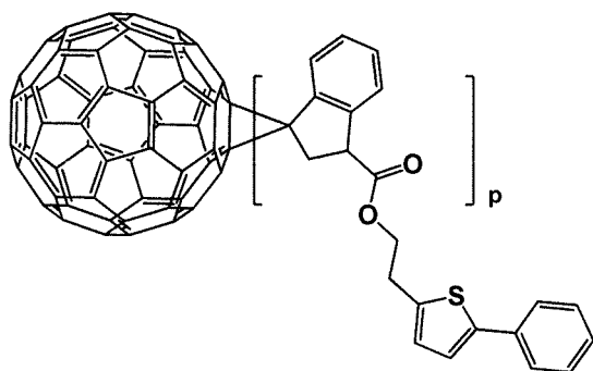
[Formula 1- 1- 39]
