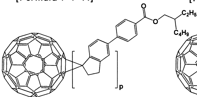
[Formula 1- 1- 11]
