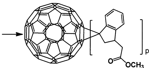
[Chemical Formula 1-1-2]
