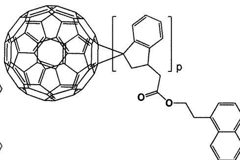
[Formula 1- 1- 18]
