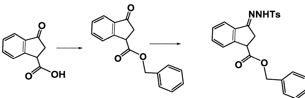
[Chemical Formula 1-1-5]
