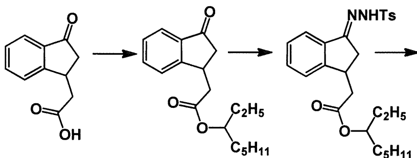
[Chemical Formula 1-1-13]
