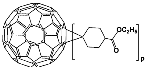
[Formula 1- 1- 11]
