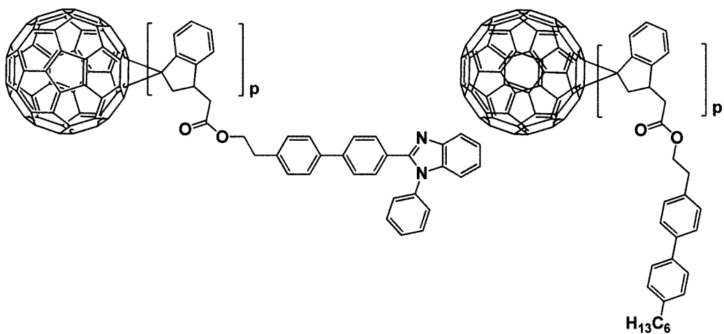
[Formula 1- 1- 28]
