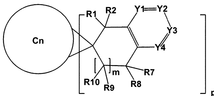
[Chemical Formula 3]
