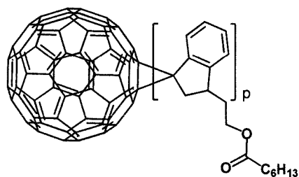
[Formula 1-1-48]
