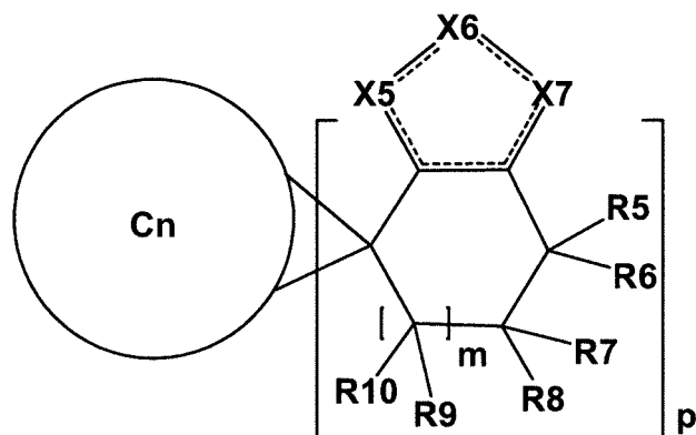
[Chemical Formula 5]
