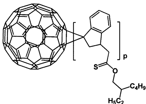
[Formula 1- 1- 53]
