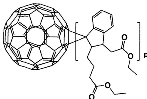
[Formula 1- 1- 42]
