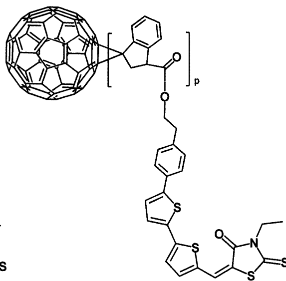
[Formula 1- 1- 46]
