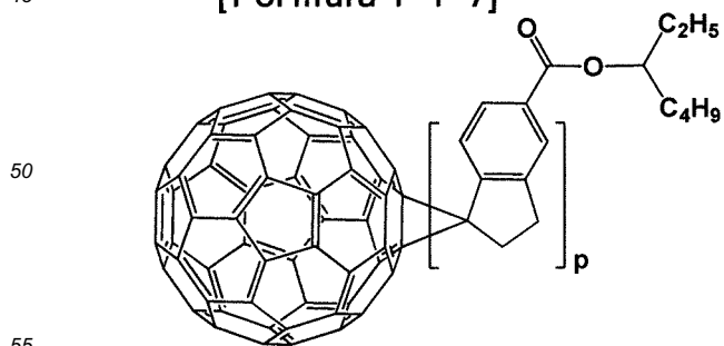
[Formula 1-1-7]
