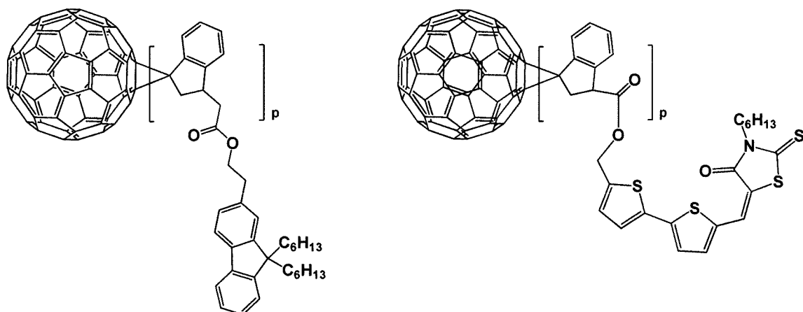
[Formula 1- 1- 30]
