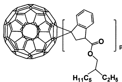
[Formula 1- 1- 34]
