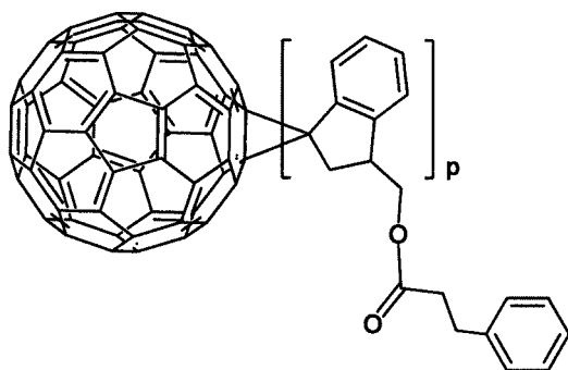
[Formula 1- 1- 47]
