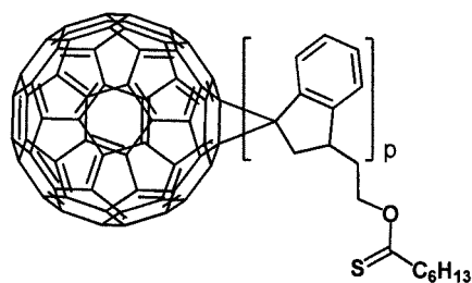
[Formula 1- 1- 52]
