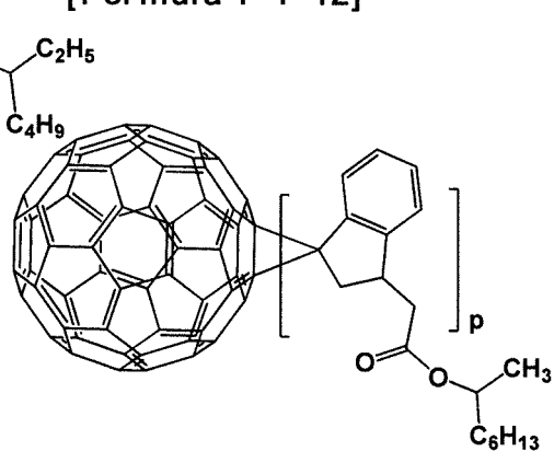
[Formula 1-1-12]
