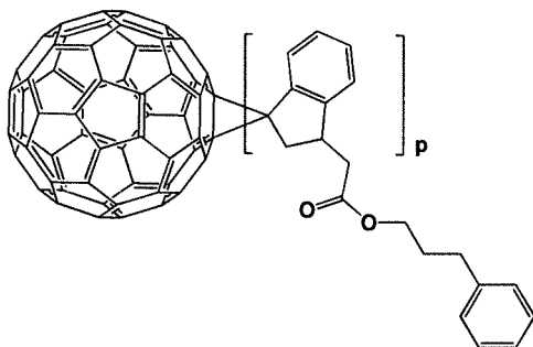
[Formula 1- 1- 15]
