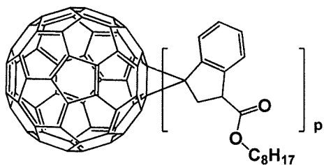
[Formula 1- 1- 35]
