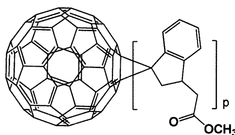
[Formula 1- 1- 2]
