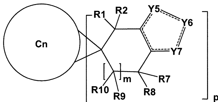
[Chemical Formula 5]
