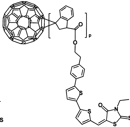
[Formula 1-1-46]
