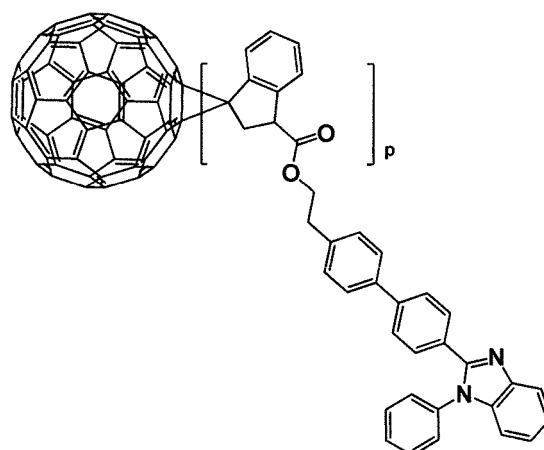
[Formula 1- 1- 40]
