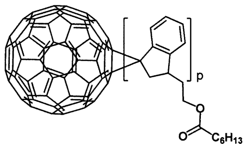
[Formula 1- 1- 48]
