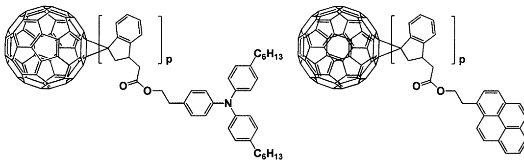
[Formula 1- 1- 28]
