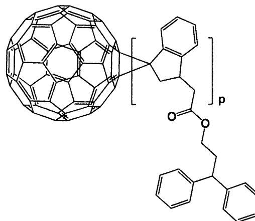
[Formula 1- 1- 22]
