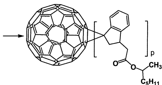
[Chemical Formula 1-1-6]
