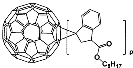
[Formula 1- 1- 35]
