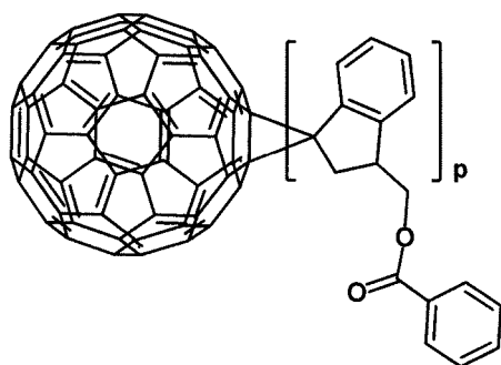
[Formula 1- 1- 49]
