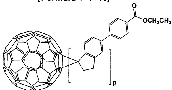
[Formula 1-1-10]
