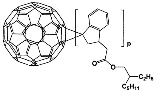
[Formula 1- 1- 14]
