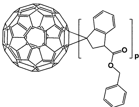
[Formula 1-1-7]
