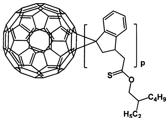
[Formula 1- 1- 53]
