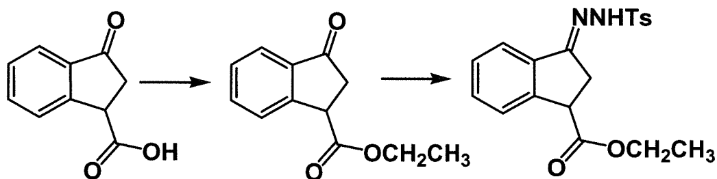
[Chemical Formula 1-1-1]
