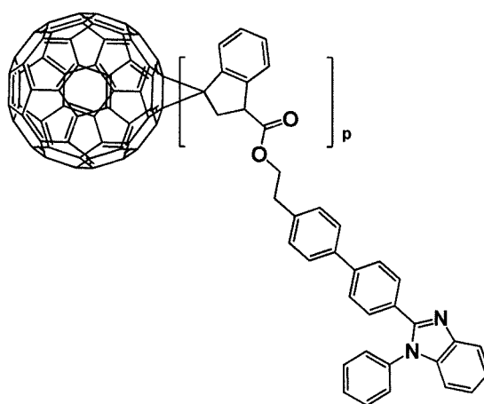
[Formula 1- 1- 38]
