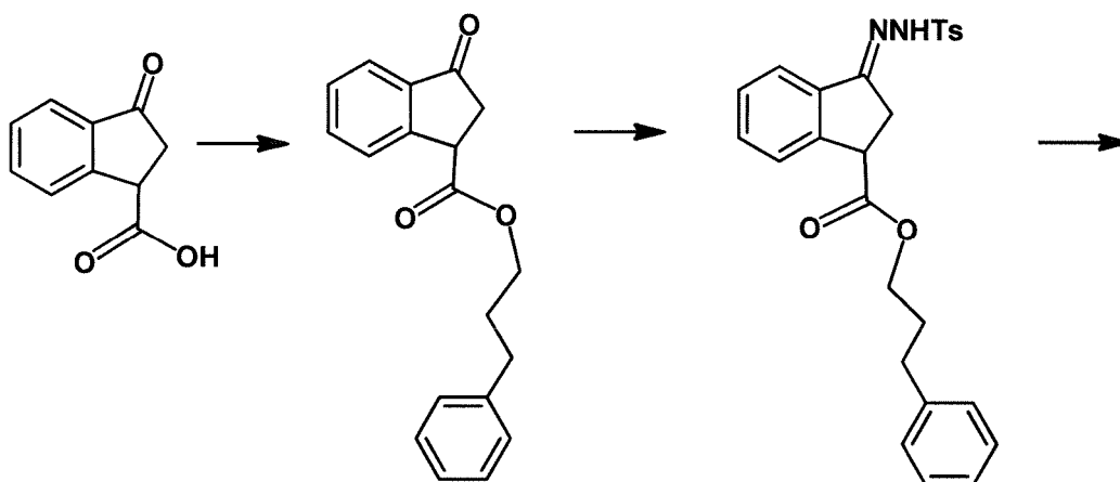
[Chemical Formula 1-1-44]
