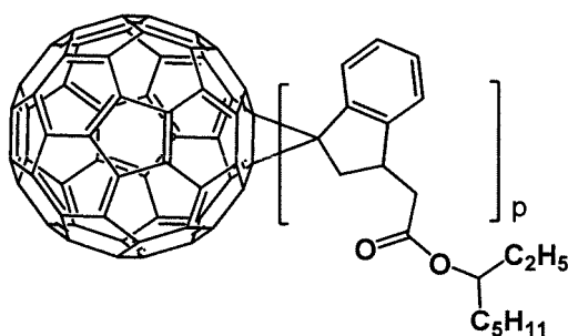
[Chemical Formula 1-1-13]
