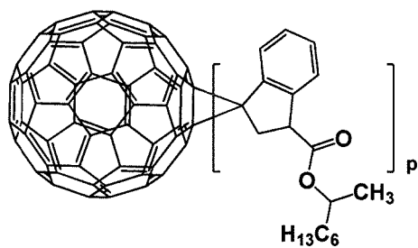
[Formula 1- 1- 38]
