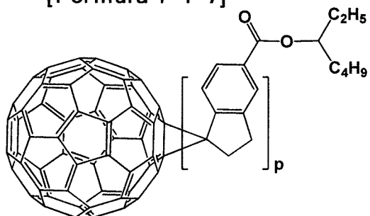
[Formula 1-1-7]
