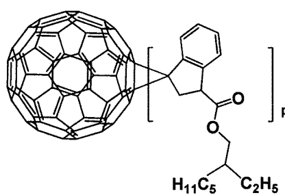
[Formula 1- 1- 34]
