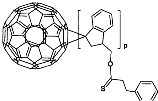
[Formula 1- 1- 51]
