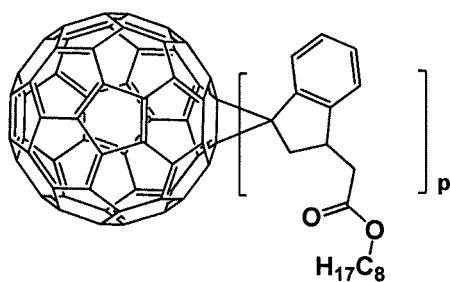
[Formula 1- 1- 31]
