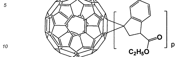
[Formula 1-1-1]
