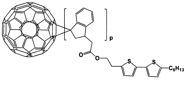
[Formula 1- 1- 16]
