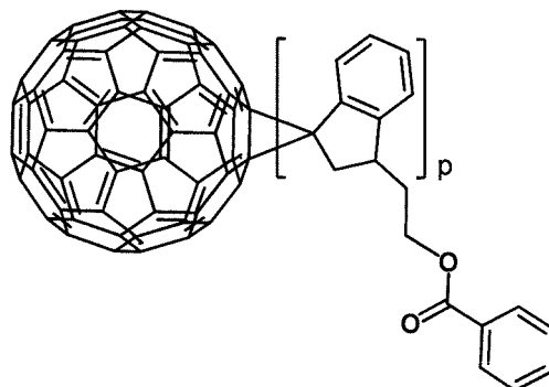
[Formula 1- 1- 50]
