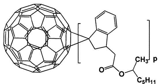
[Formula 1-1-6]
