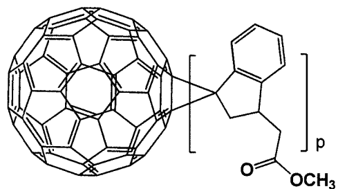
[Formula 1-1-2]
