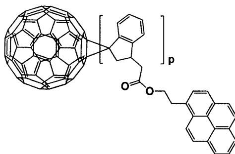
[Formula 1- 1- 26]
