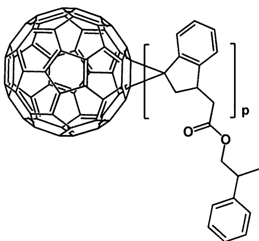
[Formula 1- 1- 43]
