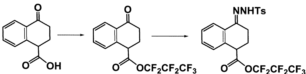
[Chemical Formula 1-1-8]
