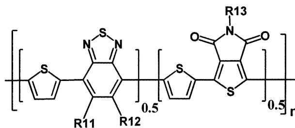
[Chemical Formula 2-1]
