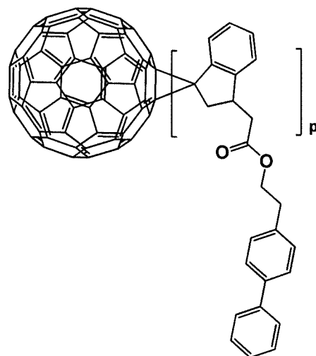
[Formula 1- 1- 32]
