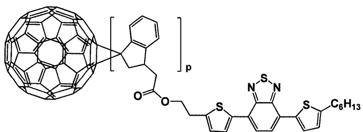
[Formula 1- 1- 24]
