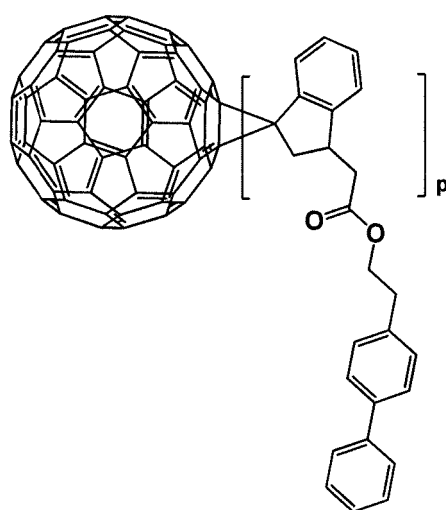
[Formula 1- 1- 32]
