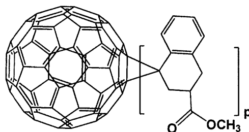
[Formula 1-1-6]
