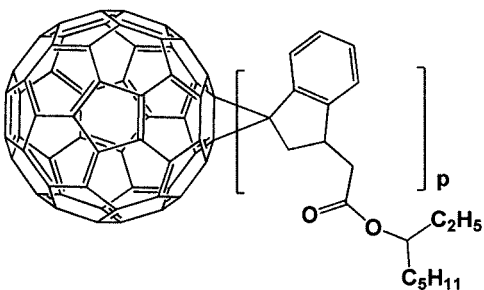
[Formula 1- 1- 13]
