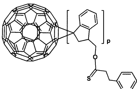
[Formula 1- 1- 51]
