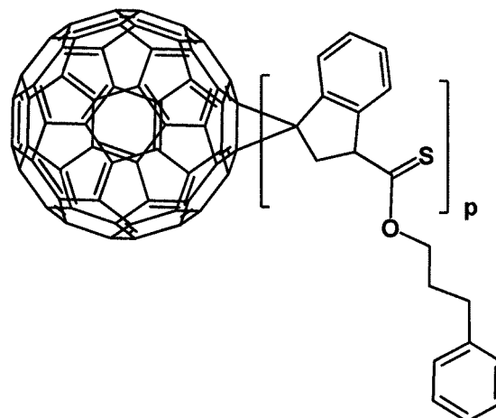
[Formula 1- 1- 54]
