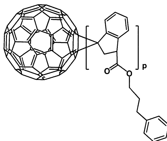
[Formula 1- 1- 44]
