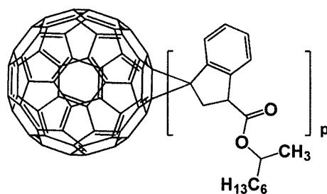
[Formula 1- 1- 36]
