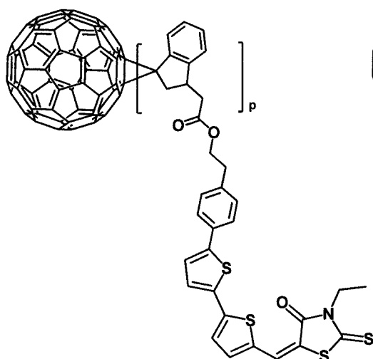
[Formula 1-1-45]
