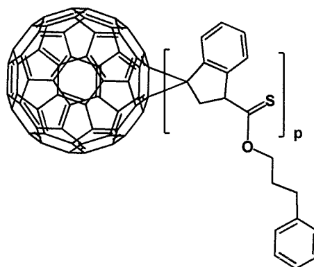
[Formula 1- 1- 54]
