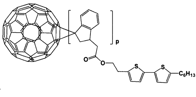
[Formula 1-1-16]
