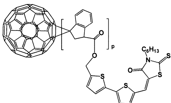
[Formula 1- 1- 30]
