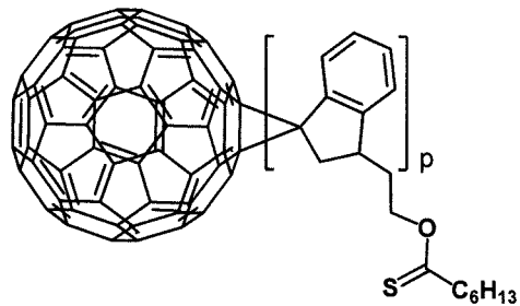
[Formula 1- 1- 52]
