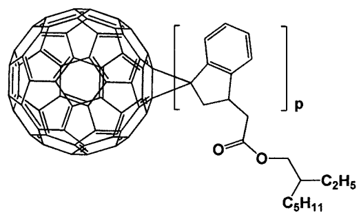
[Formula 1-1-14]
