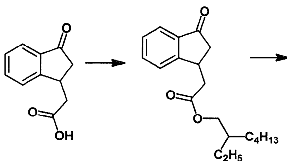
[Chemical Formula 1-1-21]
