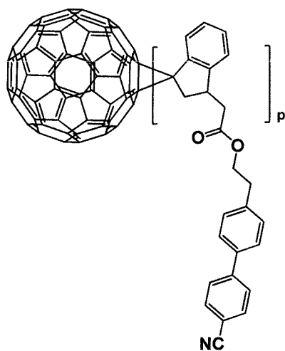
[Formula 1- 1- 35]
