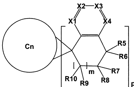
[Chemical Formula 3]
