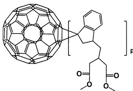
[Formula 1- 1- 40]
