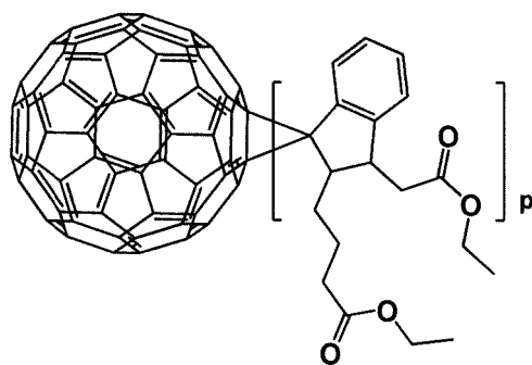
[Formula 1- 1- 42]
