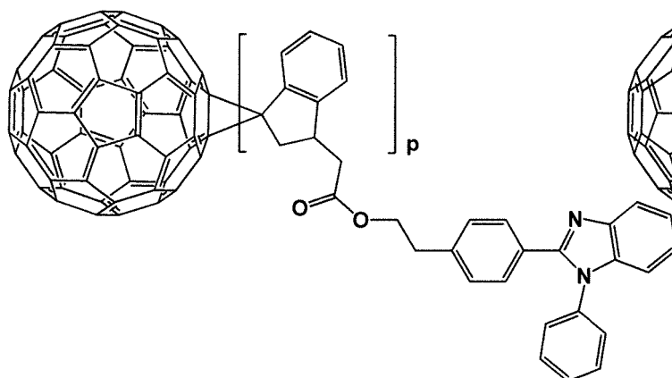
[Formula 1- 1- 19]
