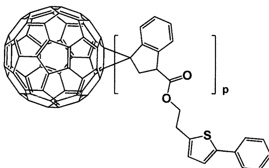
[Formula 1- 1- 41]
