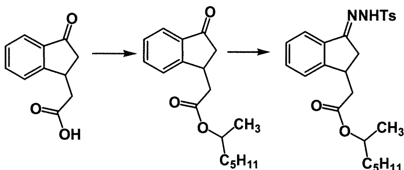
[Chemical Formula 1-1-6]
