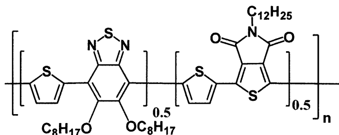
[Chemical Formula 2-1-1]
