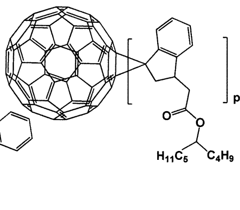
[Formula 1-1-20]
