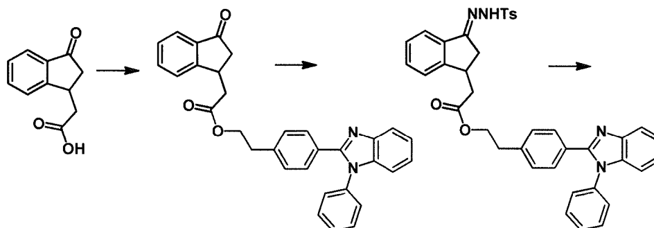
[Chemical Formula 1-1-19]
