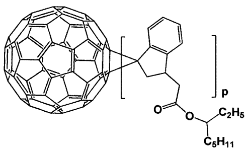
[Formula 1-1-13]
