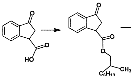
[Chemical Formula 1-1-36]
