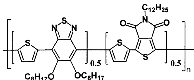
[Chemical Formula 2-1-1]
