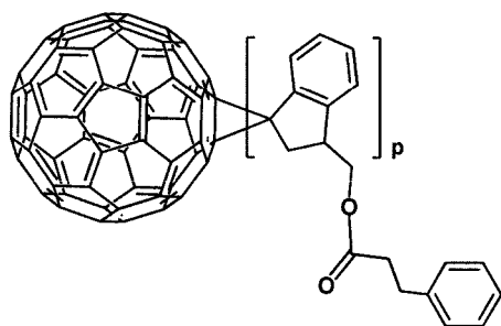
[Formula 1-1-47]
