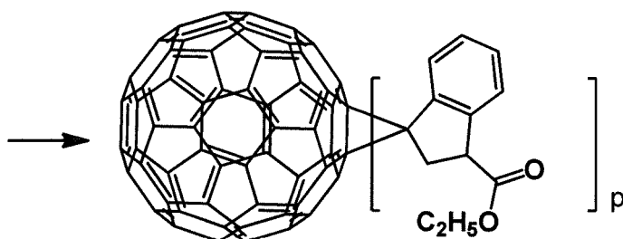
[Chemical Formula 1-1-1]
