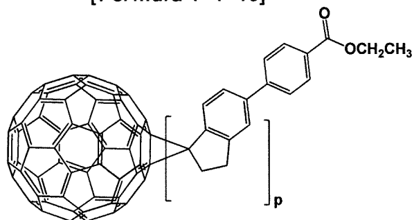
[Formula 1- 1- 10]
