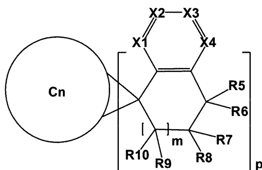
[Chemical Formula 2]
