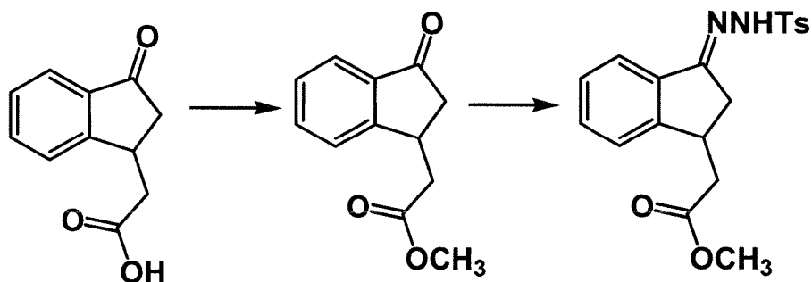
[Chemical Formula 1-1-2]
