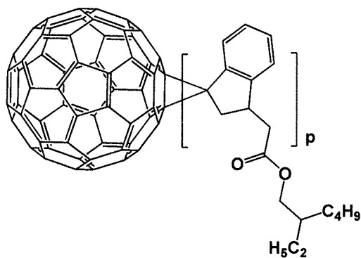
[Formula 1- 1- 21]
