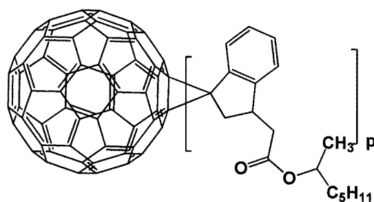
[Formula 1-1-6]
