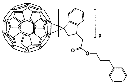
[Formula 1-1-15]
