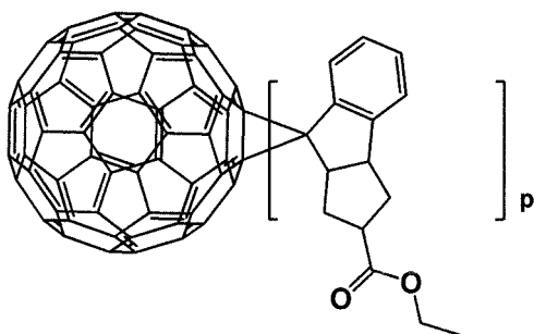
[Formula 1- 1- 41]
