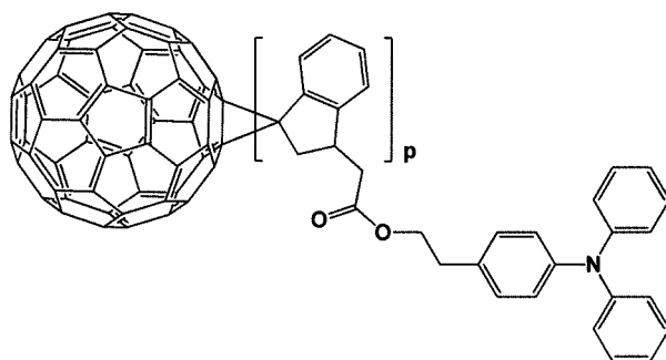
[Formula 1- 1- 17]
