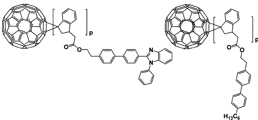
[Formula 1- 1- 30]
