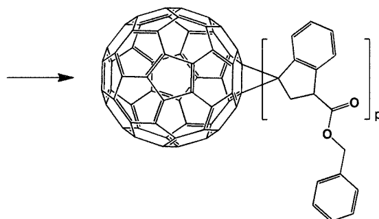
[Chemical Formula 1-1-5]
