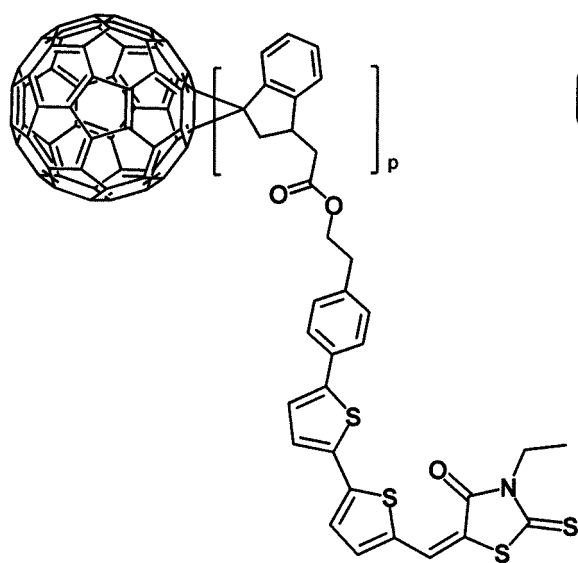
[Formula 1- 1- 45]
