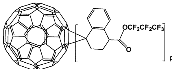
[Formula 1-1-10]
