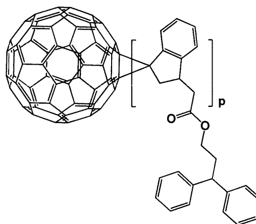
[Formula 1-1-22]
