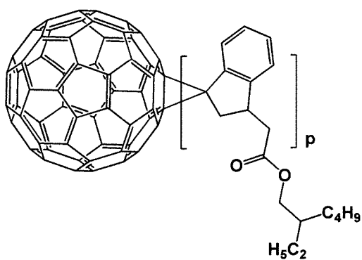
[Formula 1-1-21]
