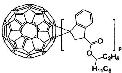
[Formula 1- 1- 37]
