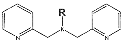
Neutral Donor
