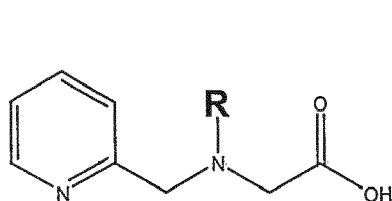
Charge = -1
