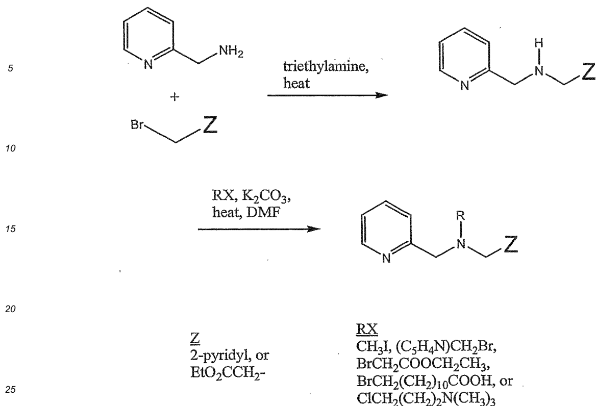
Scheme 1. Synthesis of various DPMA derivatives.
