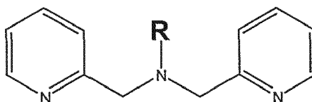
R = biologically relevant molecule
