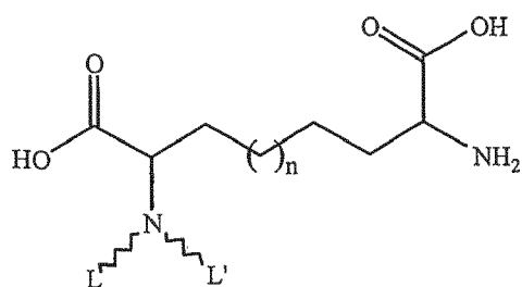
Scheme 3. The amino acid-based bifunctional chelates of this study.
