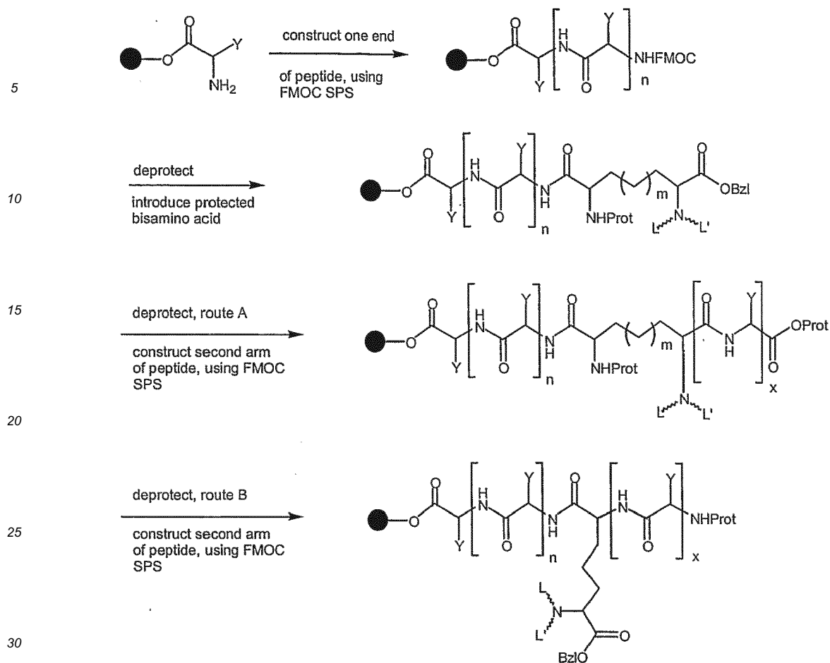
Scheme 4. Integration of the bifunctional chelate into the peptide sequence.
