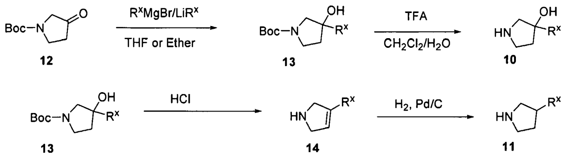
Scheme 4
