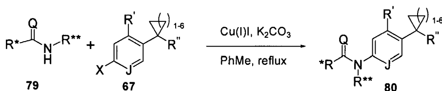
Scheme 21
