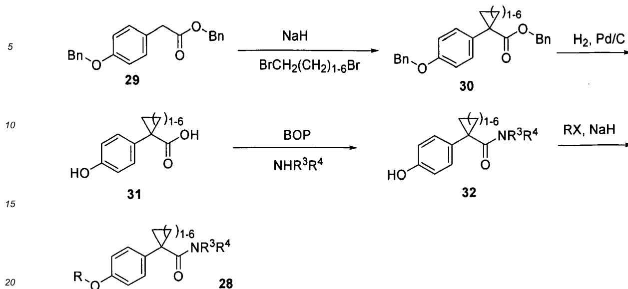
Scheme 10
