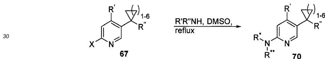
Scheme 18
