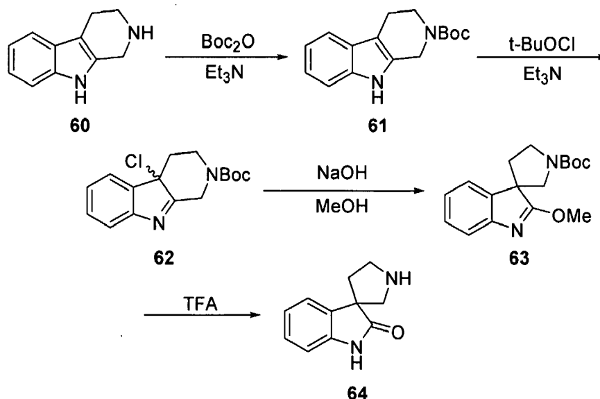
Scheme 16
