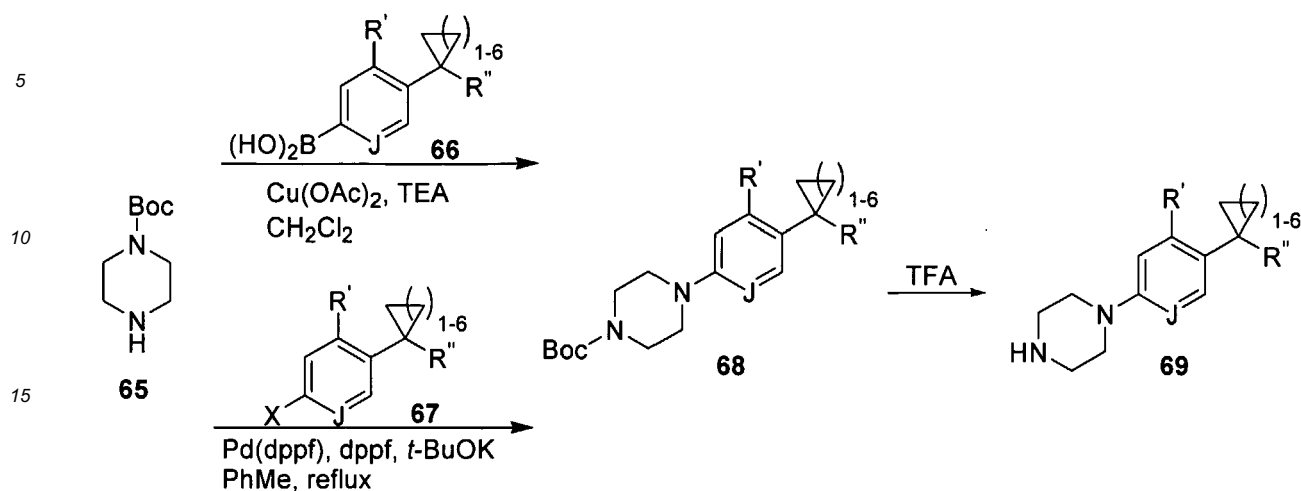
Scheme 17
