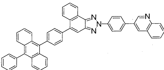
(Compound 72)
