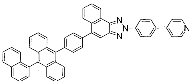
(Compound 48)
