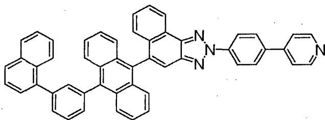
(Compound 17)
