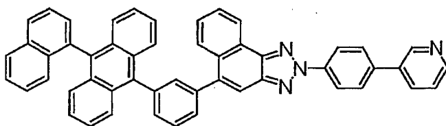
(Compound 54)
