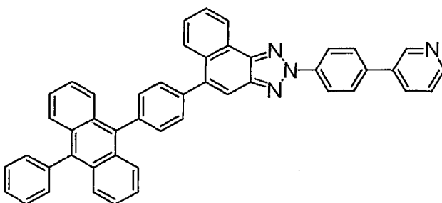
(Compound 47)
