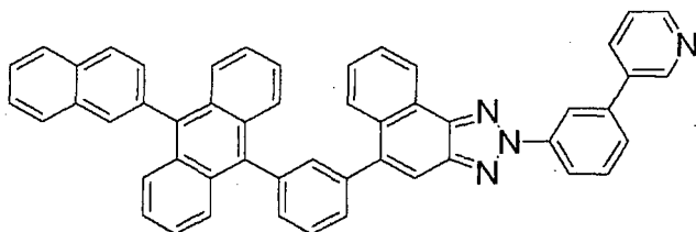
(Compound 55)
