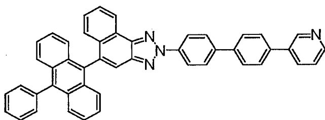
(Compound 69)
