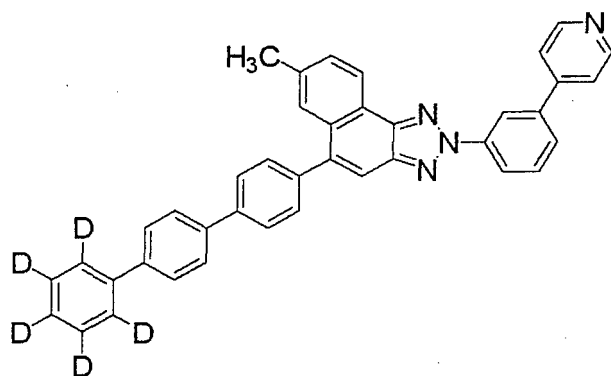
(Compound 33)
