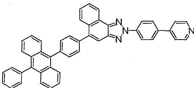
(Compound 46)
