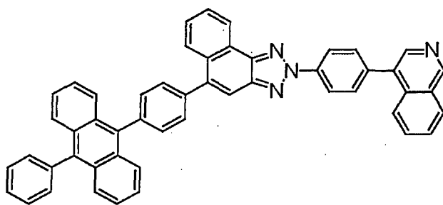
(Compound 73)
