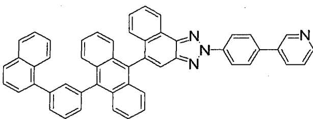
(Compound 18)
