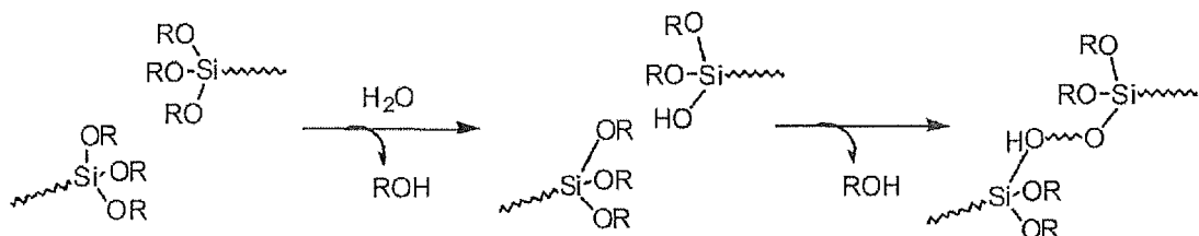
[Chemical 4]
