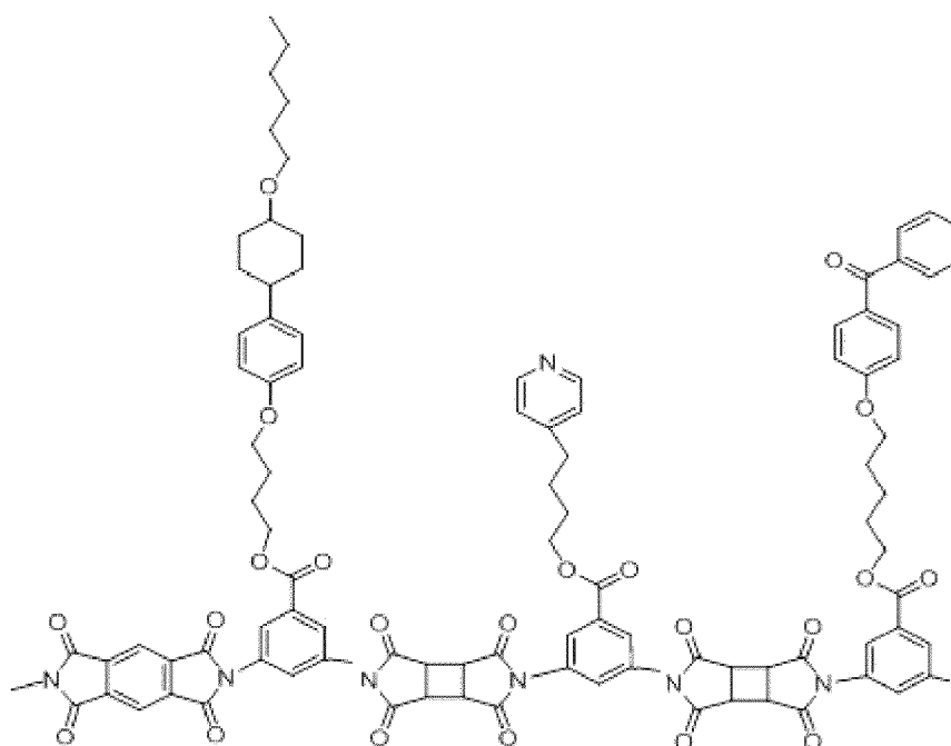
Chemical formula 2
