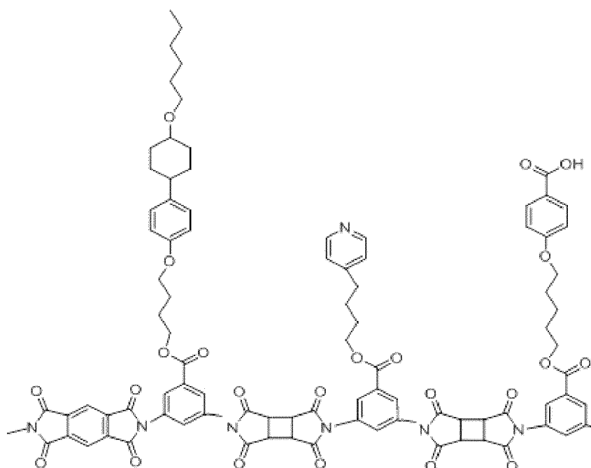
Chemical formula 2
