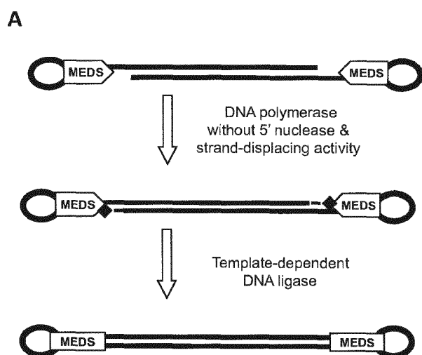
FIG. 18 Tagged circular DNA fragments are resistant to T5 Exonuclease
