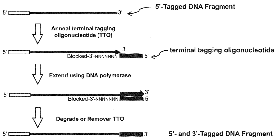
FIG. 20 Use of a Terminal Tagging Oligonucleotide to Generate 5'- and 3'-Tagged DNA Fragments
