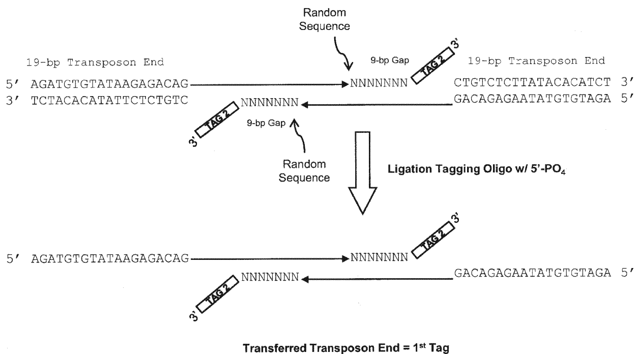
FIG. 21 Use of a DNA Ligase & a Ligation Tagging Oligo for Generating 5'- and 3'-Tagged DNA Fragments
