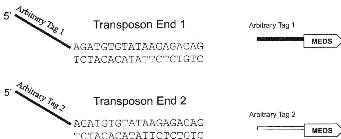
FIG. 4 Transposon Ends with Transposon End Oligonucleotides with Different Tags in Their 5'-Portions
