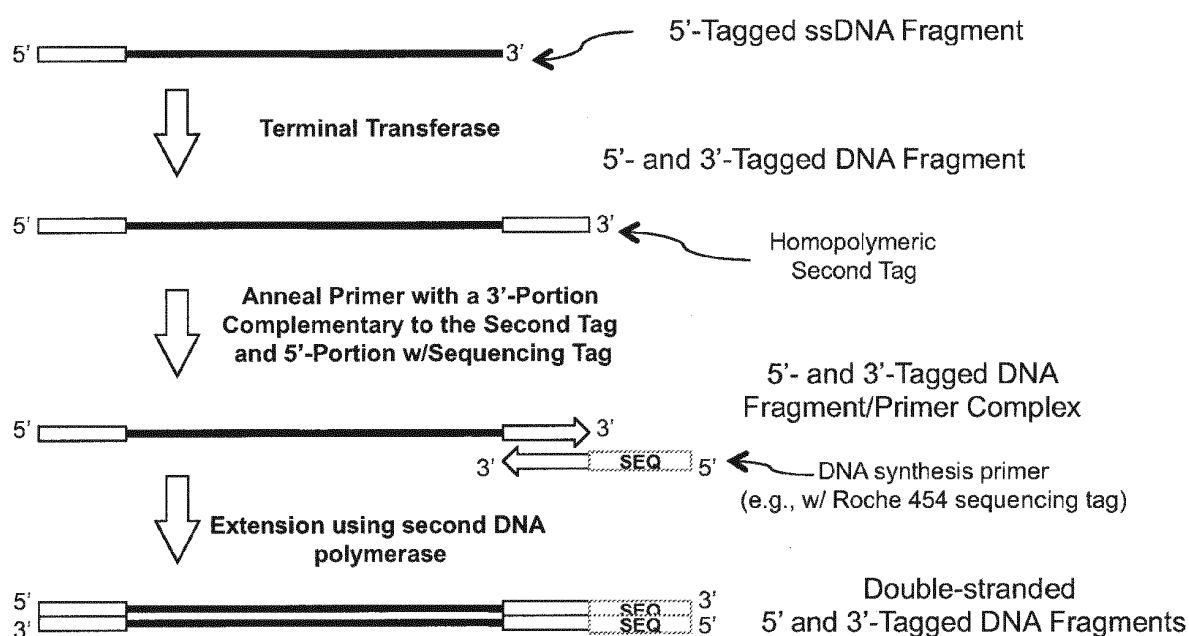
FIG. 19 Joining a Sequencing Tag to 5'- and 3'-Tagged DNA Fragments that Have a Second Tag Using a Second DNA Polymerase
