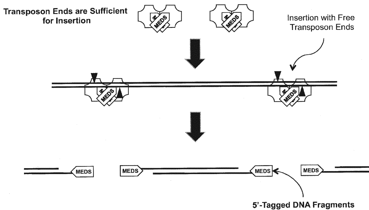
FIG. 2 Fragmenting by In Vitro Transposition
