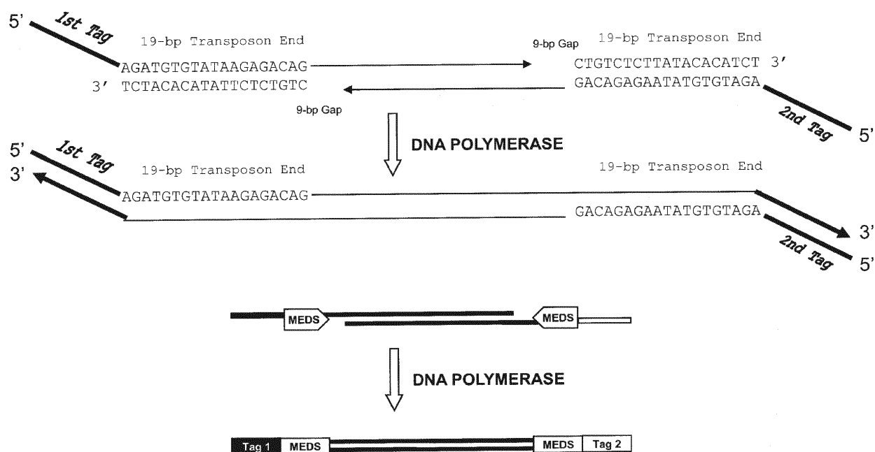
FIG. 8 Use of a DNA Polymerase for 3'-Tagging of 5'-Tagged DNA Fragments (with EZ-Tn5™ Transferred Transposon Ends Having Two Different 5'-Portions, Each Inserted into a Different Strand of Target DNA)
