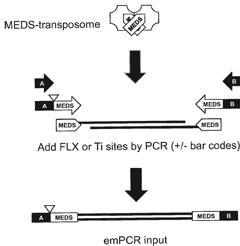
FIG. 10 Preparation of Bar Coded Roche/454 FLX-Compatible Sequencing Libraries
