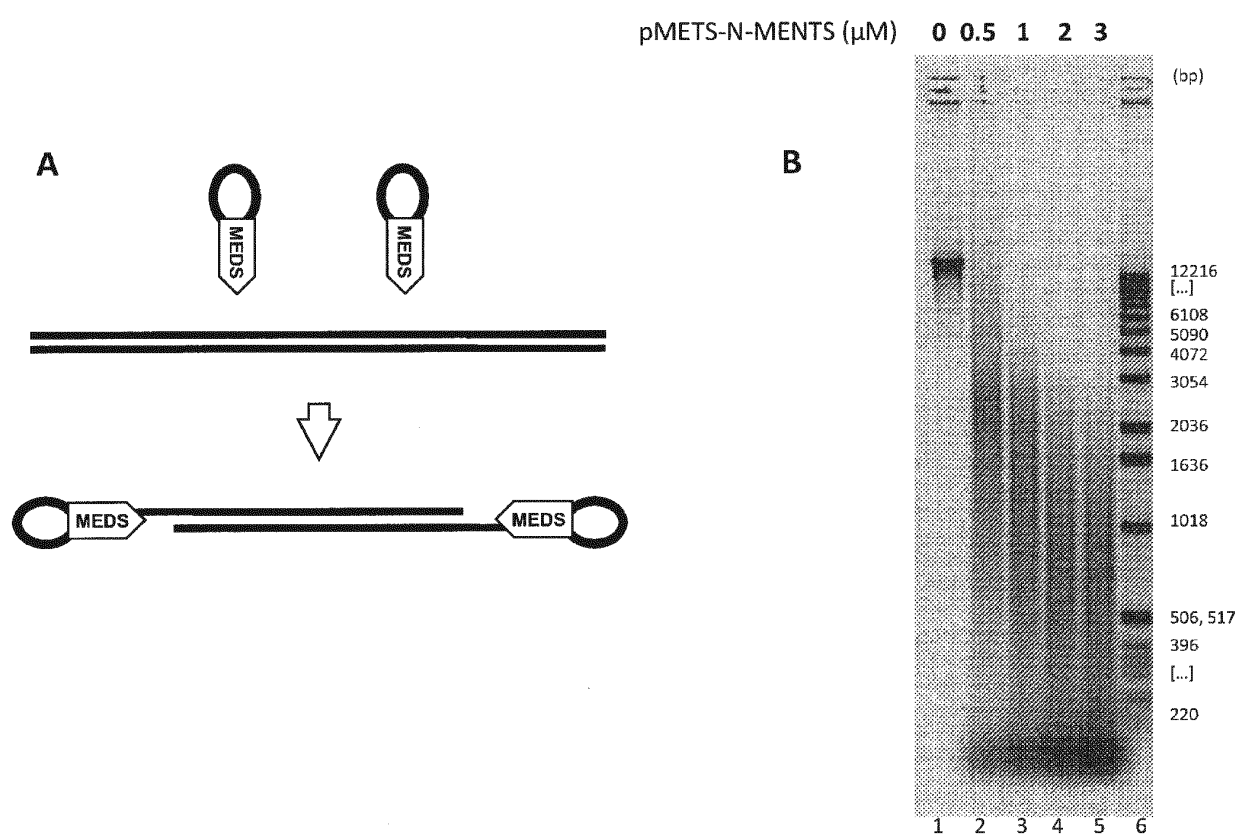
FIG. 17 5'-tagging & fragmentation of dsDNA by a transposase and a hairpin transposon end composition
