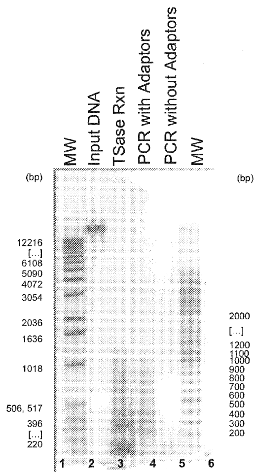
FIG. 14 Preparation of Bar Coded Illumina GAII-Compatible Sequencing Library
