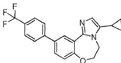
2-(10-(4-(trifluoromethyl)phenyl)-5,6-dihydrobenzo[f]imidazo[1,2-d][1,4]oxazepin-3-yl)propan-2-ol (Compound 1-10)
