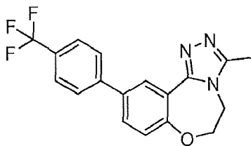
11-(4-(trifluoromethyl)phenyl)-3,4,6,7-tetrahydro-2H-benzo[f]pyrimido[1,2-d][1,4]oxazepine (Compound 1-8)
