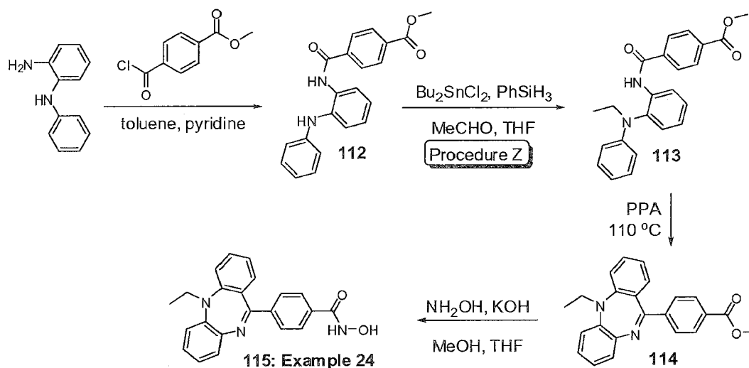
Scheme 23
