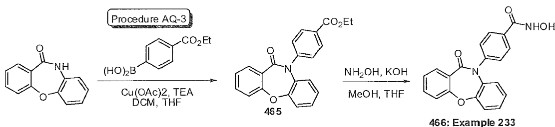
Scheme 83
