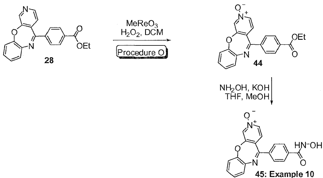
Scheme 10
