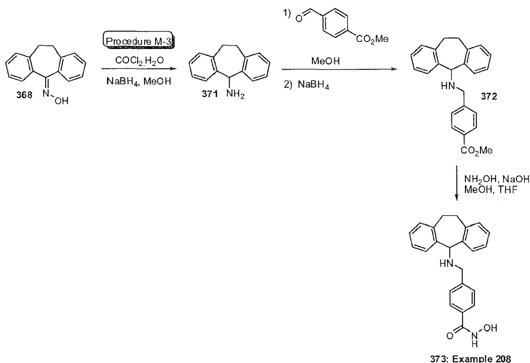
Scheme 58
