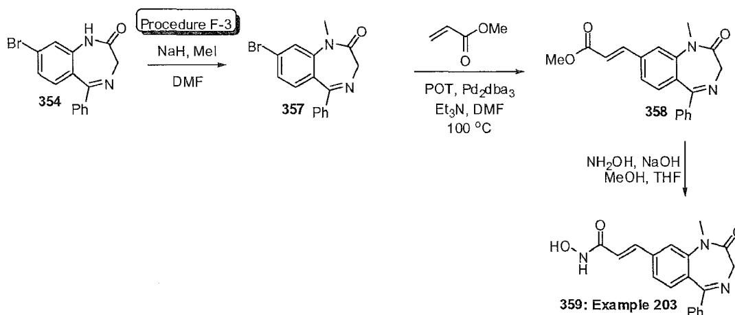
Scheme 53
