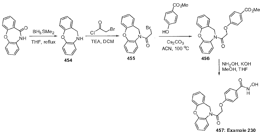
Scheme 80
