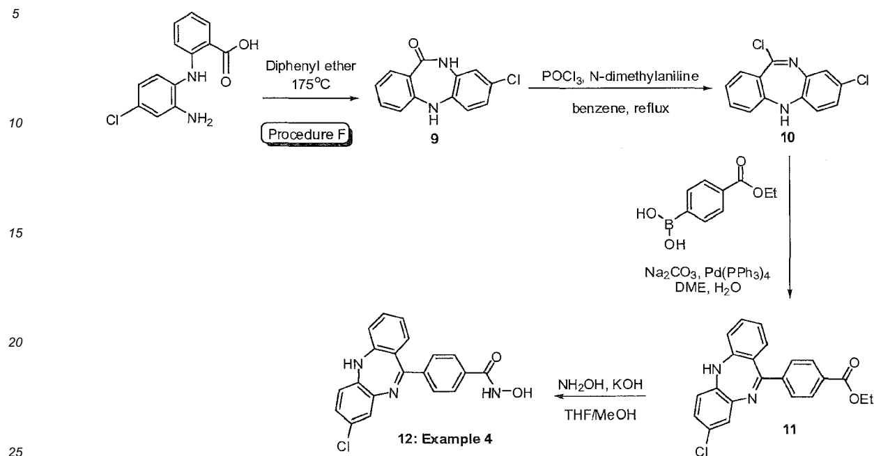
Scheme 4
