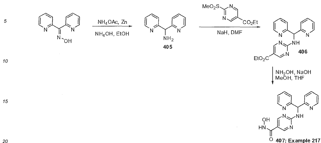
Scheme 67
