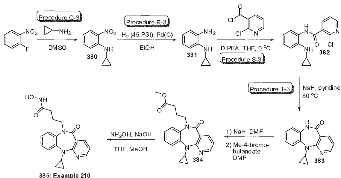
Scheme 60
