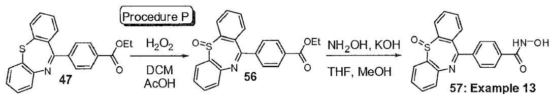
Scheme 13
