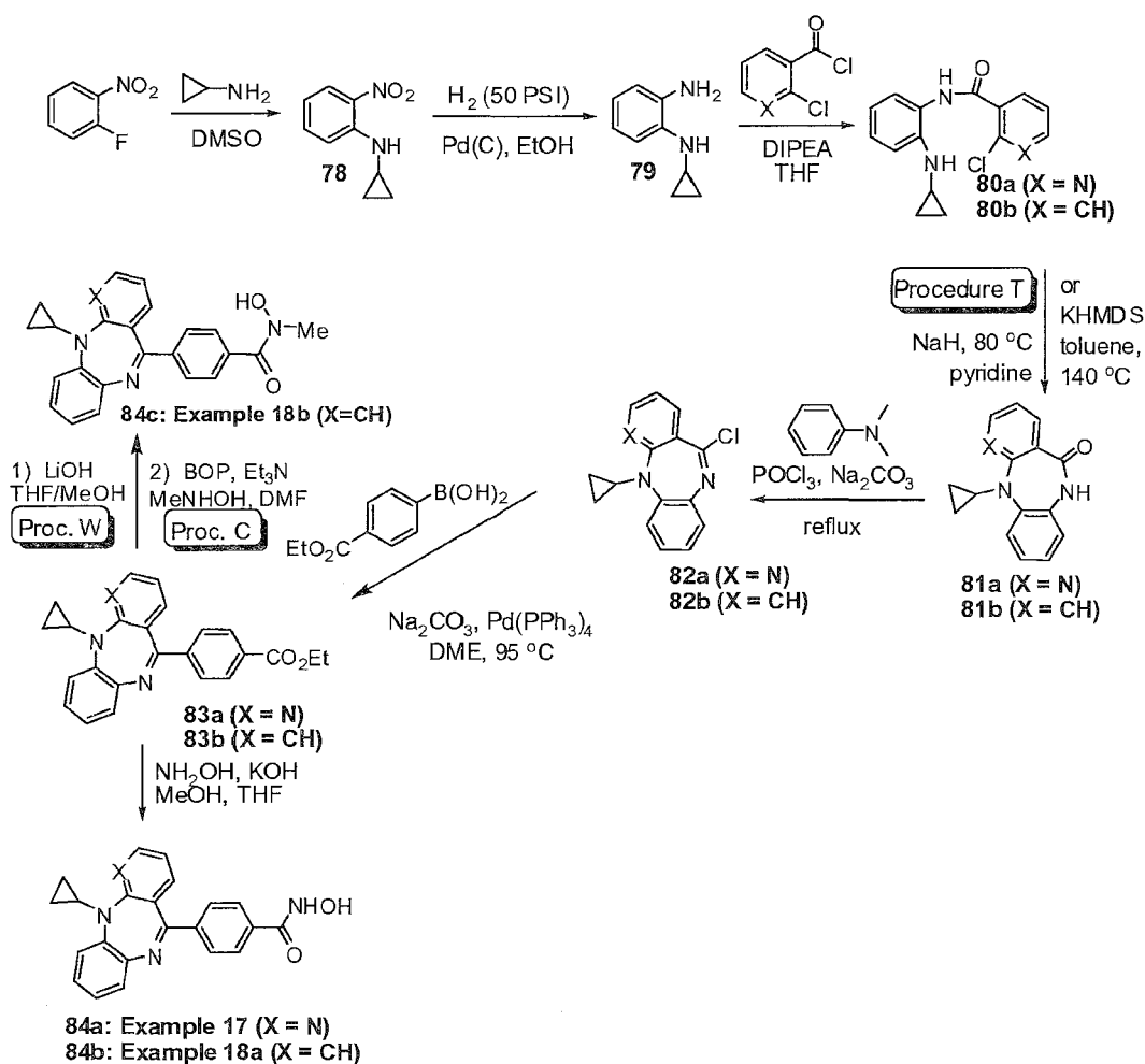
Scheme 17
