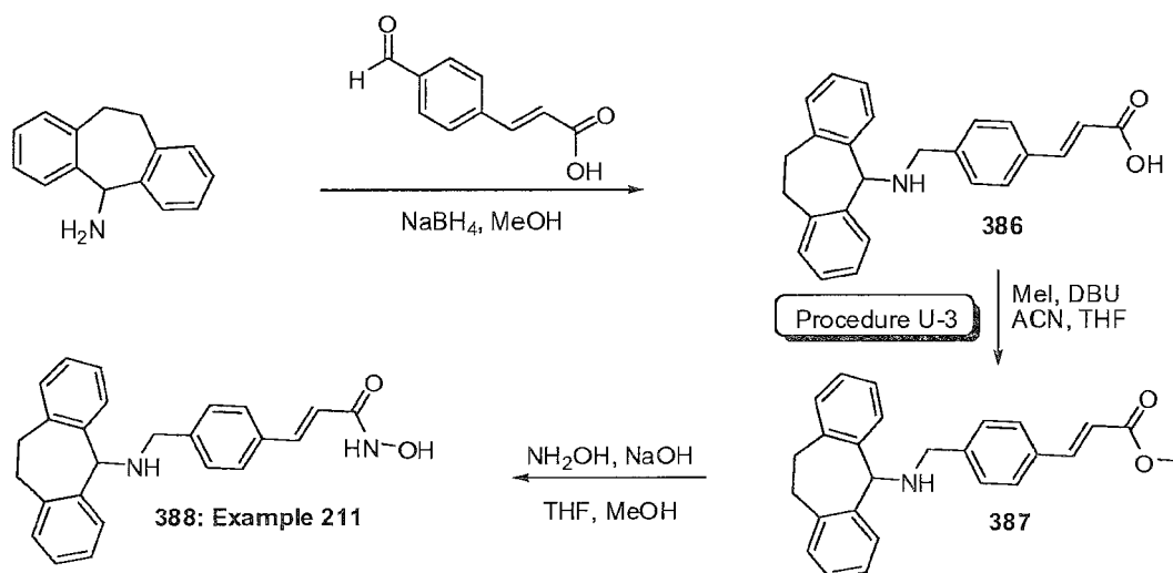
Scheme 61
