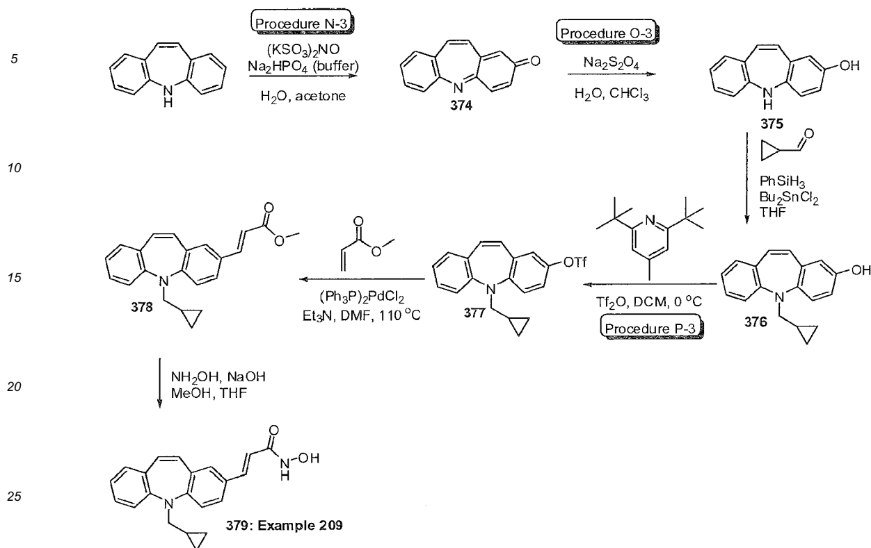
Scheme 59
