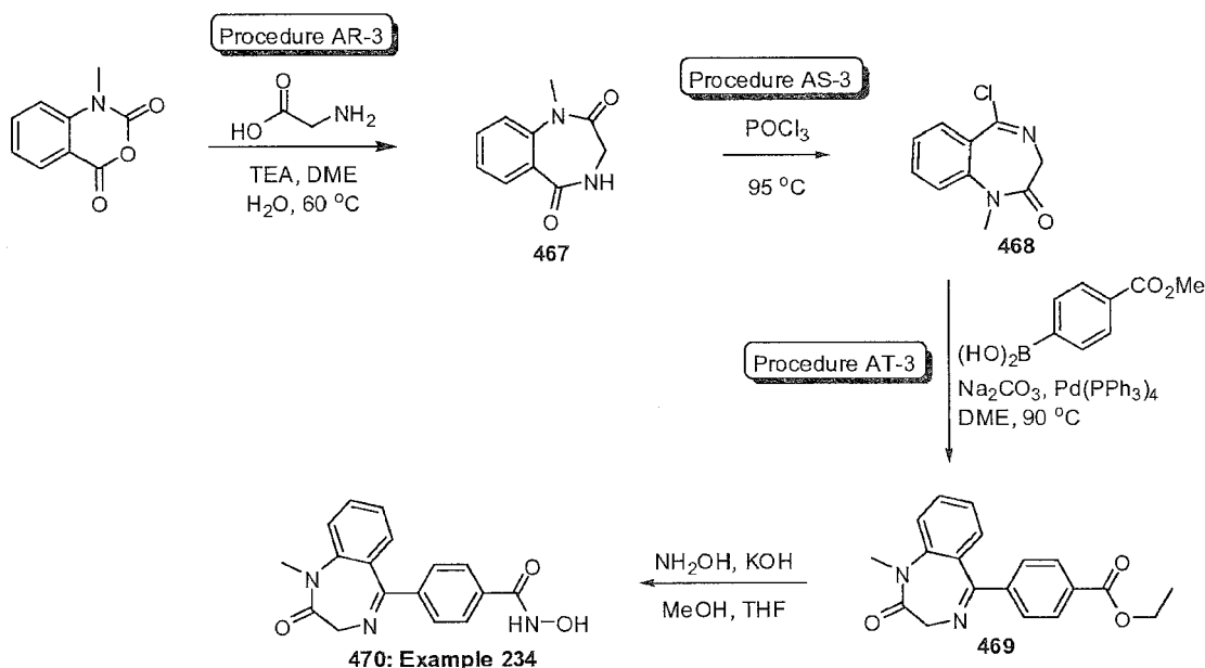
Scheme 84
