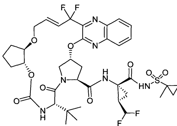
50 Compound 1
