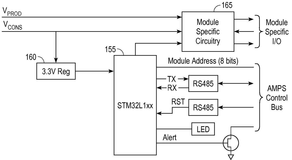
FIG. 10 – Generic Module Control Architecture
