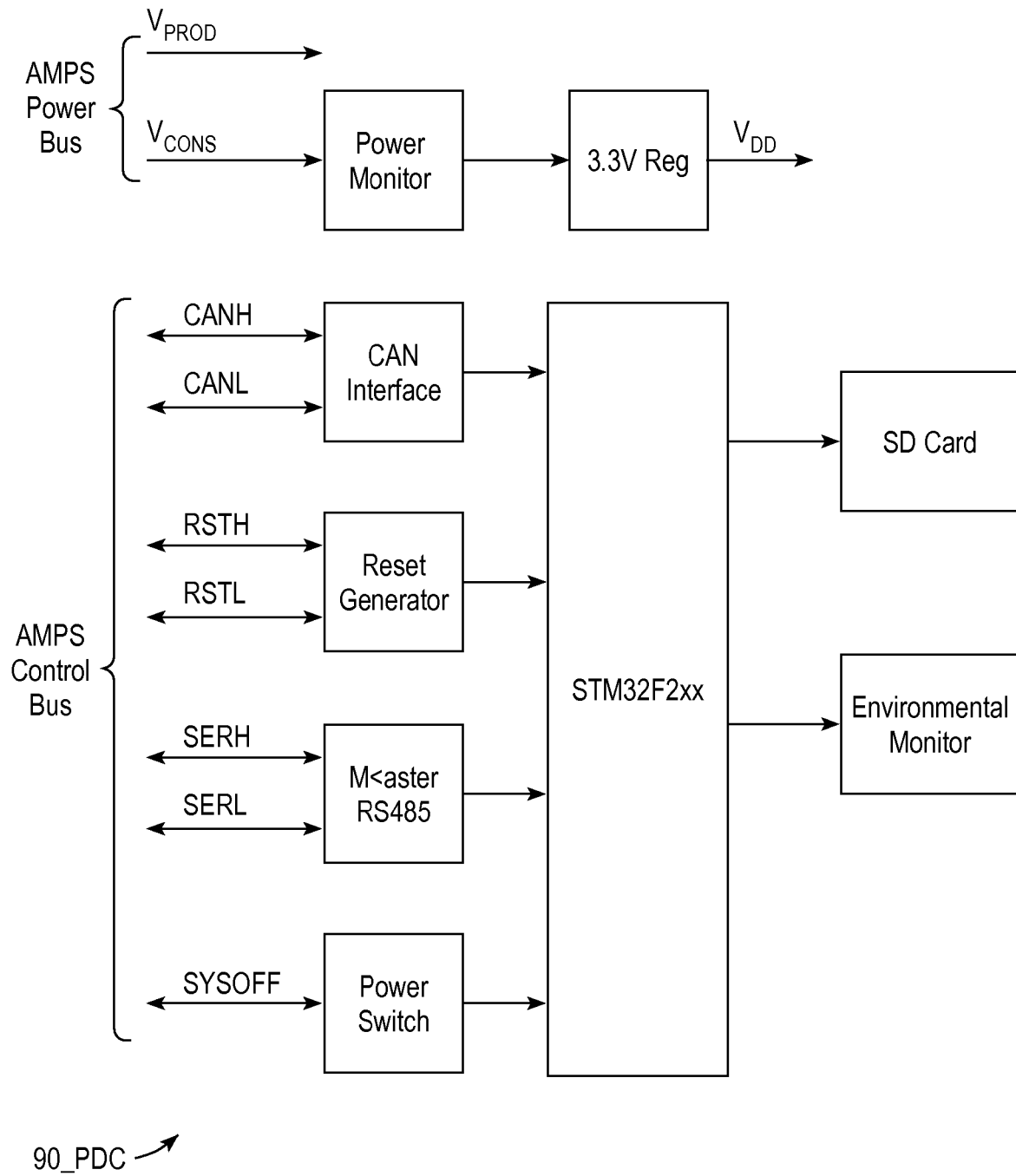
FIG. 11 – Power Domain Controller
