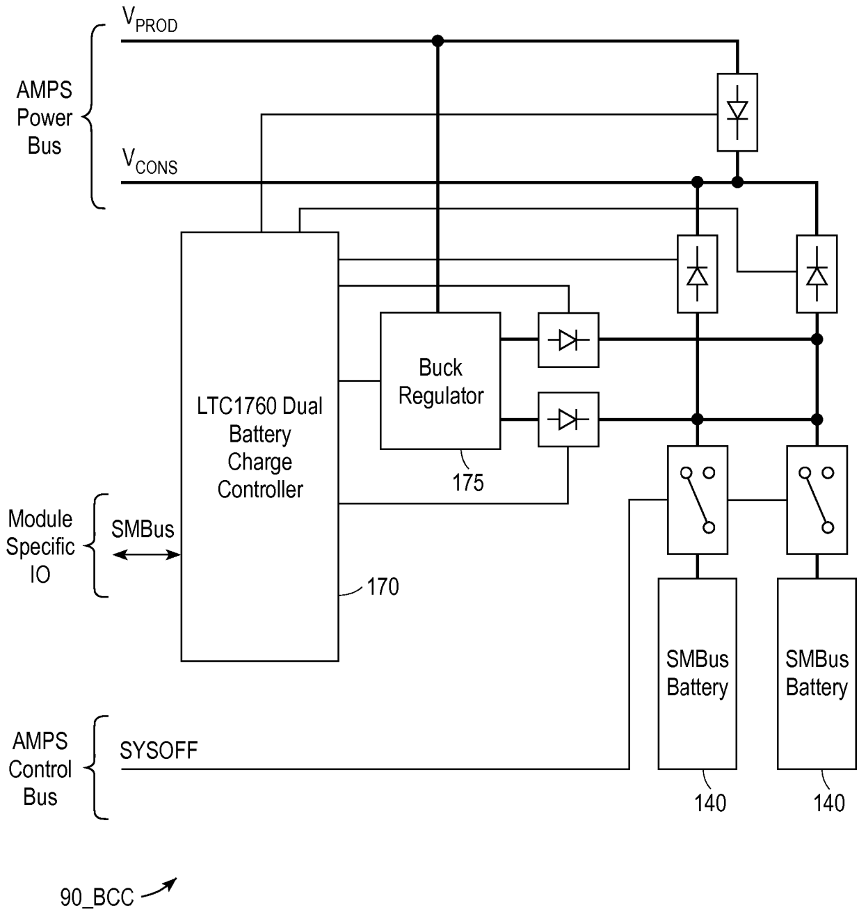
FIG. 12 – Battery Charger Control Module
