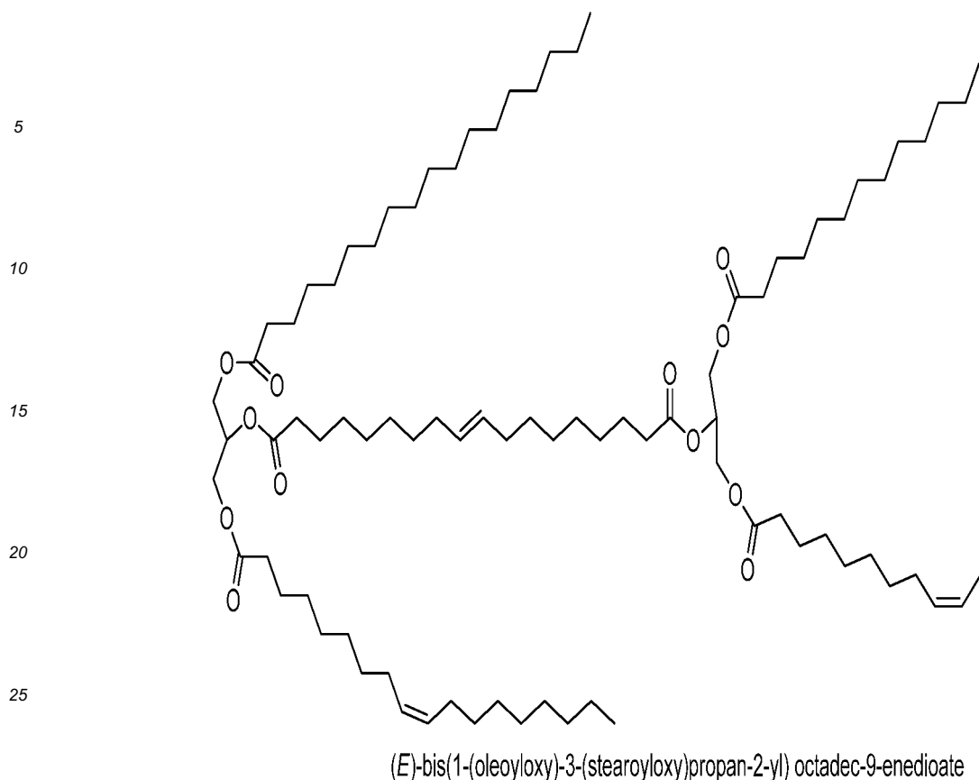
Scheme 1: Structure of (E)-1-(1-(oleoyloxy)-3-(stearoyloxy) propan-2-yl) 18-(1-(oleoyloxy)-3-(stearoyloxy)propan-2-yl) octadec-9-enedioate (Compound D).
