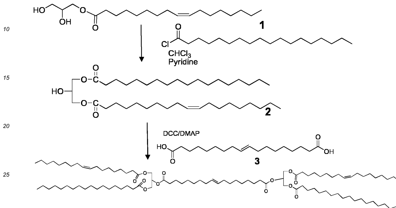
Scheme 2. Synthesis route of (E)-1-(1-(oleoyloxy)-3-(stearoyloxy)propan-2-yl) 18-(1-(oleoyloxy)-3-(stearoyloxy)propan-2-yl) octadec-9-enedioate (Compound D).
