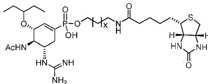
BM 5: (Tamiphosphor Guanidine)-(aliphatic chain Linker)-Biotin
