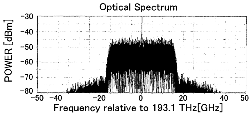
FIG. 6B OPTICAL SPECTRUM
