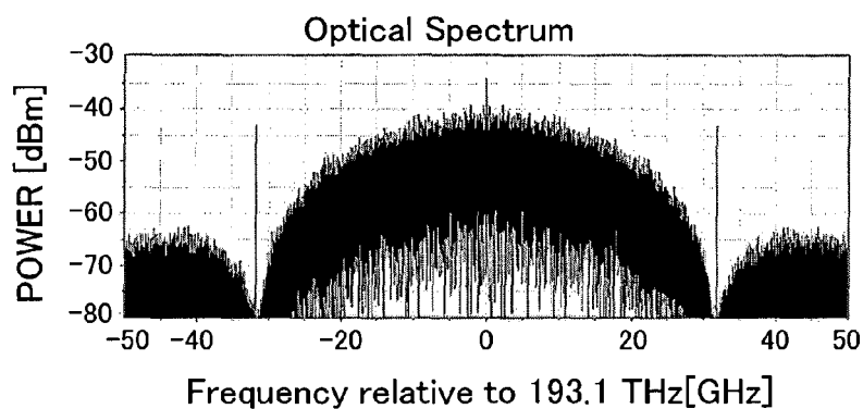
FIG. 5B OPTICAL SPECTRUM
