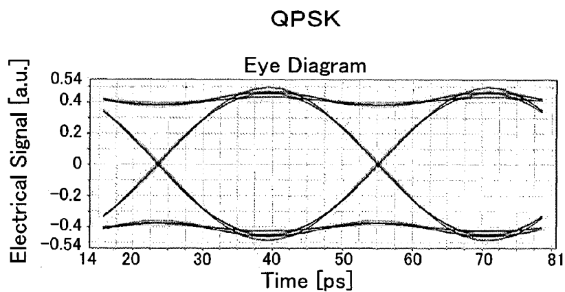
FIG. 5A ELECTRICAL MODULATED SIGNAL
