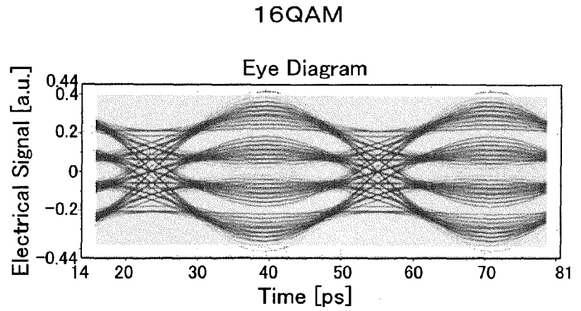
FIG. 7A ELECTRICAL MODULATED SIGNAL
