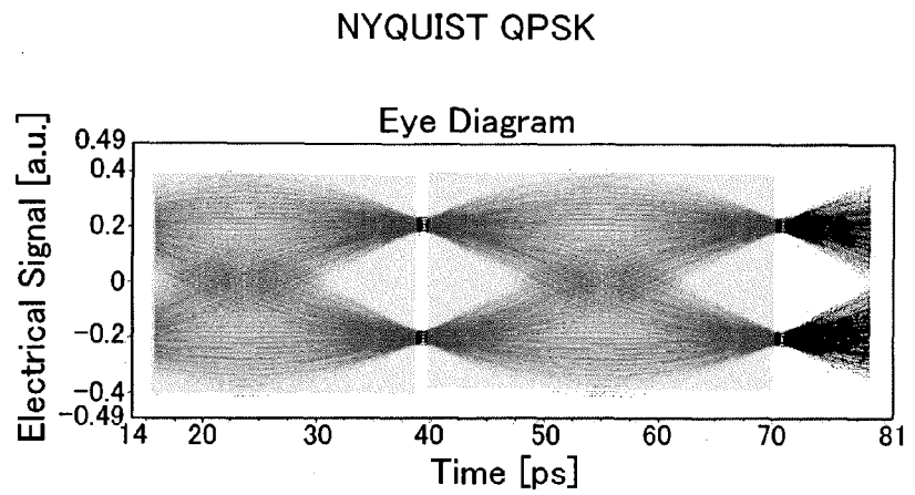
FIG. 6A ELECTRICAL MODULATED SIGNAL
