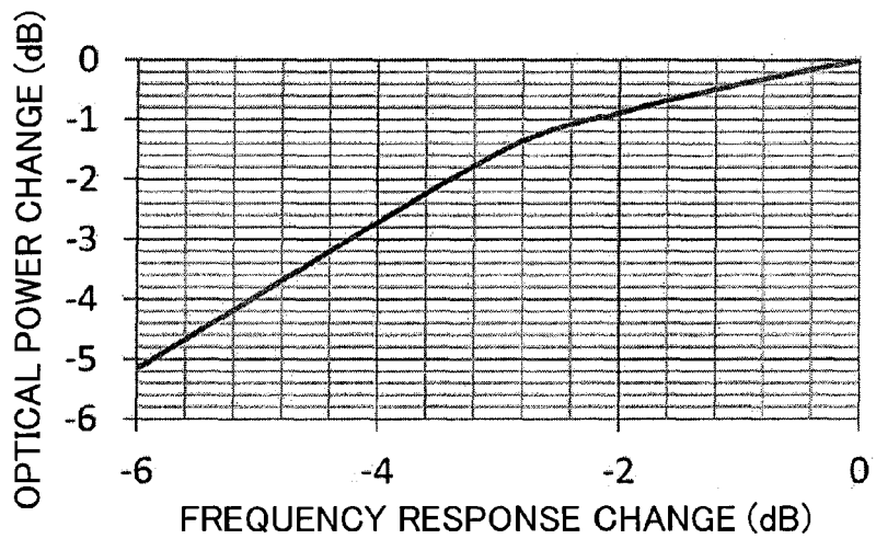
FIG. 6C FREQUENCY RESPONSE CHANGE VS OPTICAL POWER CHANGE
