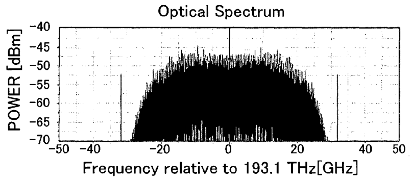
FIG. 7B OPTICAL SPECTRUM
