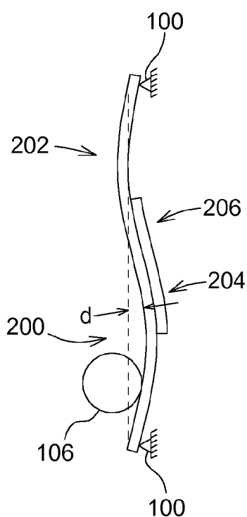
FIG. 9 Prior Art
