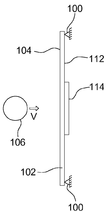
FIG. 3 Prior Art
