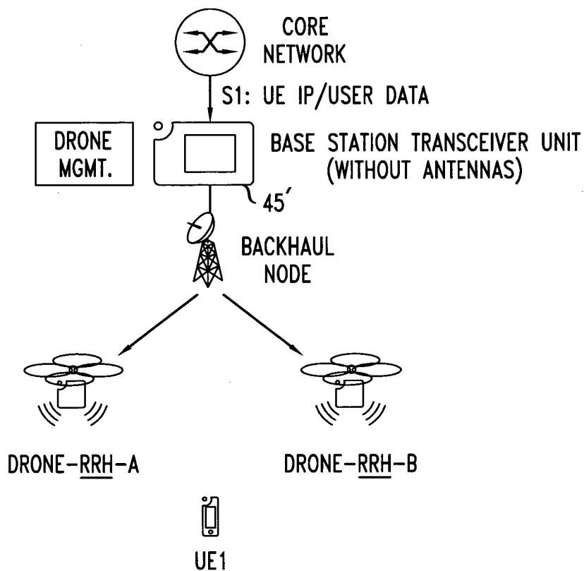
FIG. 14 ALTERNATIVE
