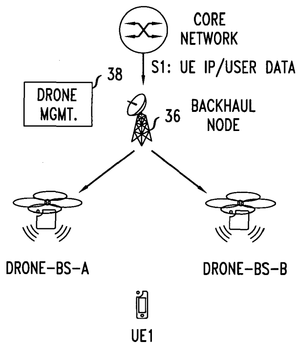
FIG. 11 DRONE WITH BASE STATION INCLUDING TRANSCEIVER
