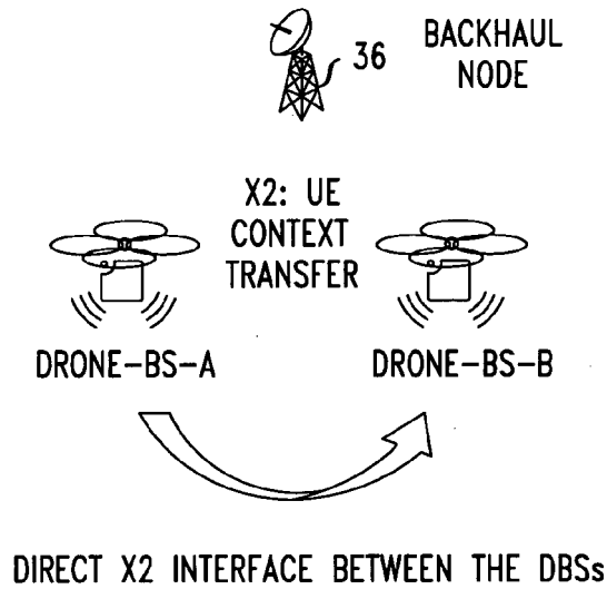
FIG. 9 ALTERNATIVE
