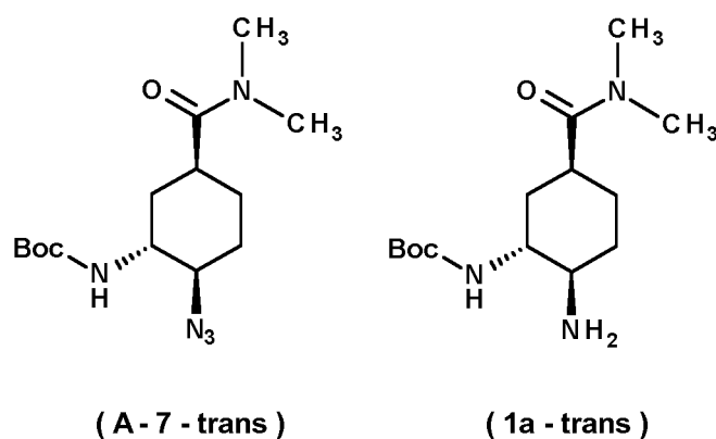
[trans-isomer]
