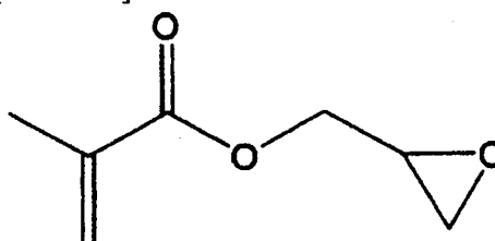
glycidyl methacrylate
