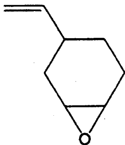
1, 2-epoxy-4-vinylcyclohexane
