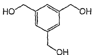
1,3,5-Tri(hydroxymethyl)benzene
