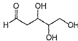
2-Deoxy-D-ribose
