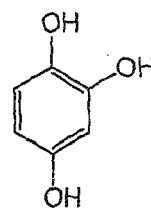
1,2,4-Trihydroxyl-benzene
