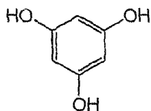
1,3,5-Trihydroxyl-benzene
