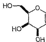
D-Galactal
