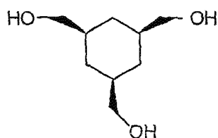
cis-1,3,5-Tri(hydroxymethyl)cyclohexane
