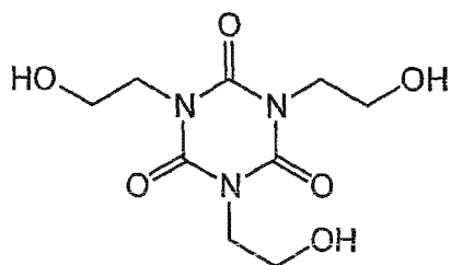
1,3,5-Tris(2-hydroxyethyl)-Cyanuric acid
