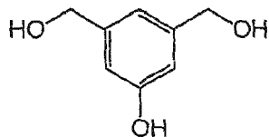
3,5-Di(hydroxymethyl)phenol
