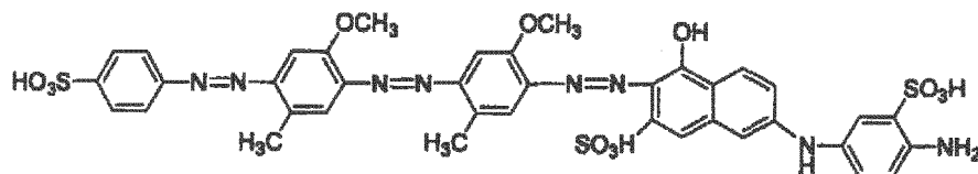
[Chemical formula 40]
