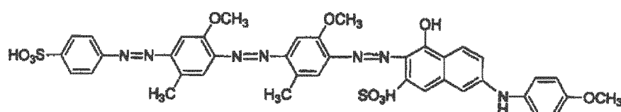
[Chemical formula 39]
