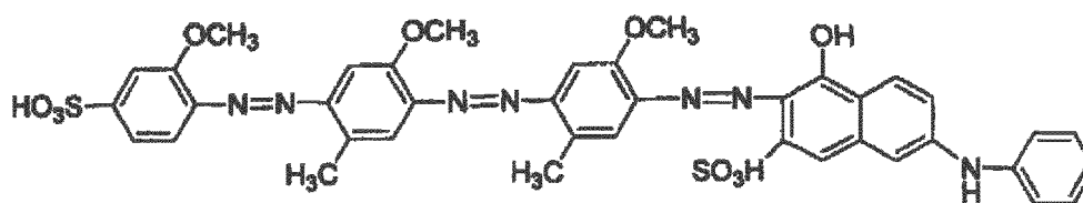
[Compound Example 29]
