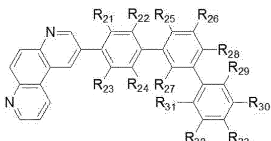
[Chemical Formula 22]
