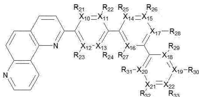
[Chemical Formula 13]
