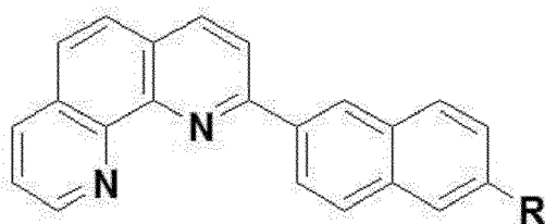
[Chemical Formula 5]
