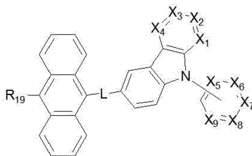
[Chemical Formula 25]
