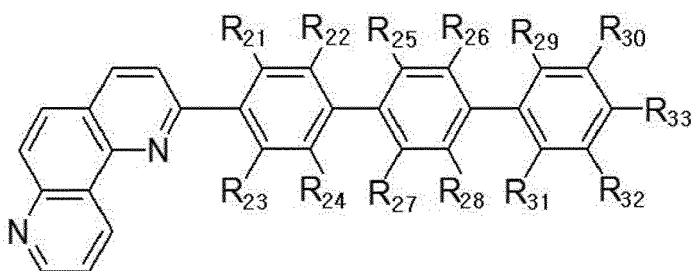
[Chemical Formula 19]
