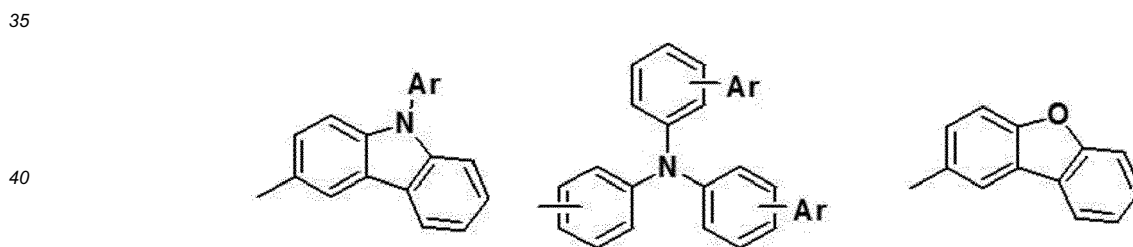
[Chemical Formula 2]
