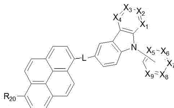
[Chemical Formula 25]
