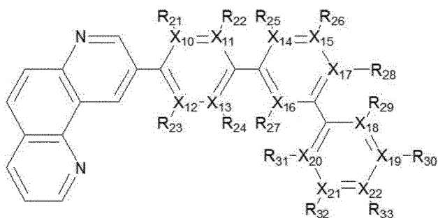
[Chemical Formula 13]
