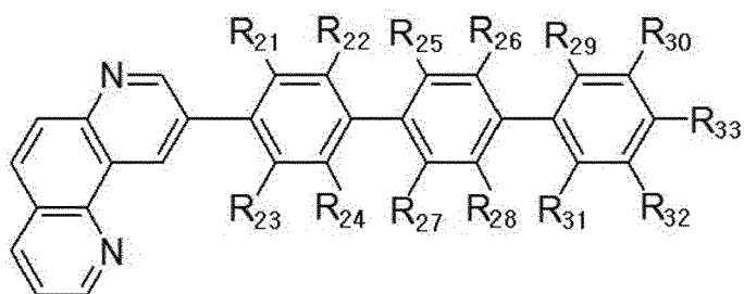
[Chemical Formula 18]
