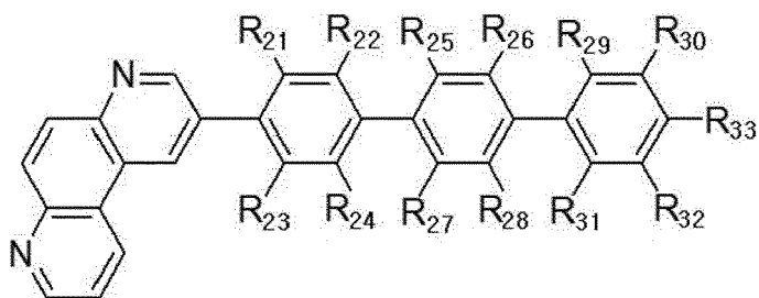
[Chemical Formula 18]
