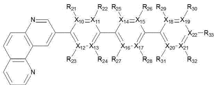
[Chemical Formula 9]
