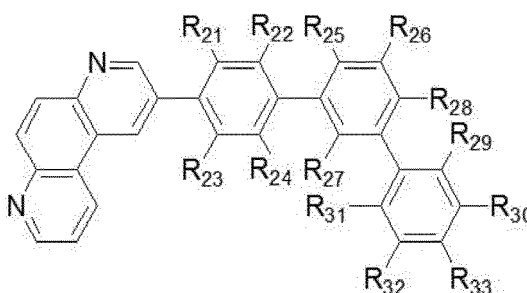
[Chemical Formula 21]
