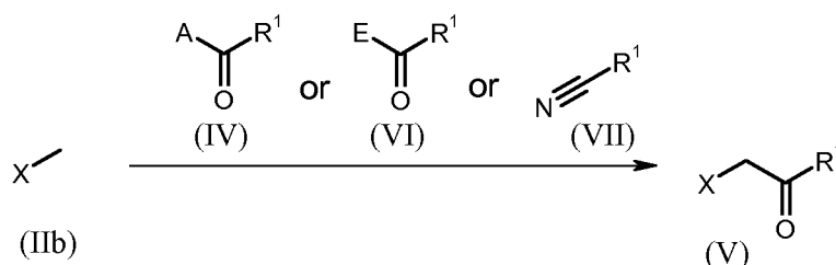
Scheme 2: Process B – Preparation of Ketones (V).
