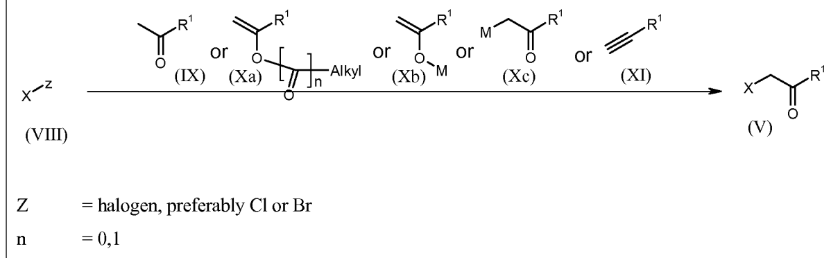
Scheme 3: Process C – Preparation of Ketones (V).
