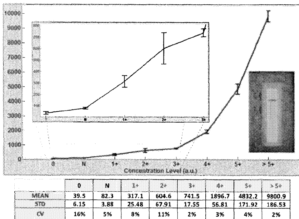
Figure 13 The summary of our measurements on the dry standard Orasure RDT kits which represents various concentration levels.
