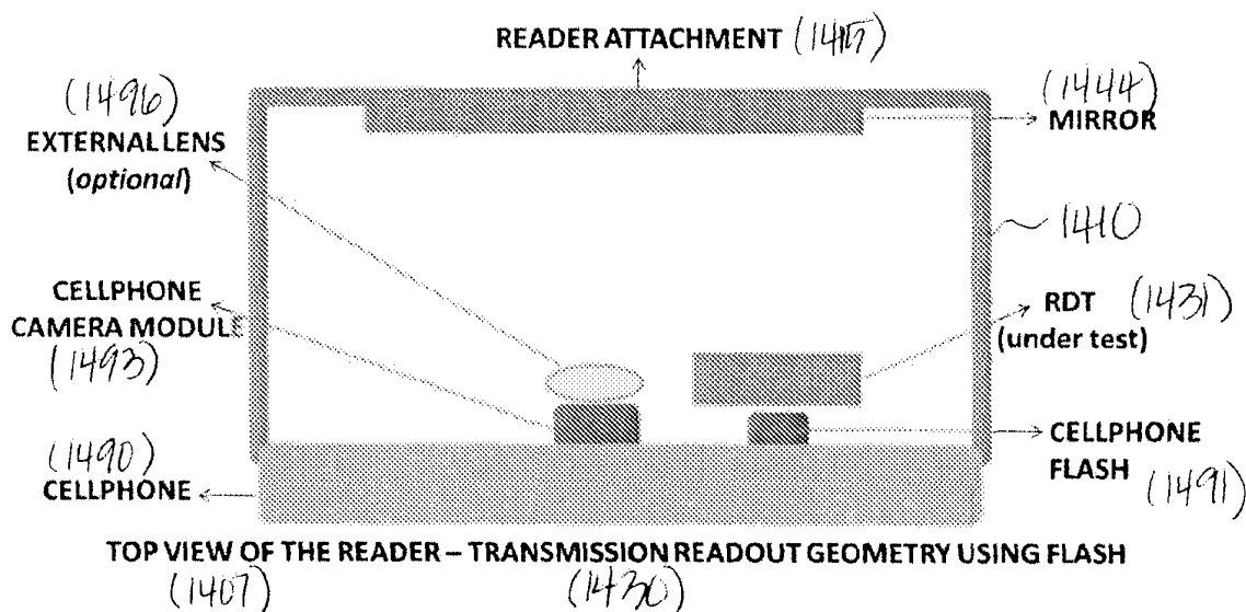
Figure 14 The schematics for the transmission imaging/readout modality using the cell-phone flash and a mirror.
