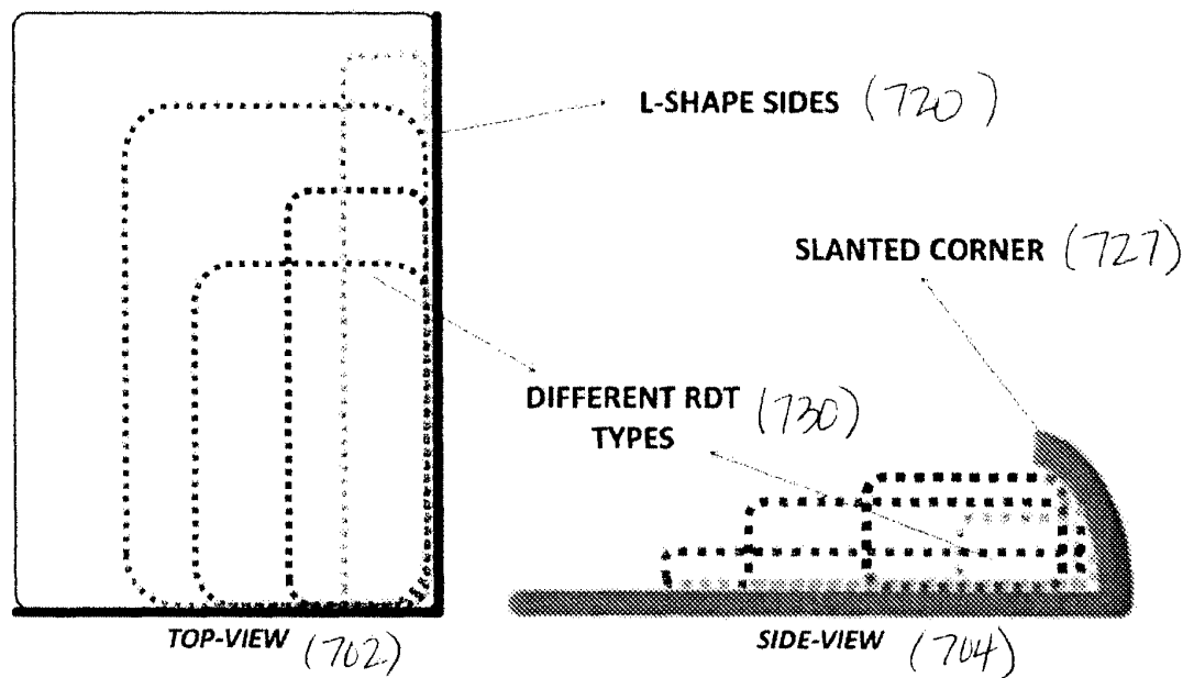
Figure 7-c Top-view schematics of the tray (left) and side-view schematics of the tray (right).
