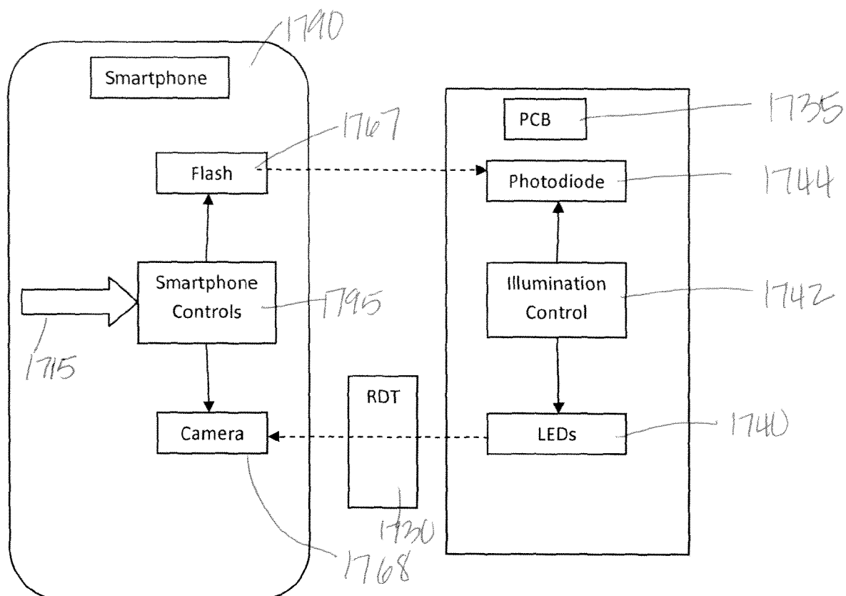
Figure17 Communication between the smartphone and tablet (application) and the embedded PCB
