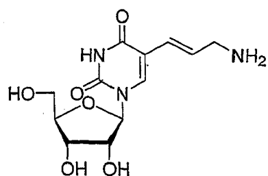
a. Alkylamino deoxythymidine
