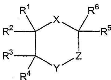
(LCM-2)
