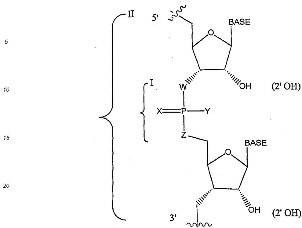
FORMULA 1
