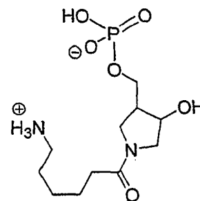
b. Abasic pyrrolidine cationic
