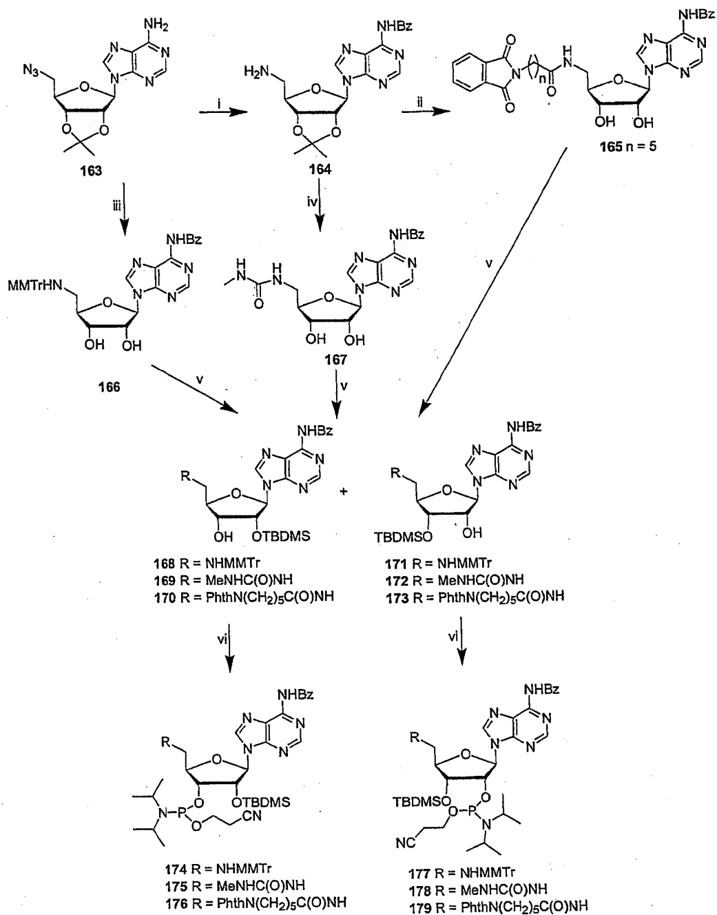
Scheme 8 a
