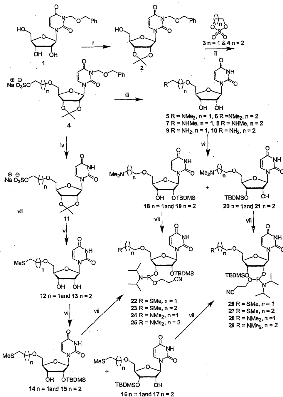
Scheme 1 a
