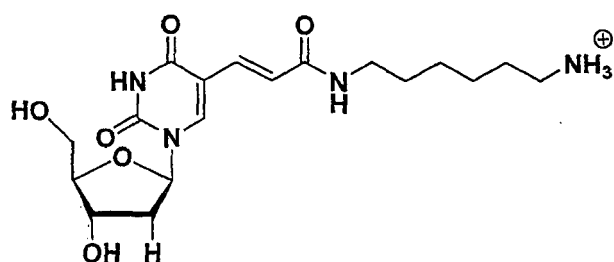
a. Alkylamino deoxythymidine
