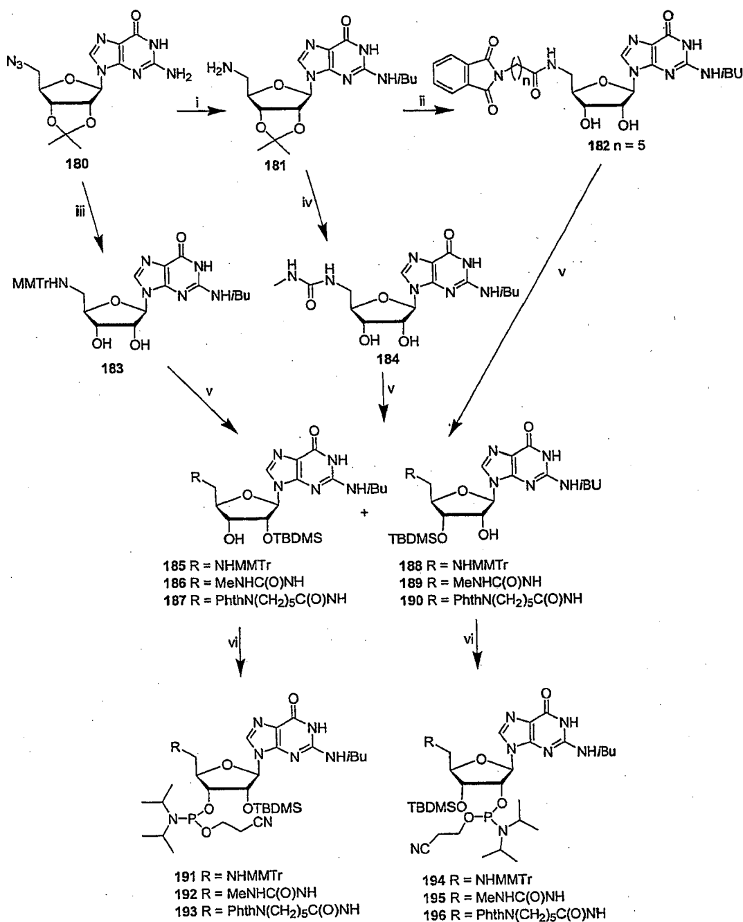
Scheme 9 a
