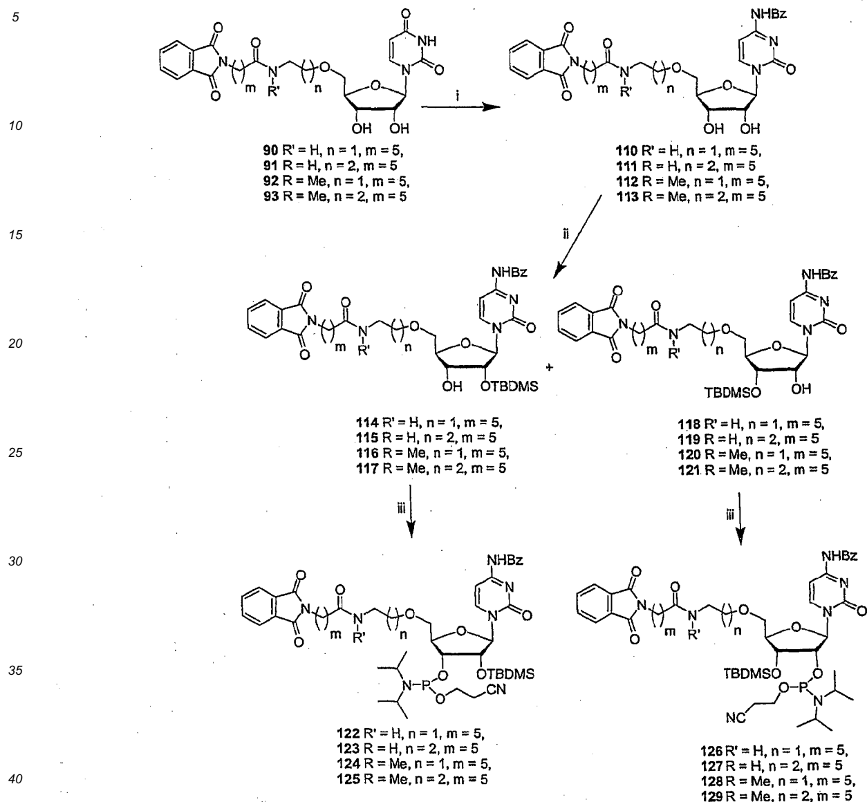
Scheme 5 a
