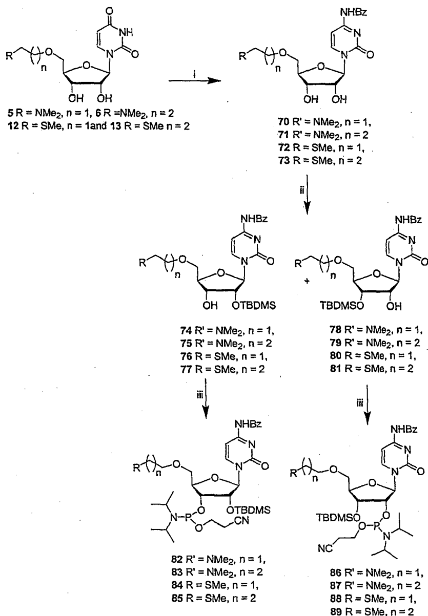
Scheme 3 a
