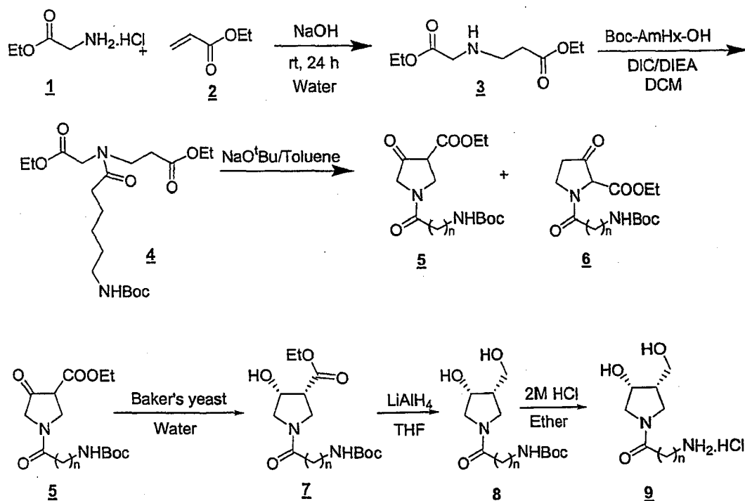
Scheme 1. Synthesis of cis-(-(3S,4R)-pyrrolidine diol
