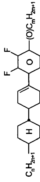
CPQY-n-(O)m
