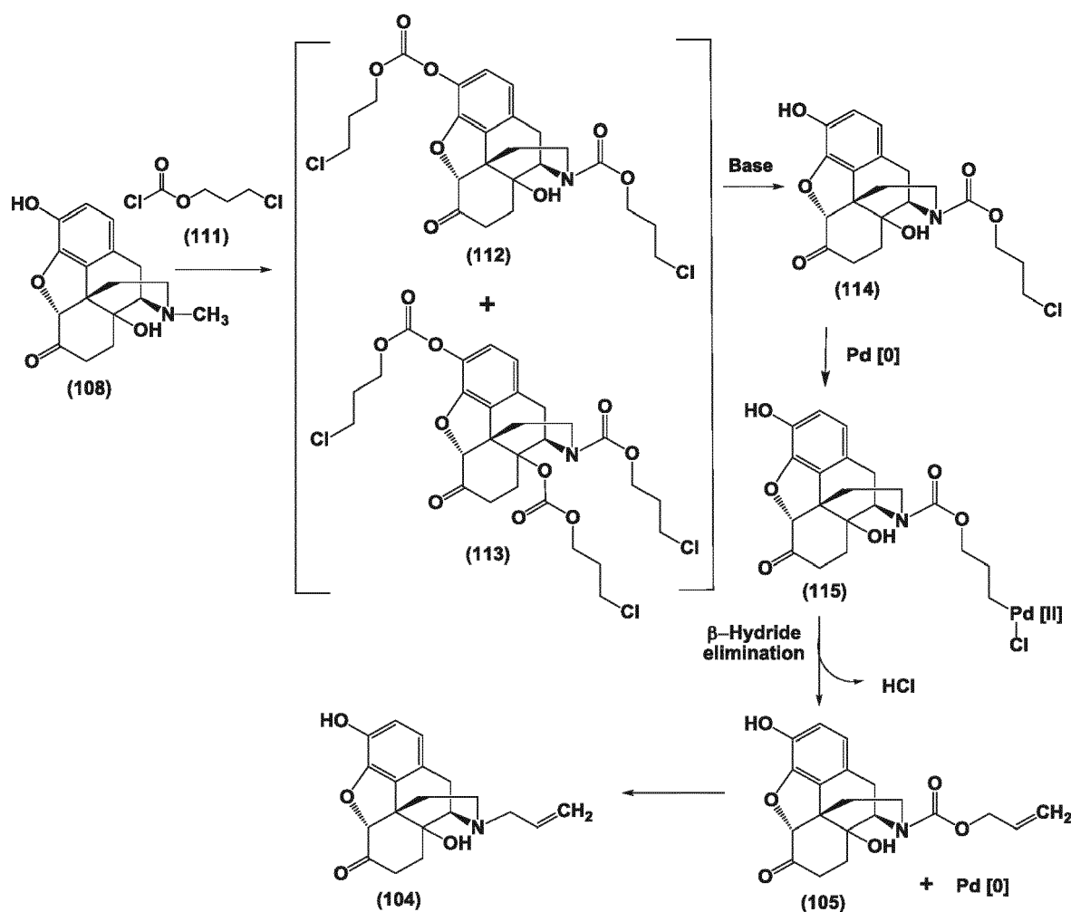
Scheme 12
