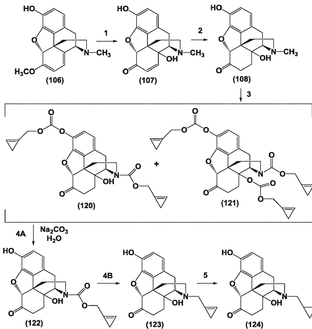
Scheme 16
