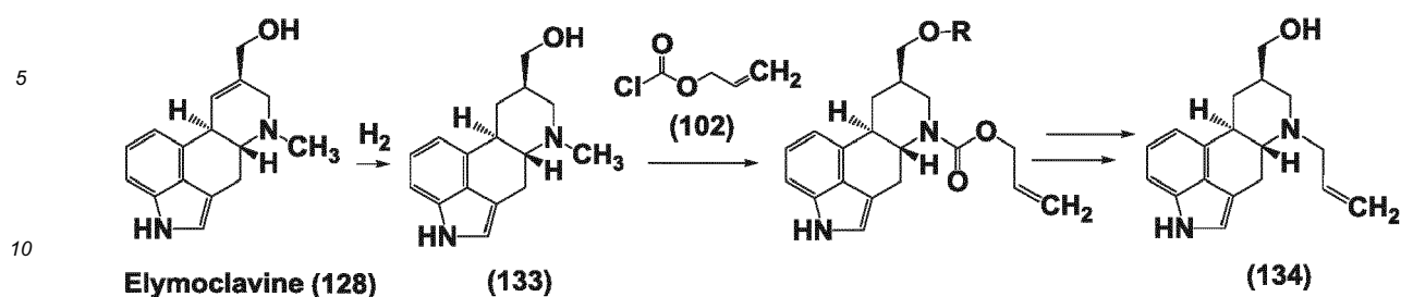
Scheme 21
