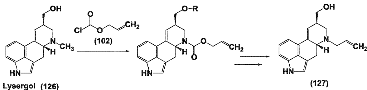
Scheme 17
