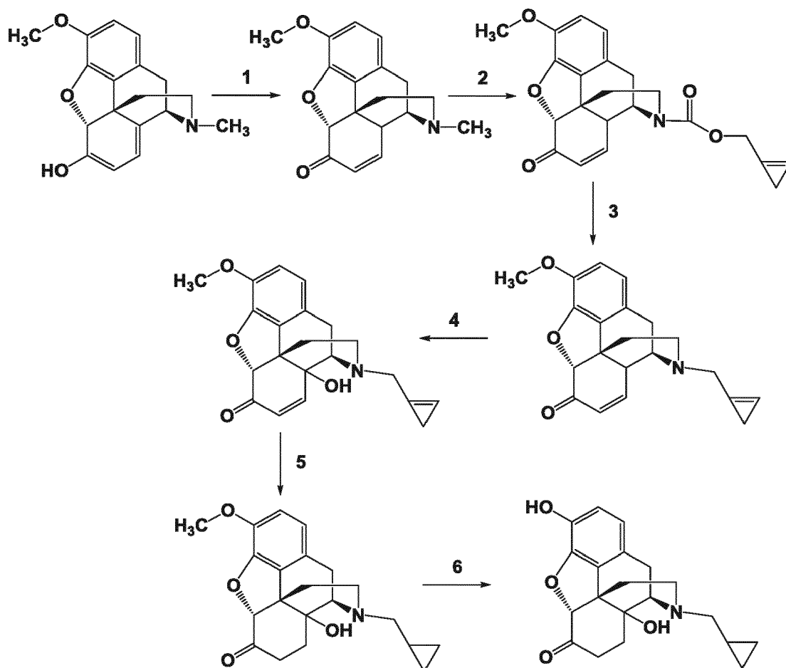
Scheme 33
