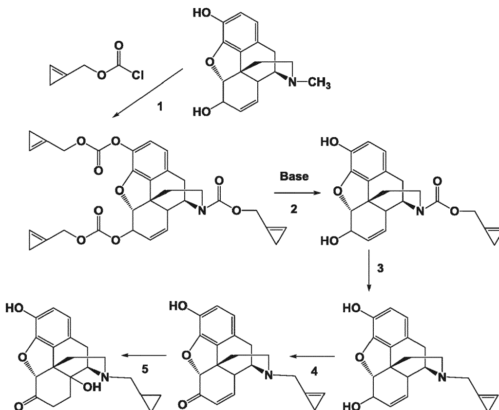
Scheme 31
