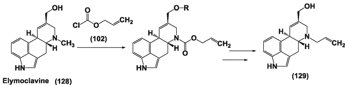
Scheme 18
