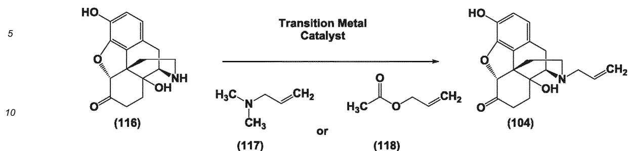
Scheme 13
