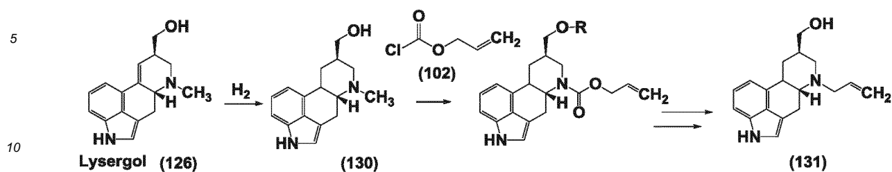
Scheme 19
