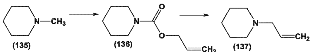
Scheme 23
