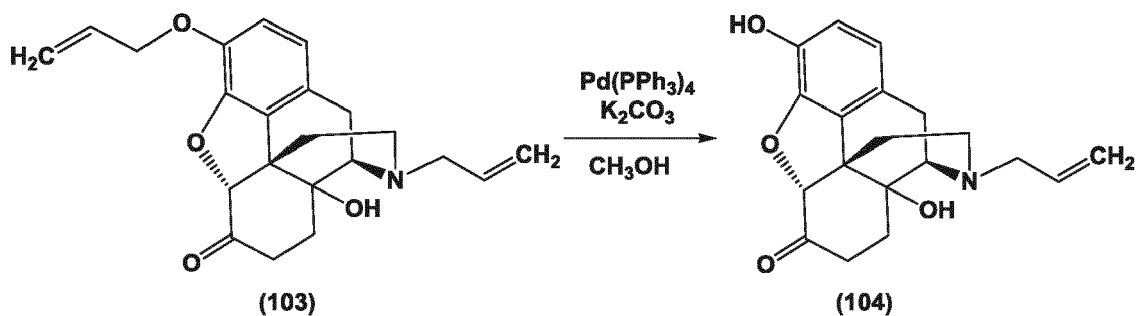
Scheme 4
