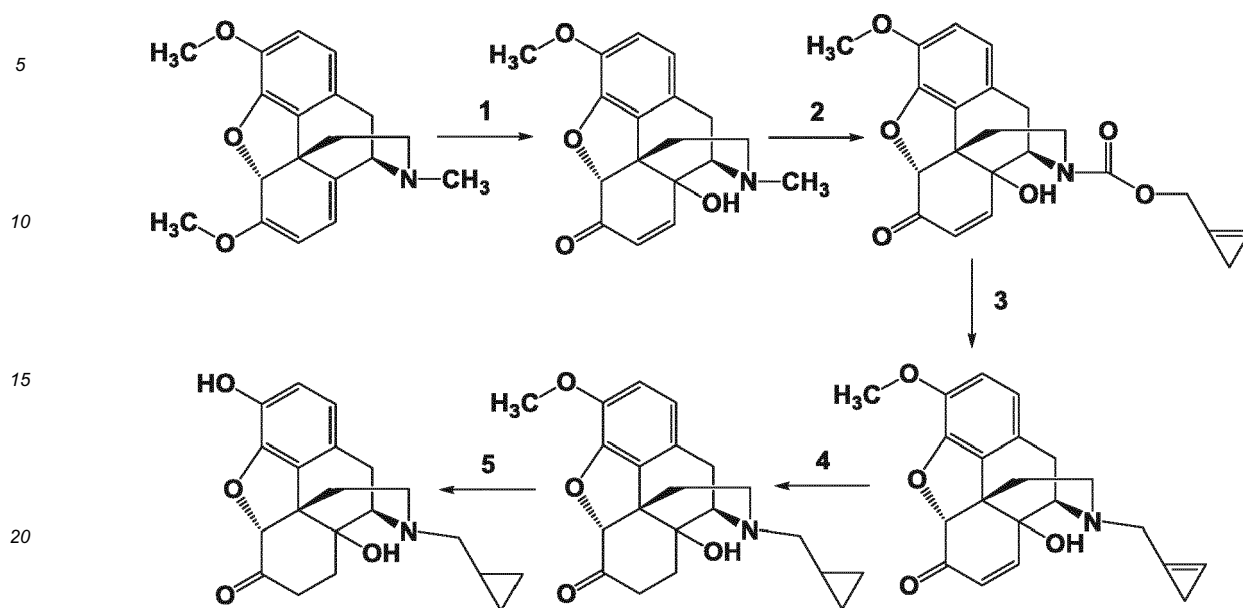
Scheme 34
