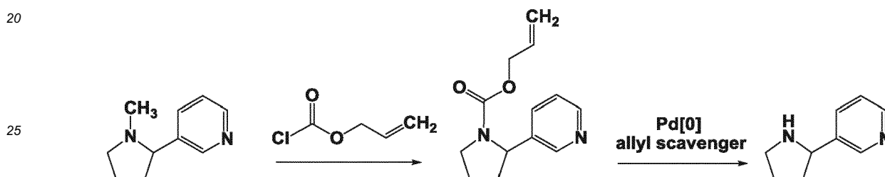
Scheme 28: Nicotine
