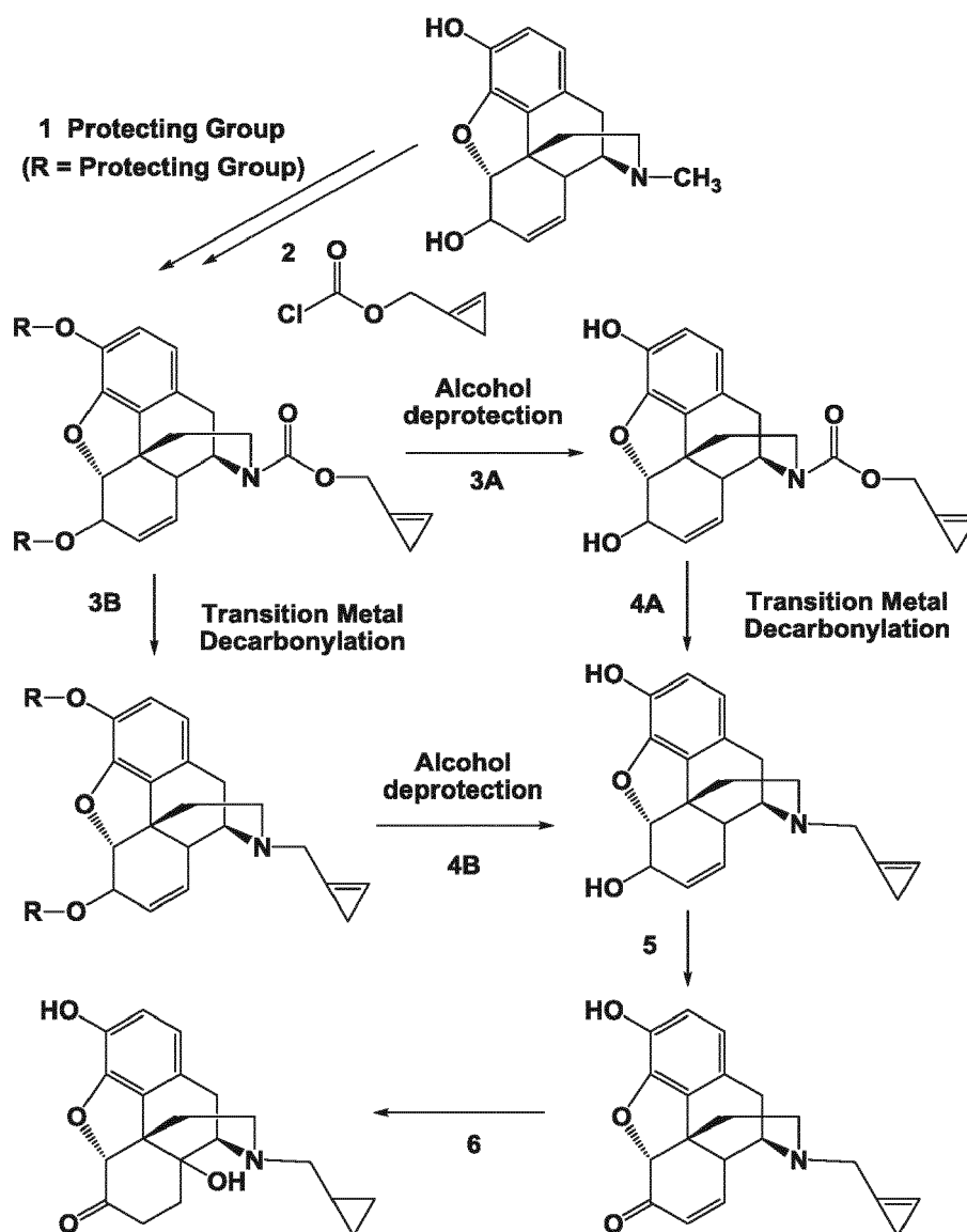
Scheme 32
