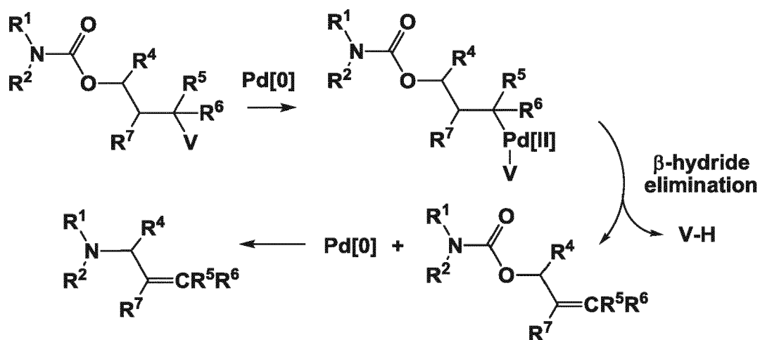
Scheme 29
