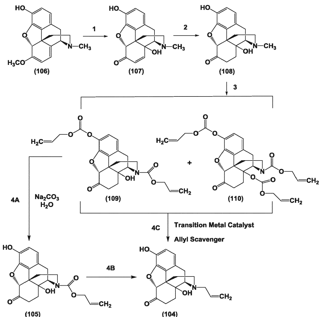
Scheme 10
