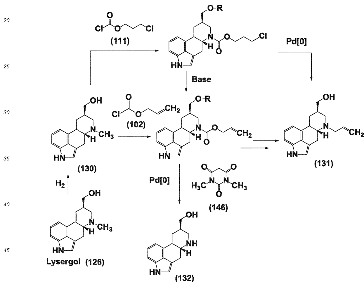
Scheme 20
