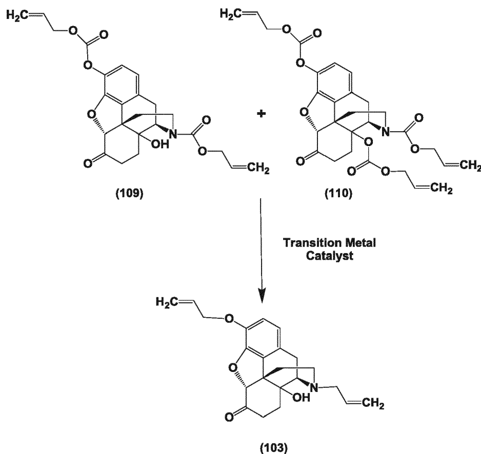
Scheme 7
