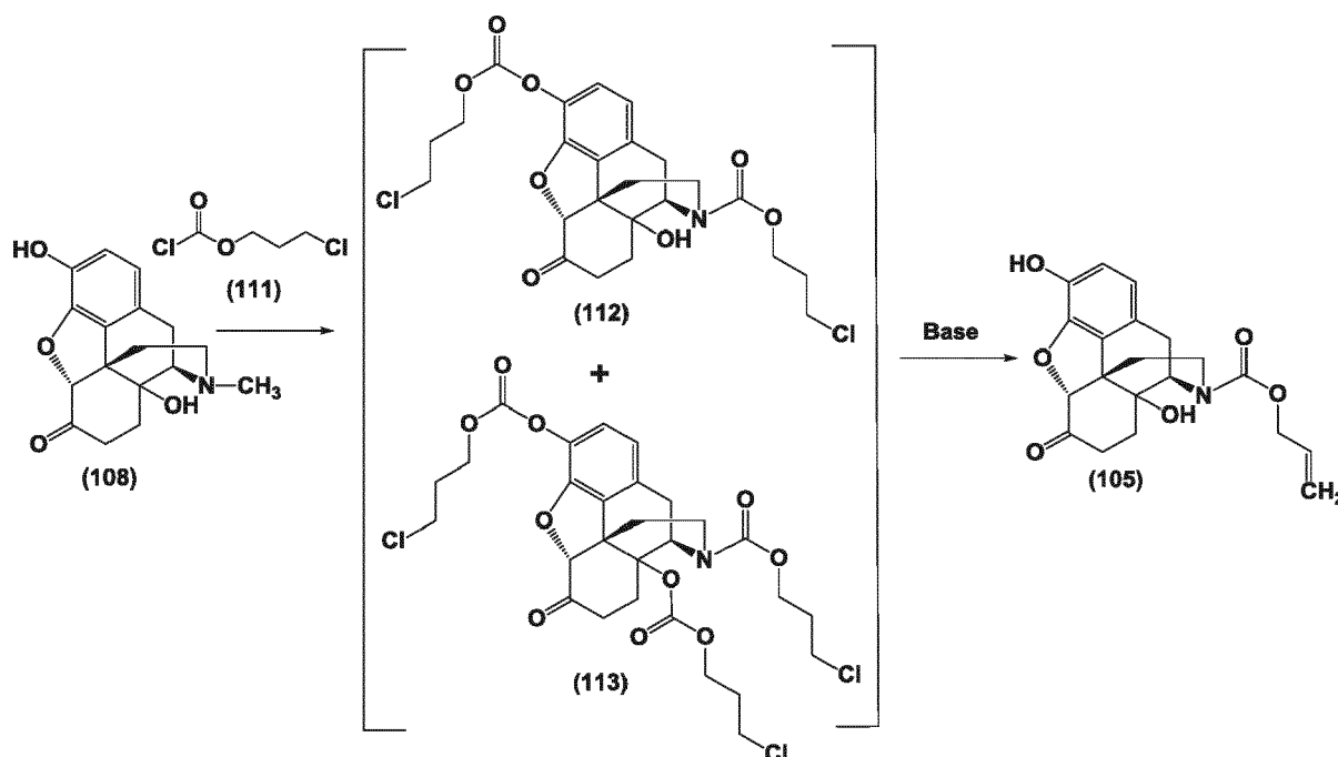
Scheme 11
