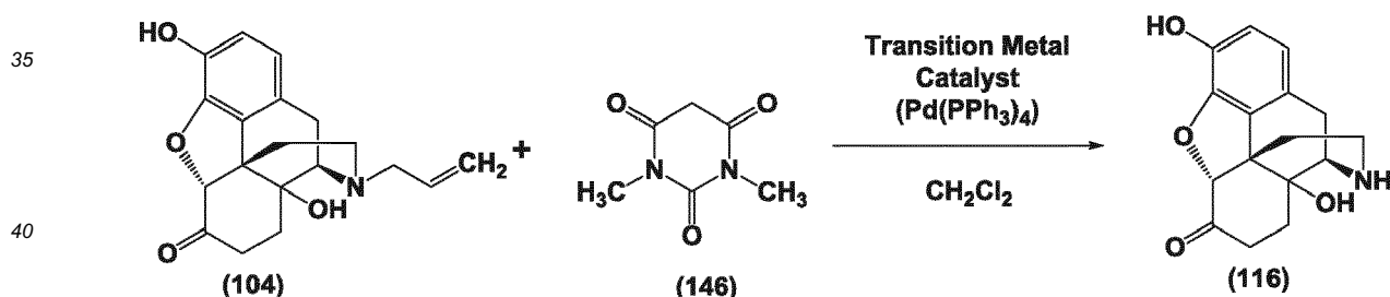
Scheme 14
