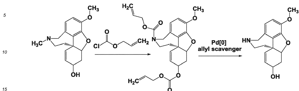
Scheme 28: Nicotine
