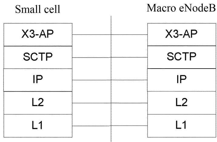
The control plane of second link interface
