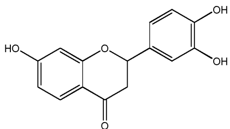
Isobutein (m/z = 272)
