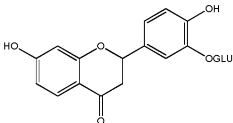
Isomonospermoside (m/z = 434)
