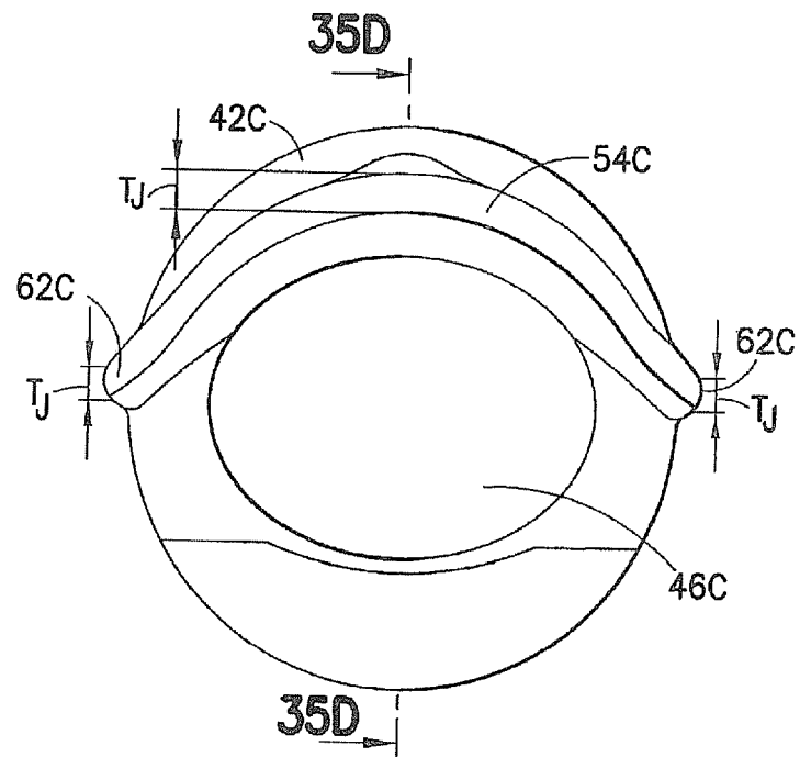
FIG.35C
