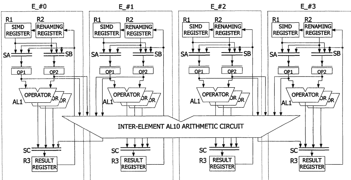
FIG.1 4SIMD OPERATOR
