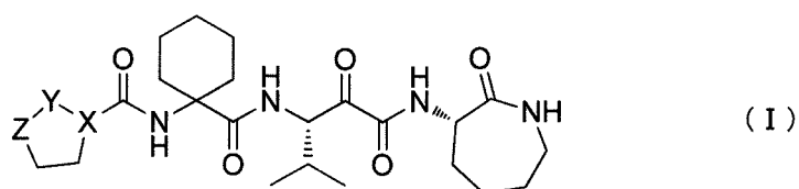
[Chemical Formula 1]
