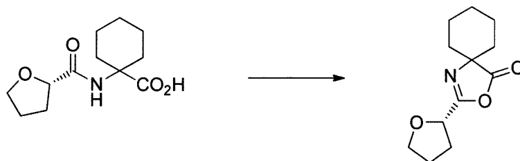
[Chemical Formula 20]
