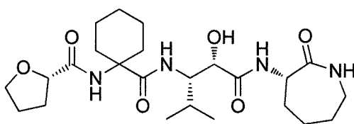
[Chemical Formula 19]
