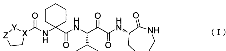
[Chemical Formula 1]
