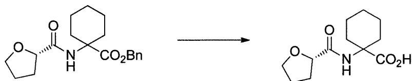
[Chemical Formula 18]
