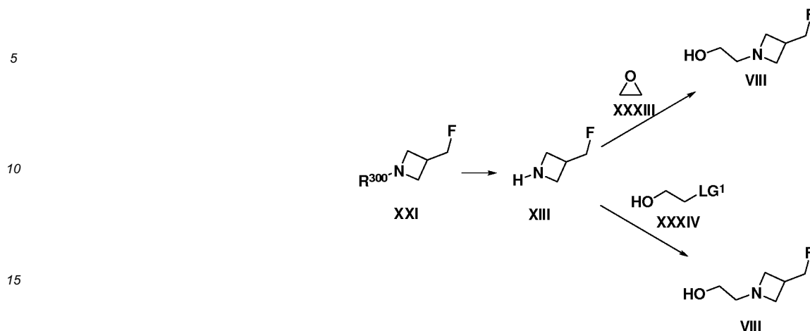
Scheme 10.
