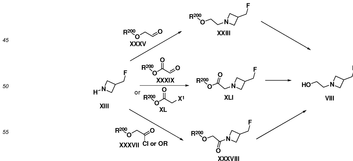
Scheme 11
