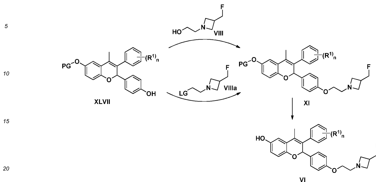
Scheme 13.
