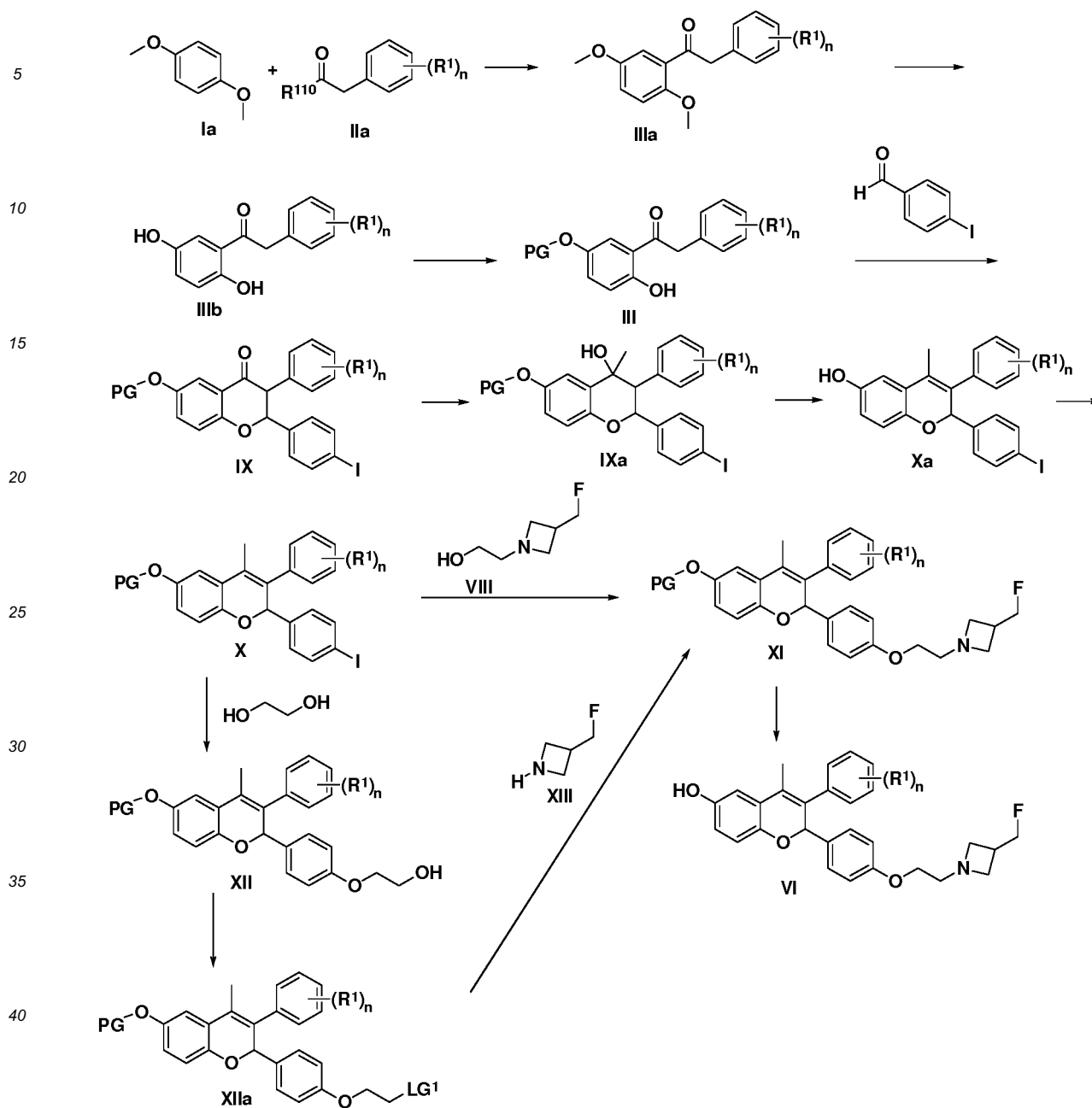
Scheme 3:
