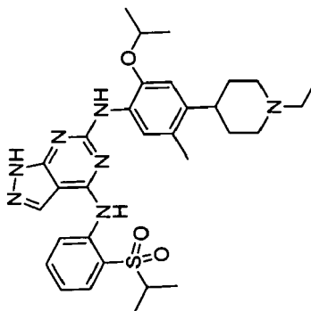
N6-(4-(1-ethylpiperidin-4-yl)-2-isopropoxy-5-methylphenyl)-N4-(2-(isopropylsulfonyl)phenyl)-1H-pyrazolo[3,4-d]pyrimidine-4,6-diamine
