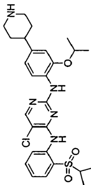
5-chloro-N2-(2-isopropoxy-4-(piperidin-4-yl)phenyl)-N4-(2-(pyrrolidin-1-ylsulfonyl)phenyl)pyrimidine-2,4-diamine
