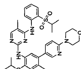
N2-(2-isopropoxy-4-methyl-5-(6-morpholinopyridin-3-yl)phenyl)-N4-(2-(isopropylsulfonyl)phenyl)-5-methylpyrimidine-2,4-diamine
