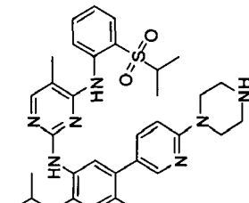
N2-(2-isopropoxy-4-methyl-5-(6-(piperazin-1-yl)pyridin-3-yl)phenyl)-N4-(2-(isopropylsulfonyl)phenyl)-5-methylpyrimidine-2,4-diamine
