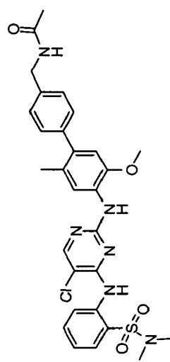
4-(5-chloro-4-(2-(N,N-dimethylsulfamoyl)phenylamino)pyrimidin-2-ylamino)-N-cyclopropyl-5'-methoxy-2'-methylbiphenyl-4-carboxamide
