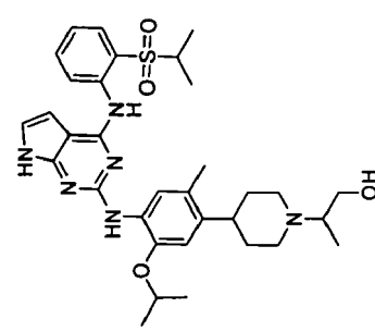
N2-(4-(1-ethylpiperidin-4-yl)-2-isopropoxy-5-methylphenyl)-N4-(2-(isopropylsulfonyl)phenyl)-7H-pyrrolo[2,3-d]pyrimidine-2,4-diamine
