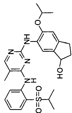
6-(4-(2-(isopropylsulfonyl)phenylamino)-5-methylpyrimidin-2-ylamino)-2,3-dihydro-5-isopropoxy-1H-inden-1-ol
