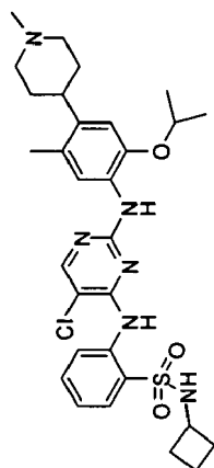
5-chloro-N2-(2-isopropoxy-5-methyl-4-(1-methylpiperidin-4-yl)phenyl)-N4-(2-(pyrrolidin-1-yl)sulfonyl)pyrimidine-2,4-diamine
