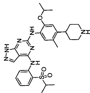
N6-(2-isopropoxy-5-methyl-4-(piperidin-4-yl)phenyl)-N4-(2-(isopropylsulfonyl)phenyl)-1H-pyrazolo[3,4-d]pyrimidine-4,6-diamine
