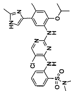
2-(5-chloro-2-(2-isopropoxy-4-methyl-5-(2-methyl-1H-imidazol-4-yl)phenylamino)pyrimidin-4-ylamino)-N,N-dimethylbenzenesulfonamide
