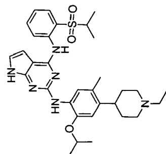
N2-(2-isopropoxy-5-methyl-4-(piperidin-4-yl)phenyl)-N4-(2-(methylsulfonyl)phenyl)-7H-pyrrolo[2,3-d]pyrimidine-2,4-diamine
