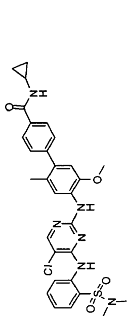
4-(5-chloro-4-(2-(N,N-dimethylsulfamoyl)phenylamino)pyrimidin-2-ylamino)-N-cyclopropyl-5'-methoxy-2'-methylbiphenyl-4-carboxamide
