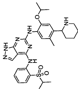
N6-(2-isopropoxy-5-methyl-4-(piperidin-2-yl)phenyl)-N4-(2-(isopropylsulfonyl)phenyl)-1H-pyrazolo[3,4-d]pyrimidine-4,6-diamine
