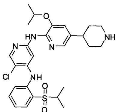
5-chloro-N2-(3-isopropoxy-5-(piperidin-4-yl)pyridin-2-yl)-N4-(2-(isopropylsulfonyl)phenyl)pyridine-2,4-diamine
