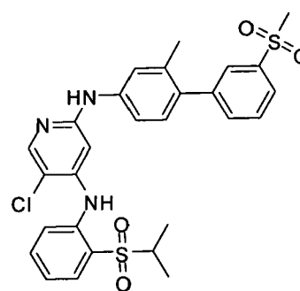
5-chloro-N4-(2-(isopropylsulfonyl)phenyl)-N2-(2-methyl-3'-(methylsulfonyl)biphenyl-4-yl)pyridine-2,4-diamine
