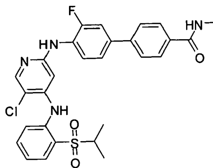
4'-(5-chloro-4-(2-(isopropylsulfonyl)phenylamino)pyridin-2-ylamino)-3'-fluoro-N-methylbiphenyl-4-carboxamide
