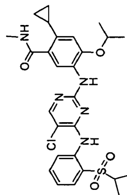
5-(4-(2-(isopropylsulfonyl)phenylamino)-5-chloropyrimidin-2-ylamino)-4-isopropoxy-2-methyl-N-(1-methylpiperidin-4-yl)benzamide
