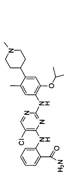
2-(2-(2-isopropoxy-5-methyl-4-(1-methylpiperidin-4-yl)phenylamino)-5-chloropyrimidin-4-ylamino) benzamide
