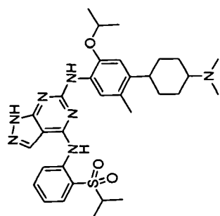
N6-(4-(4-(dimethylamino)cyclohexyl)-2-isopropoxy-5-methylphenyl)-N4-(2-(isopropylsulfonyl)phenyl)-1H-pyrazolo[3,4-d]pyrimidine-4,6-diamine
