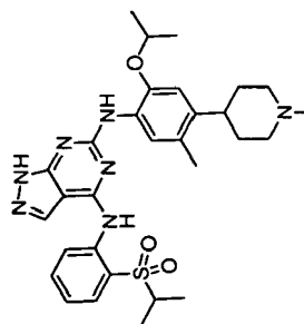
N6-(4-(1-ethylpiperidin-4-yl)-2-isopropoxy-5-methylphenyl)-N4-(2-(isopropylsulfonyl)phenyl)-1H-pyrazolo[3,4-d]pyrimidine-4,6-diamine
