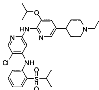
5-chloro-N2-(5-(1-ethylpiperidin-4-yl)-3-isopropoxypyridin-2-yl)-N4-(2-(isopropylsulfonyl)phenyl)pyridine-2,4-diamine
