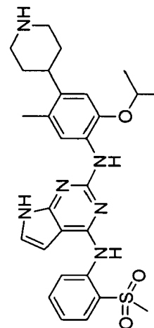
N2-(2-isopropoxy-5-methyl-4-(piperidin-4-yl)phenyl)-N4-(2-(methylsulfonyl)phenyl)-7H-pyrrolo[2,3-d]pyrimidine-2,4-diamine
