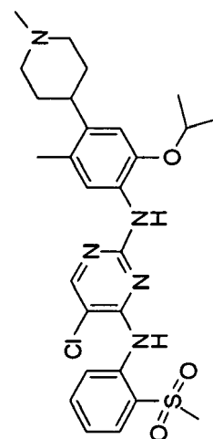
5-chloro-N2-(2-isopropoxy-5-methyl-4-(1-methylpiperidin-4-yl)phenyl)-N4-(2-(aminosulfonyl)phenyl)pyrimidine-2,4-diamine
