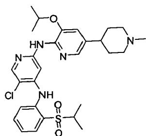
5-chloro-N2-(3-isopropoxy-5-(piperidin-4-yl)pyridin-2-yl)-N4-(2-(isopropylsulfonyl)phenyl)pyridine-2,4-diamine
