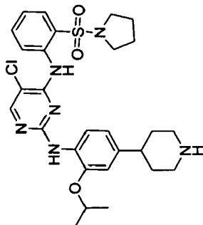
5-chloro-N2-(2-isopropoxy-4-(piperidin-4-yl)phenyl)-N4-(2-(pyrrolidin-1-ylsulfonyl)phenyl)pyrimidine-2,4-diamine
