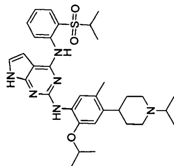
N2-(2-isopropoxy-4-(1-isopropylpiperidin-4-yl)-5-methylphenyl)-N4-(2-(isopropylsulfonyl)phenyl)-7H-pyrrolo[2,3-d]pyrimidine-2,4-diamine
