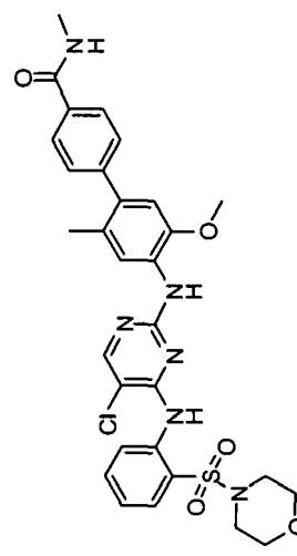
5-chloro-N4-(2-(morpholin-4-yl)sulfonyl)phenyl)-N2-(2-methoxy-5-methyl-4-(4-(methylacetamidophenyl)phenyl)pyrimidin-2,4-diamine
