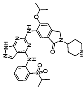
5-isopropoxy-6-(4-(2-(isopropylsulfonyl)phenylamino)-1H-pyrazolo[3,4-d]pyrimidin-6-ylamino)-2-(piperidin-4-yl)isoindolin-1-one
