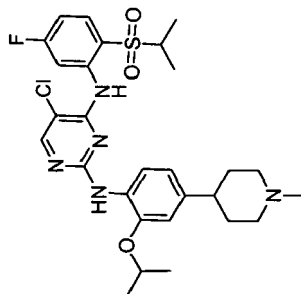
5-chloro-N4-(5-fluoro-2-(isopropylsulfonyl)phenyl)-N2-(2-isopropoxy-4-(1-methyl piperidin-4-yl)phenyl)pyrimidine-2,4-diamine
