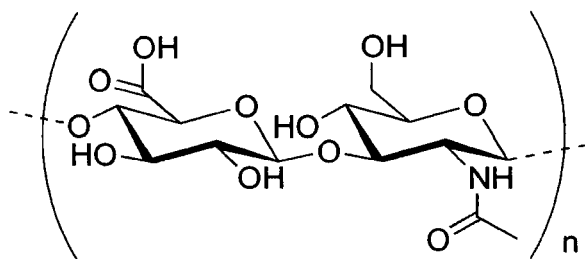
Figure 1. Structure of hyaluron -- D-glucuronic acid and D-N-acetylglucosamine, linked via alternating \beta -1,4 and \beta -1,3 glycosidic bonds.
