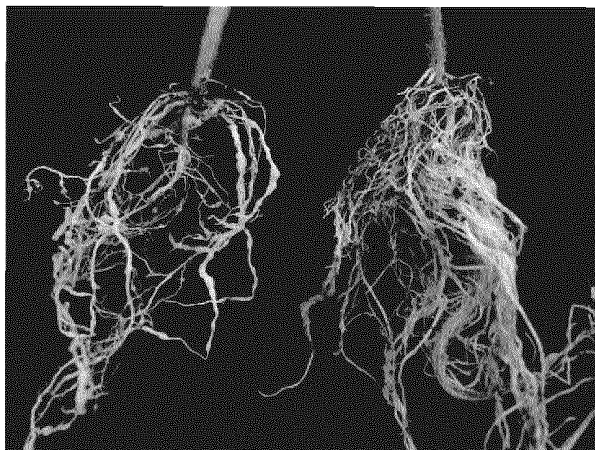
Root gall severity: 4 Root gall severity: 0 (B-barrier) (deposited line)
