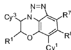
(IIc)
