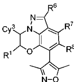
(IIIa)
