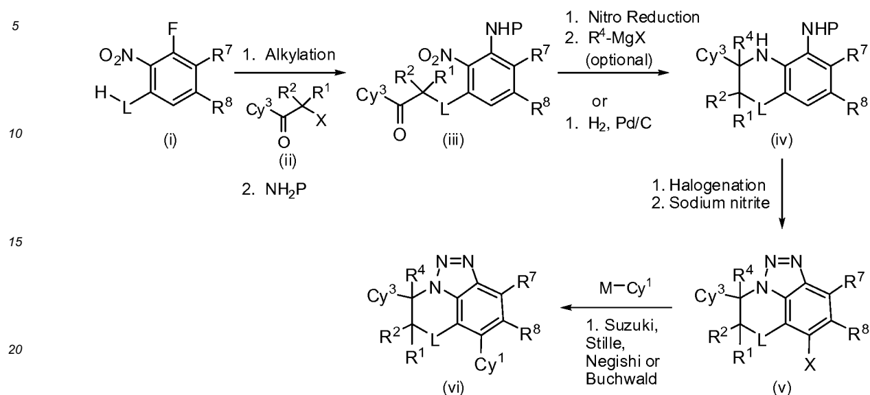
Scheme V
