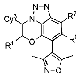
(IIIc)
