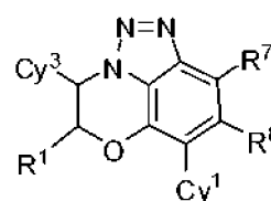
(IIc)
