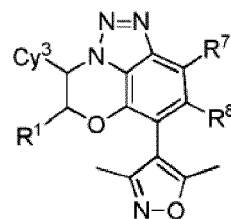
(IIIc)
