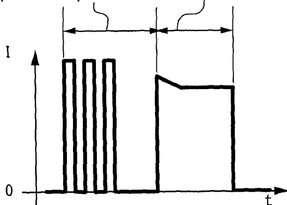
FIG.11D pulsation process continuous current pass process
