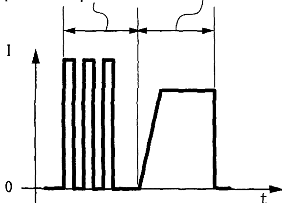
FIG.11A pulsation process continuous current pass process
