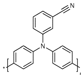
Compound (H)
