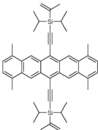
Compound (A)
