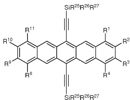
Formula (2)
