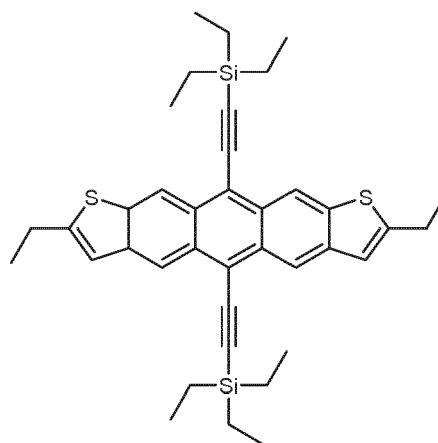
Compound (F)
