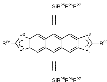
Formula (3)
