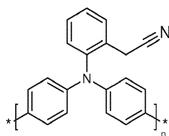
Compound (I)
