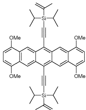
Compound (B)
