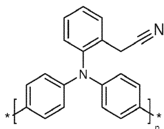
Compound (I)
