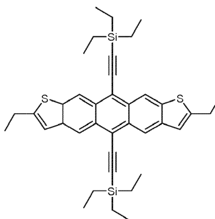
Compound (F)
