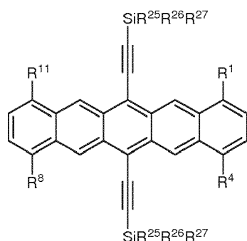
Formula (4)
