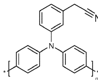
Compound (J)
