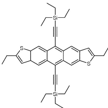
Compound (E)
