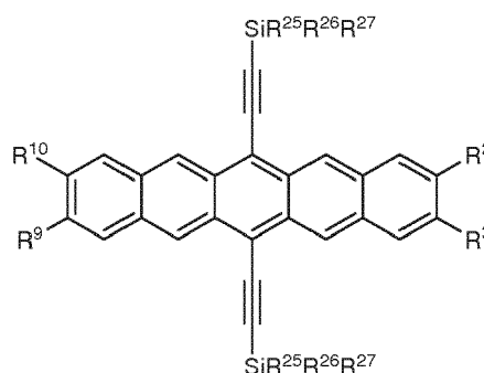
Formula (5)
