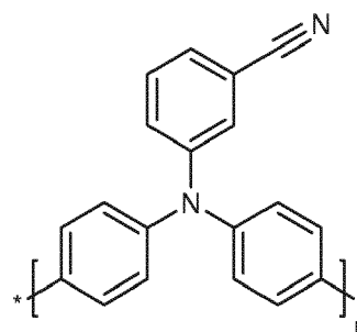
Compound (H)
