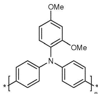
Compound (G)
