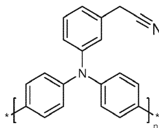
Compound (J)
