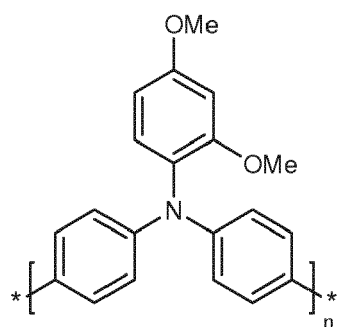
Compound (G)
