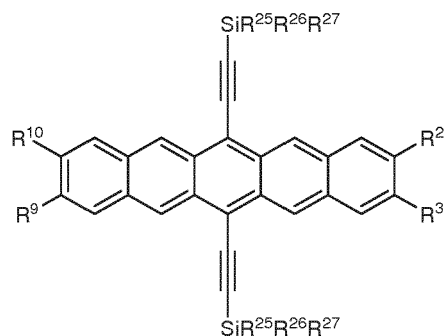
Formula (5)
