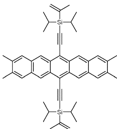
Compound (C)
