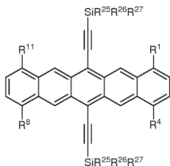
Formula (4)
