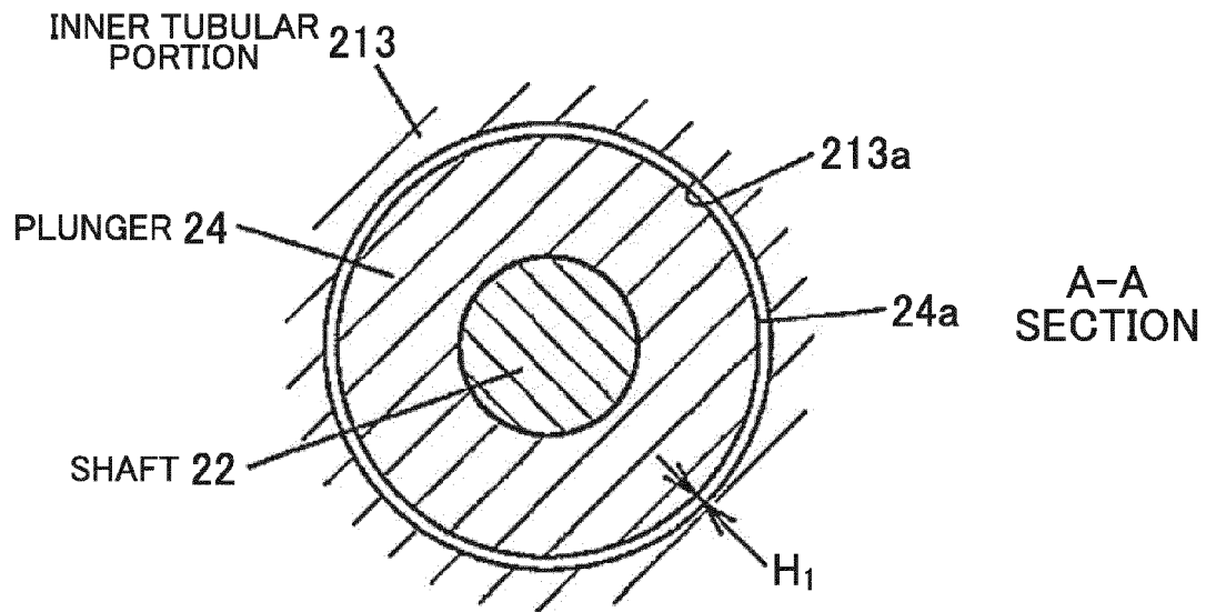
FIG. 3A (FIRST EMBODIMENT)
