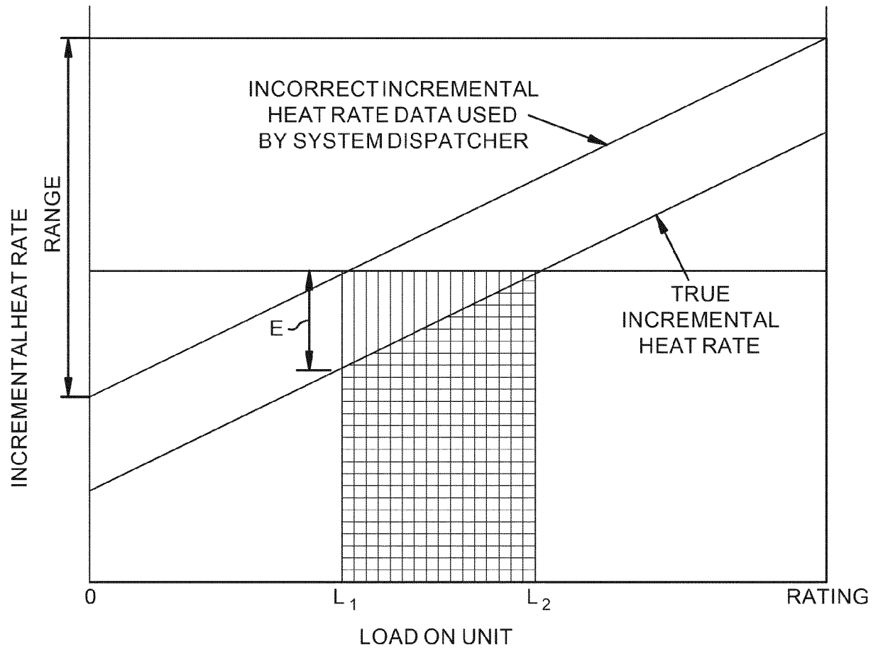
EFFECT OF INCREMENTAL HEAT RATE ERRORS
