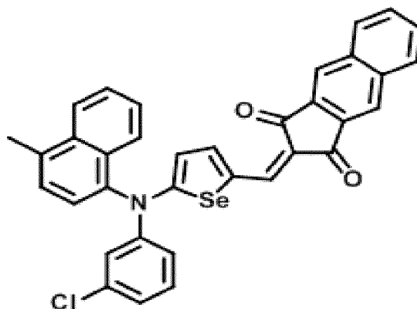
[Chemical Formula 1-7]
