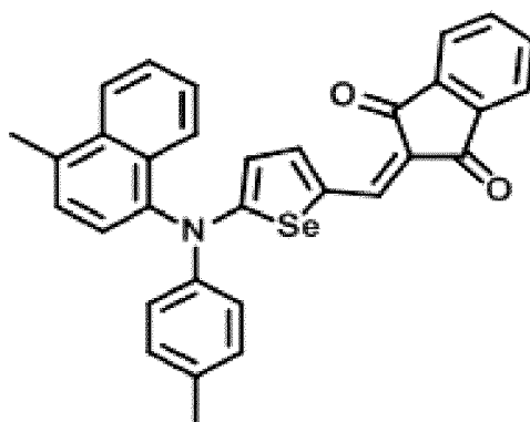
[Chemical Formula 1-2]
