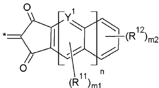
[Chemical Formula 3-1-1]
