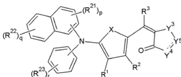
[Chemical Formula 4-3]
