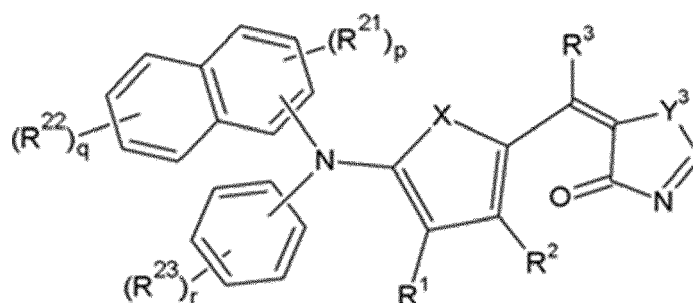
[Chemical Formula 4-3-2]
