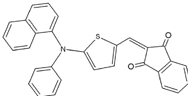
[Chemical Formula 1-17]
