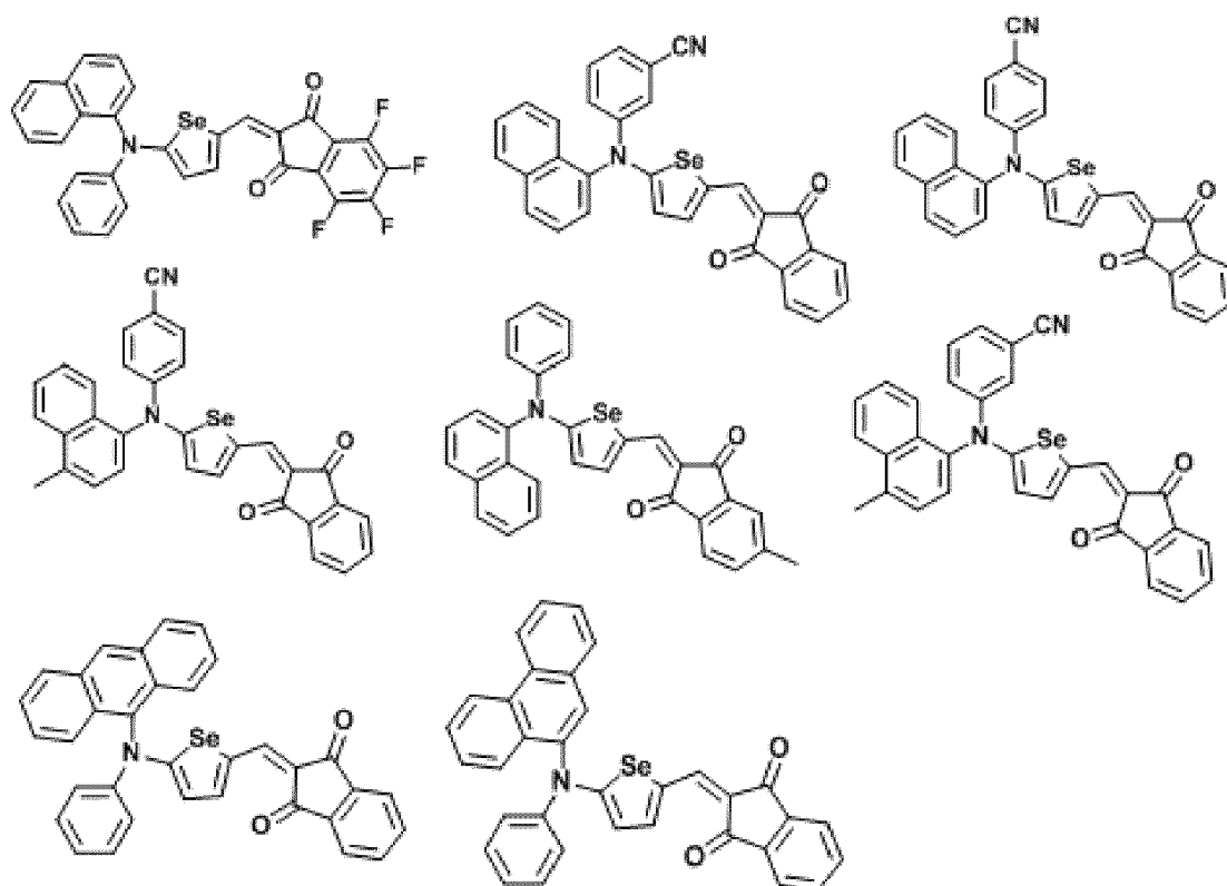
[Chemical Formula 5-2]
