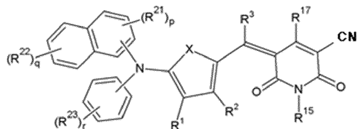
[Chemical Formula 4-2-1]
