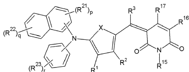
[Chemical Formula 4-2]
