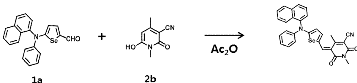
[Reaction Scheme 1-16]
