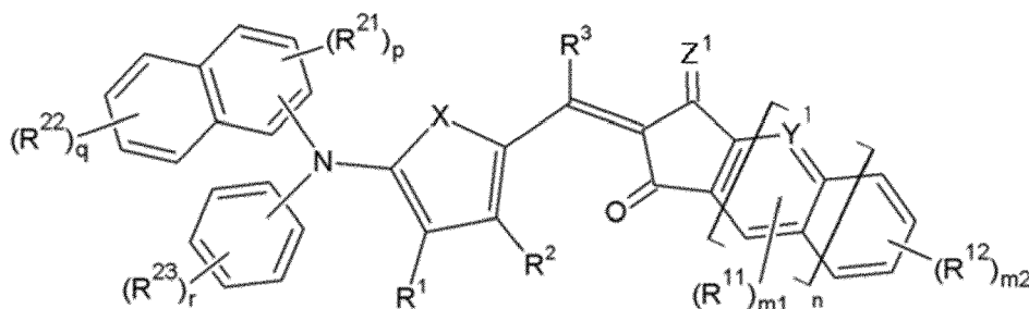
[Chemical Formula 4-2]
