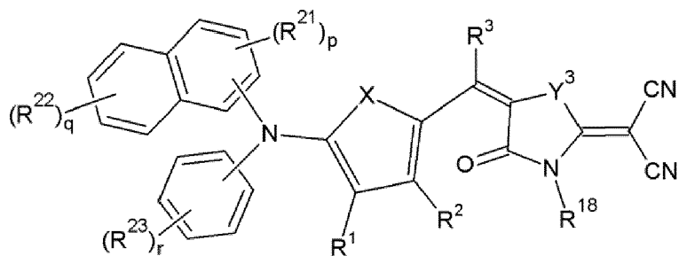
[Chemical Formula 4-3-1]
