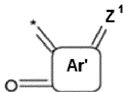
[Chemical Formula 2]
