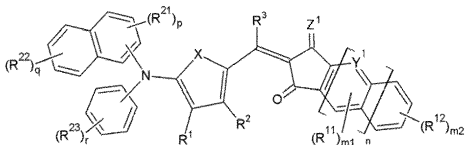
[Chemical Formula 4-2]
