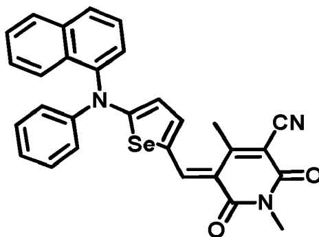
[Chemical Formula 1-16]
