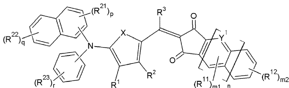
[Chemical Formula 4-1-1]
