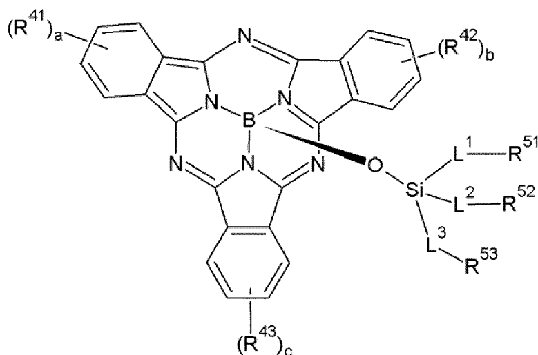
[Chemical Formula 9]
