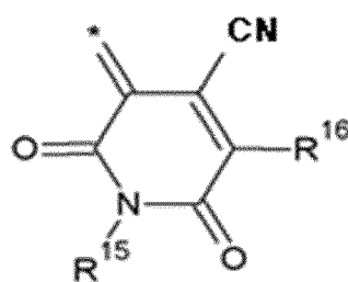
[Chemical Formula 3-2-2]
