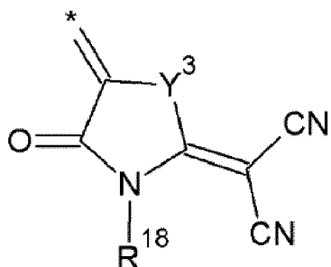
[Chemical Formula 3-3-2]
