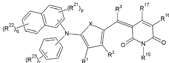
[Chemical Formula 4-2]
