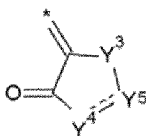
[Chemical Formula 3-3]
