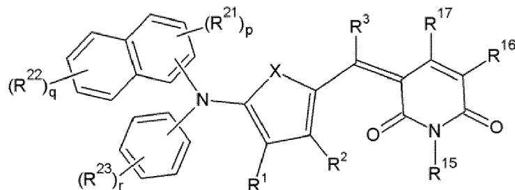
[Chemical Formula 4-3]
