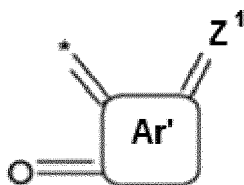
[Chemical Formula 2]
