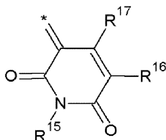
[Chemical Formula 3-2]
