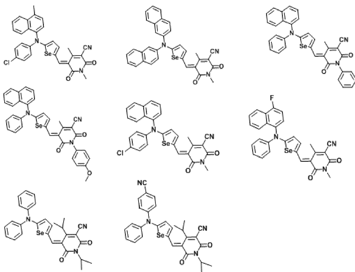
[Chemical Formula 5-4]
