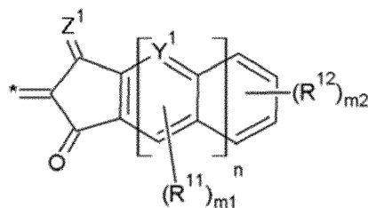
[Chemical Formula 3-1]
