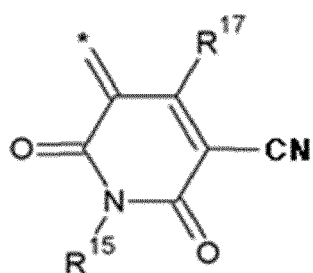
[Chemical Formula 3-2-1]
