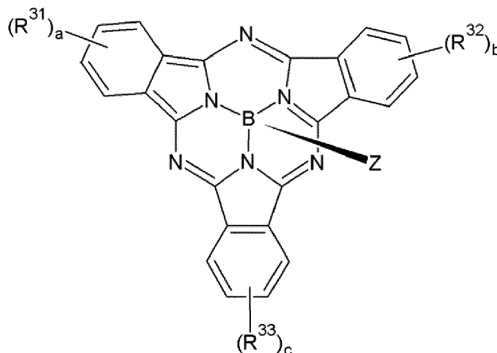
[Chemical Formula 6]
