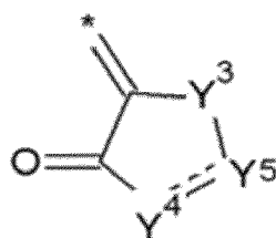
[Chemical Formula 3-3]
