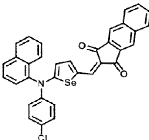
[Chemical Formula 1-8]
