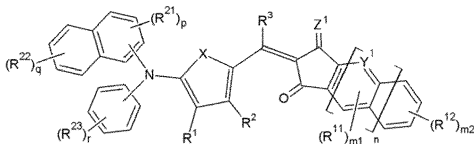
[Chemical Formula 4-1]
