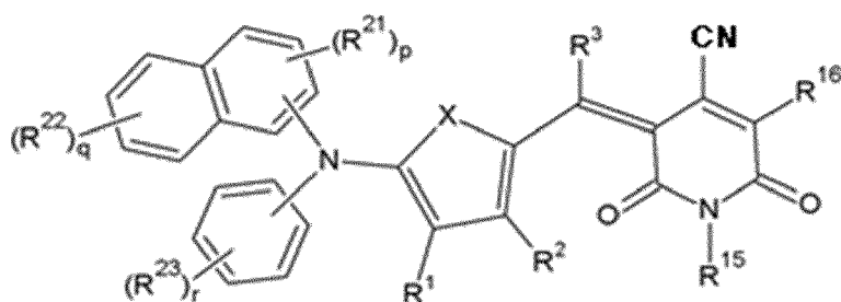
[Chemical Formula 4-2-2]
