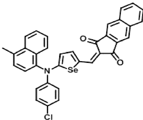
[Chemical Formula 1-9]
