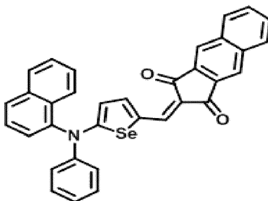
[Chemical Formula 1-3]
