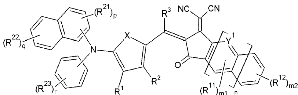
[Chemical Formula 4-1-2]
