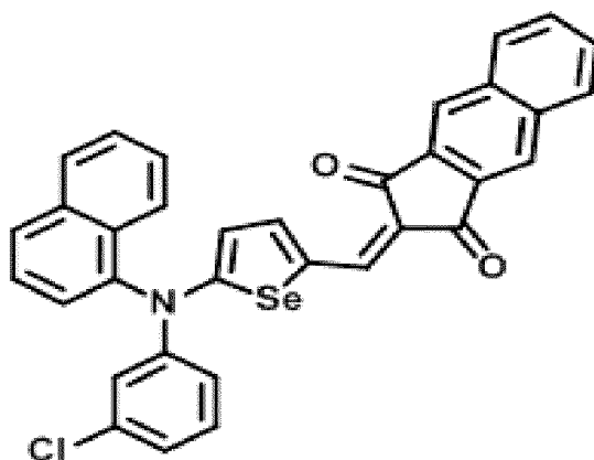
[Chemical Formula 1-6]
