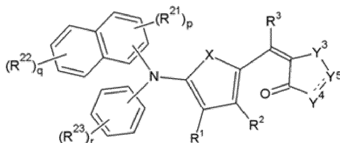
[Chemical Formula 4-3]
