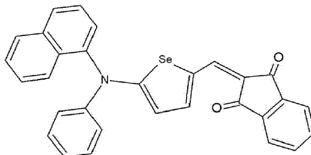
[Reaction Scheme 1]
