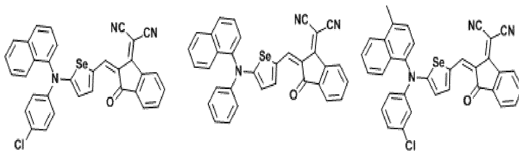
[Chemical Formula 5-4]
