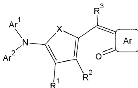
[Chemical Formula 1]
