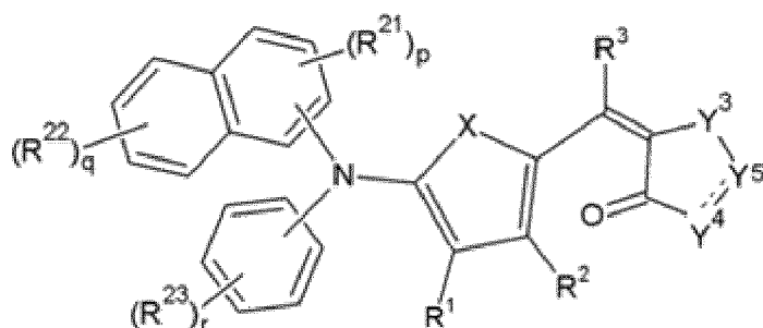
[Chemical Formula 4-3]
