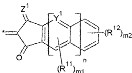
[Chemical Formula 3-1]
