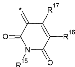
[Chemical Formula 3-2]
