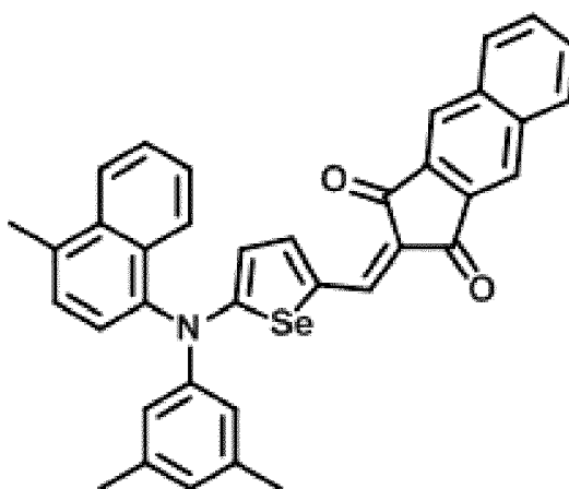
[Chemical Formula 1-5]
