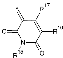
[Chemical Formula 3-3]
