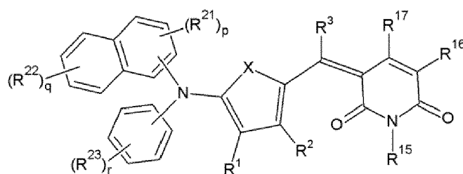
[Chemical Formula 4-2]
