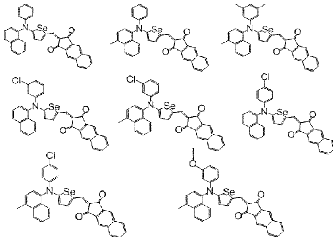
[Chemical Formula 5-2]
