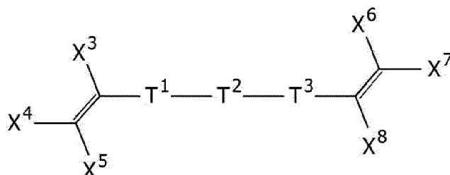
[Chemical Formula 8]
